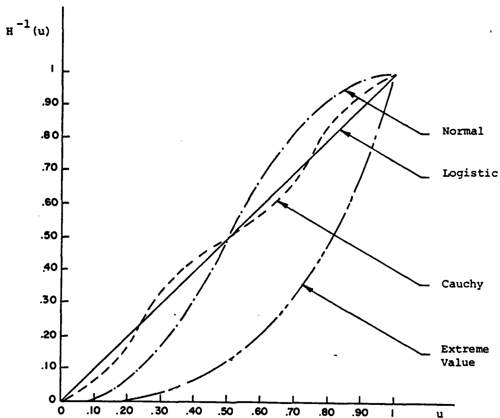
Figure 1. The H^{-1} functions for various distributions in the case that \sigma is known.
