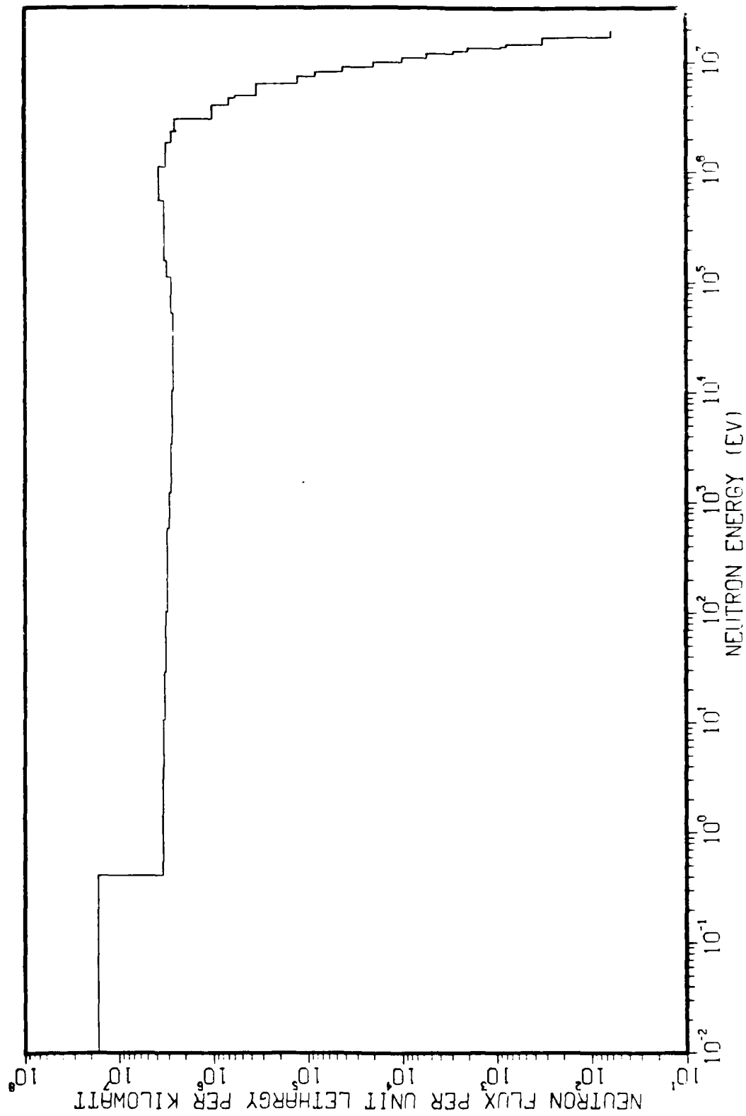
Figure II.3.21. Back (1-D) Neutron Flux vs Energy ERI With 2" PB and Exercise Wheel.
