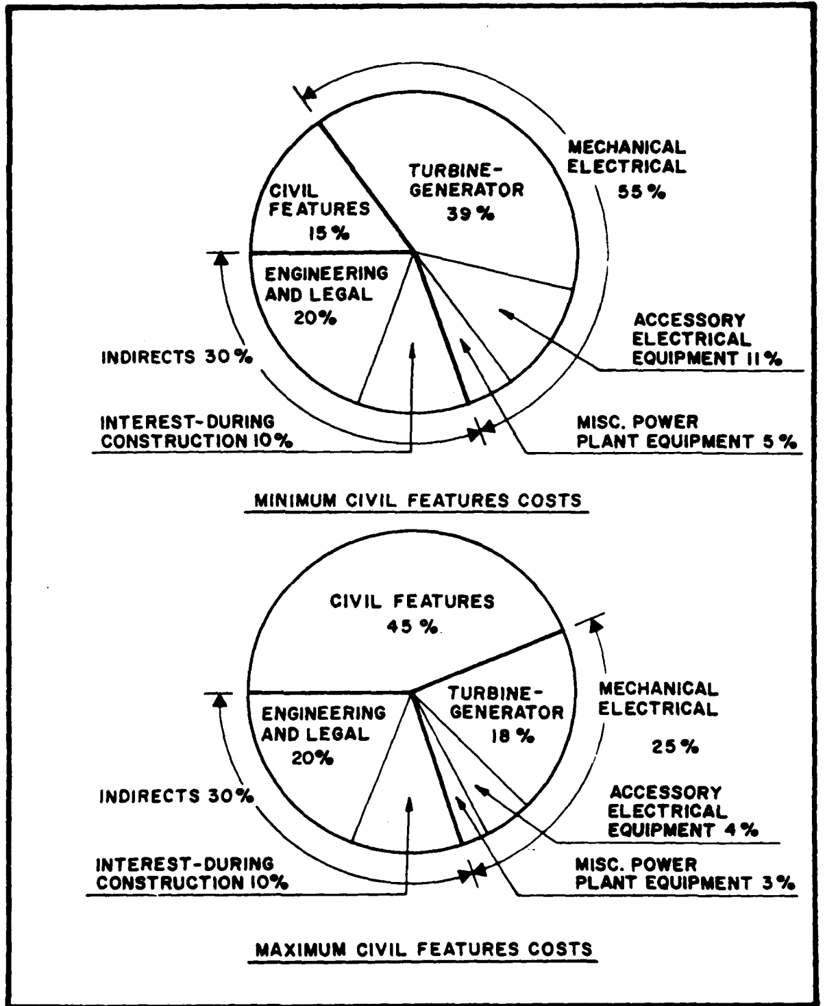
Figure 1. Range of Civil Features Costs (Vol. 6 HEC, 1979)
