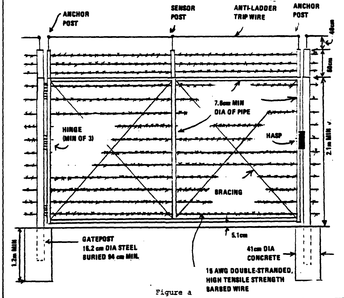
Figure 14 Taut Wire Fence Gate
