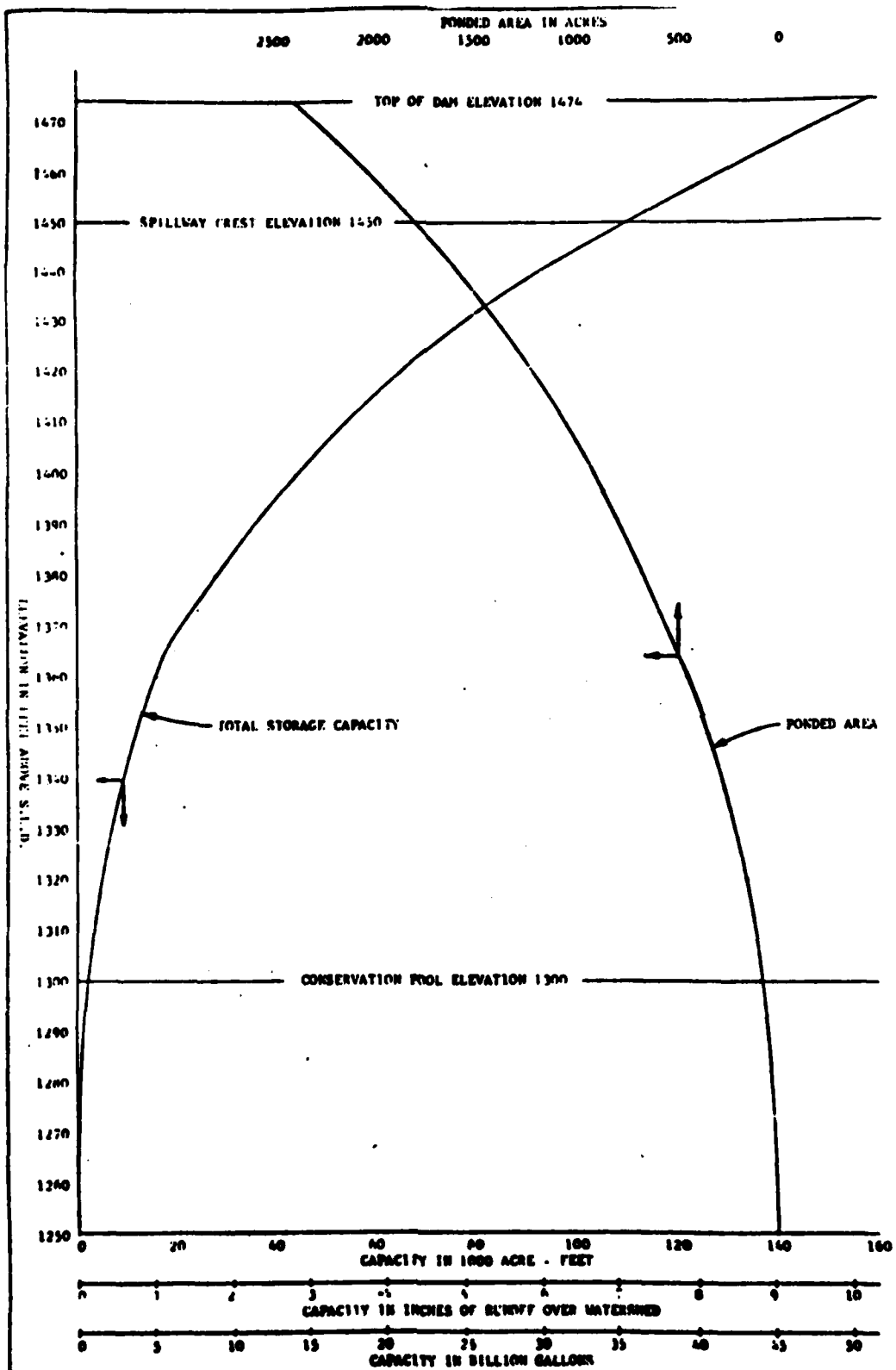
LEHIGH RIVER, PA. FRANCIS S. WALTER RESERVOIR ELEVATION VS. TOTAL CAPACITY AREA & CAPACITY
