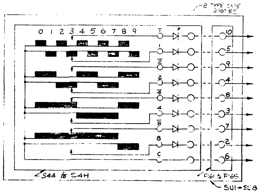
FIG. 24(b) PRESET STOP SWITCH UNIT
