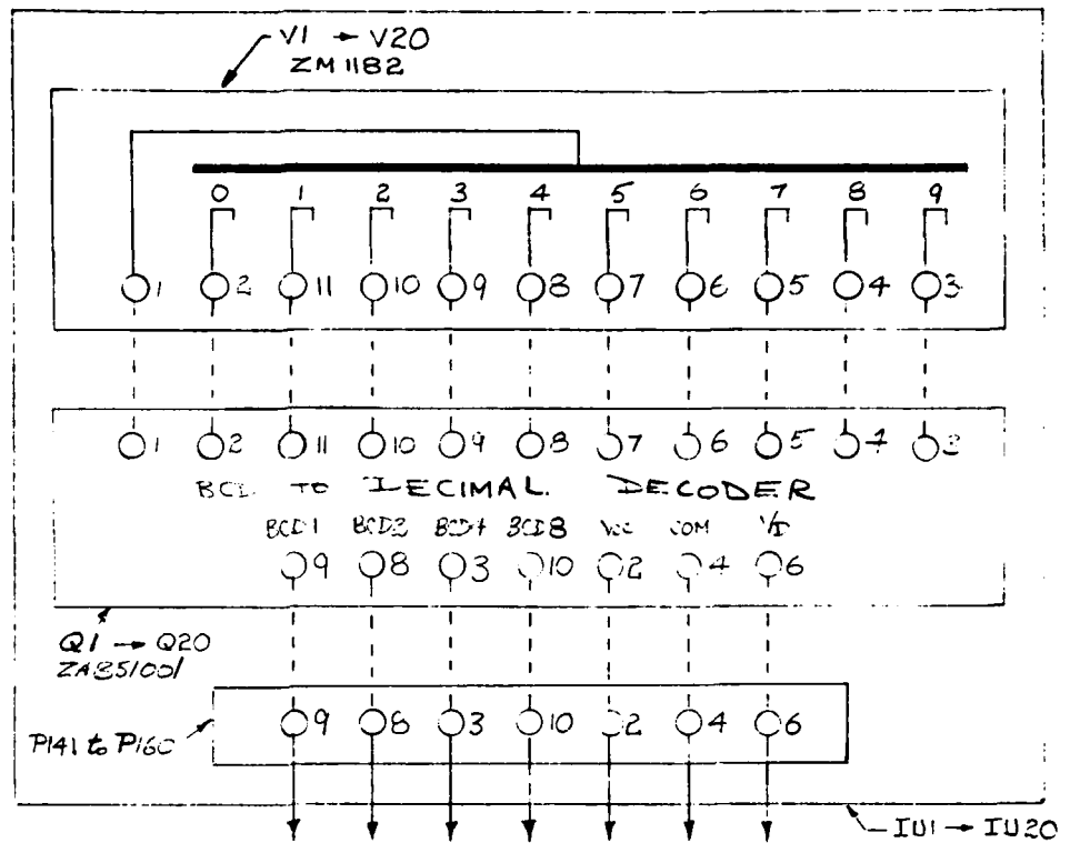
FIG. 24(a) NUMERIC INDICATOR UNIT
