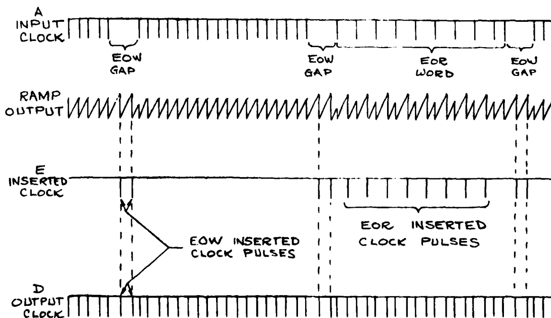
FIG. 11(b) ELECTRONIC FLYWHEEL WAVEFORMS FOR SERIAL SYSTEM EMPLOYING FRAME SYNCHRONIZATION TYPE B
