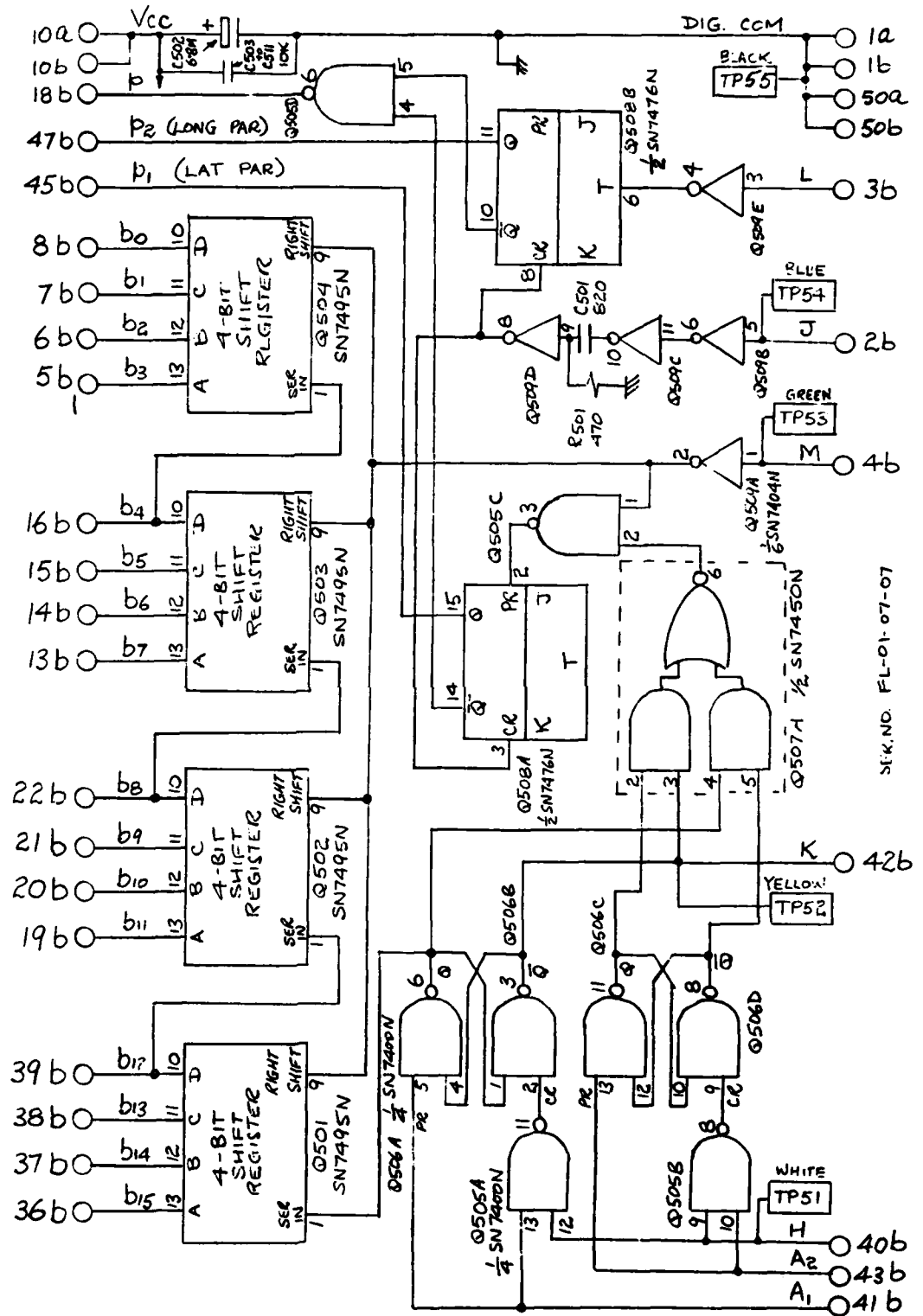
FIG. 19 SERIAL TO PARALLEL CONVERTER FOR SERIAL SYSTEM
