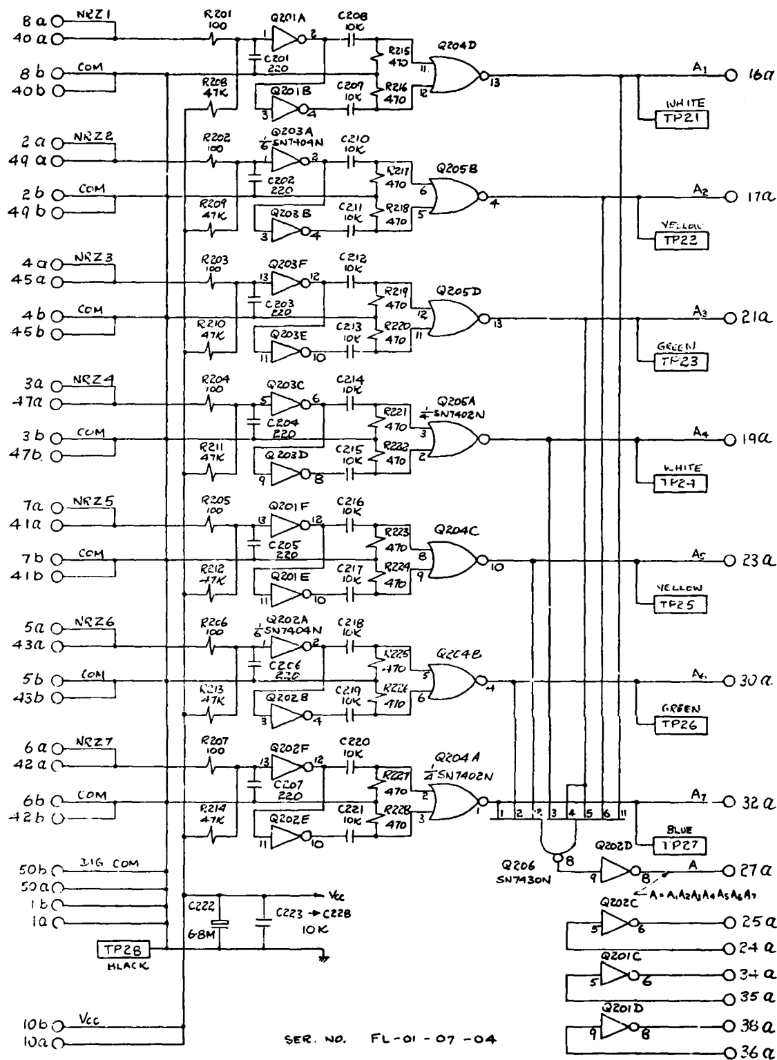
FIG. 8 INPUT CLOCK SIGNAL GENERATOR
