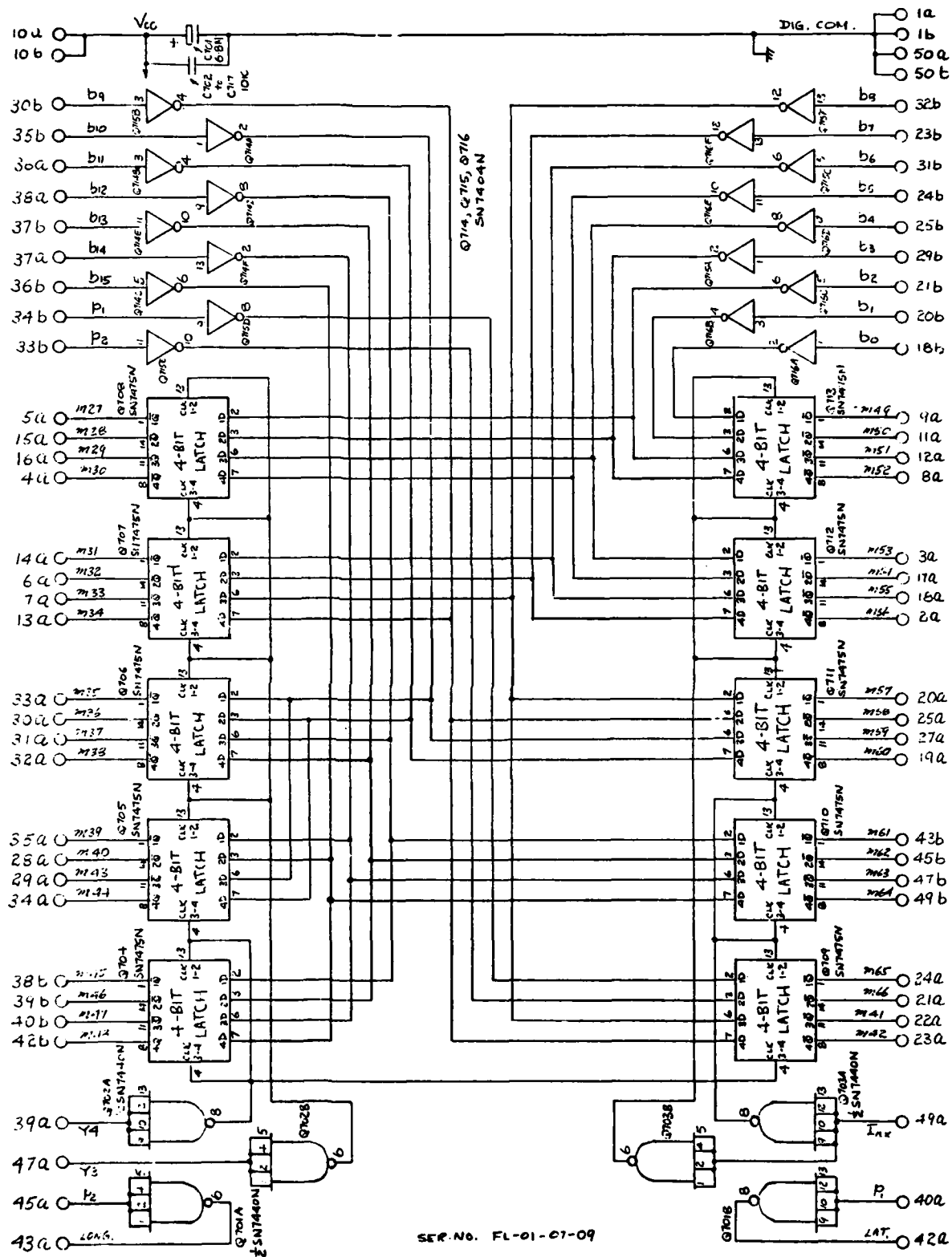
FIG. 23 SELECTED DATA AND FIXED DATA STORE
