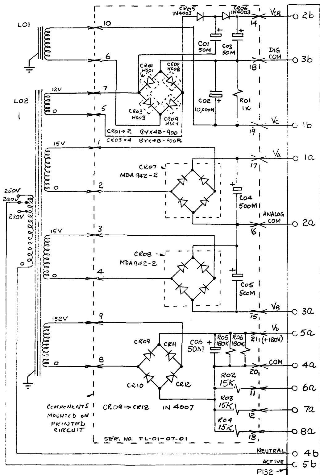
FIG. 5 AC TO DC CONVERTER
