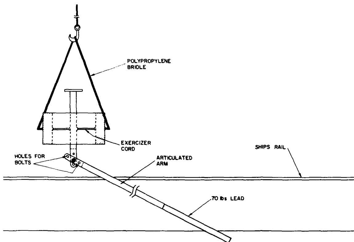
Fig. 6 — Deployment of assembled float and mast
