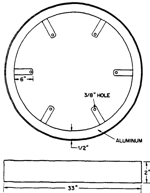
Fig. 2 - Retainer ring
