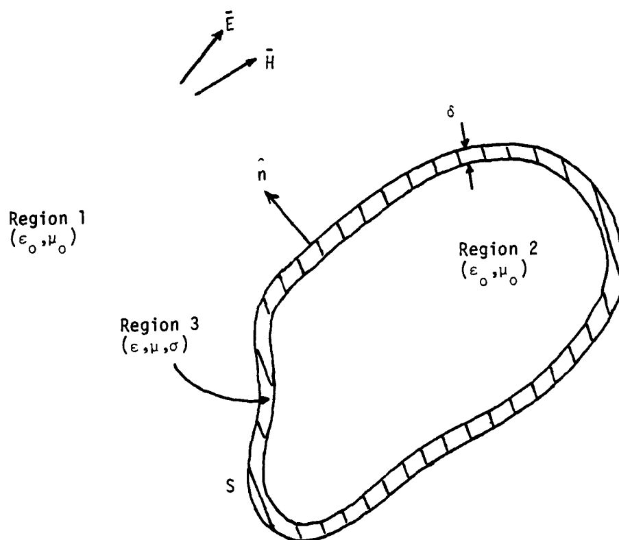
Fig. 1.3 Diagram for the Derivation of the Resistive Boundary Condition.
