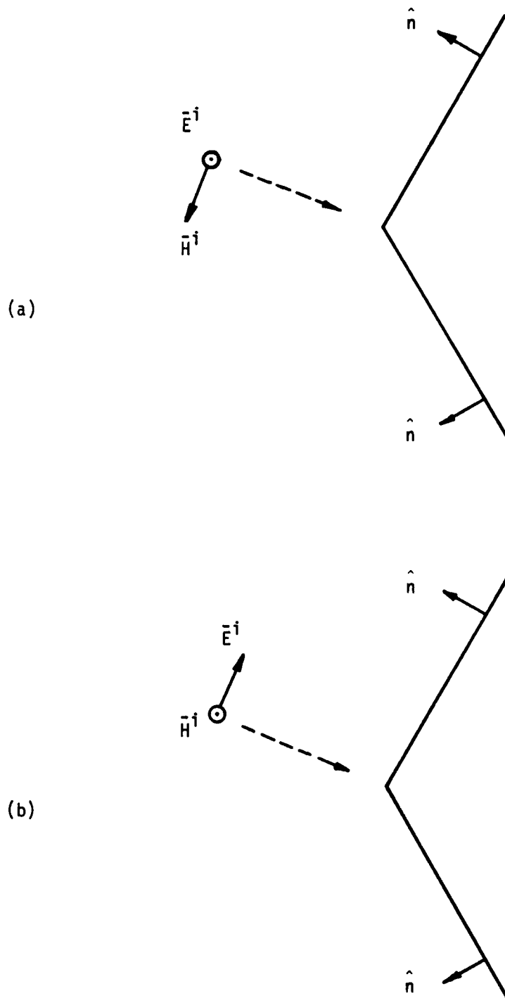
Fig. 1.5 Two-Dimensional Excitation of a Wedge by an (a) E-Polarized and (b) H-Polarized Plane Wave.
