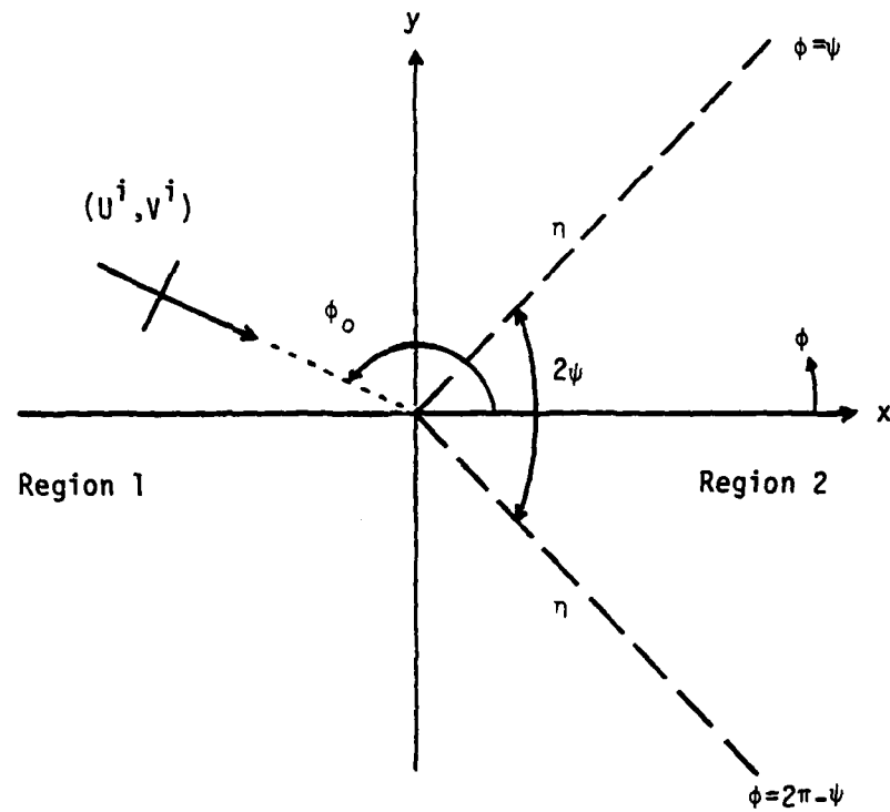
Fig. 4.1: Geometry for the Application of the Kontorovich-Lebedev Transform to the Scattering by a Resistive Wedge.
