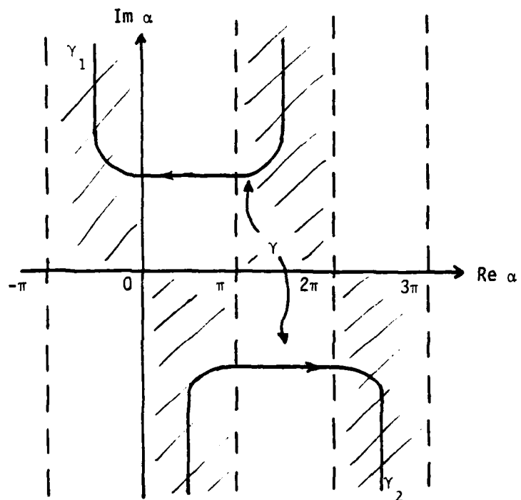
Fig. 3.1: The Contour of Integration \gamma in the Complex \alpha -Plane for Use with the Maliuzhinets Method.
