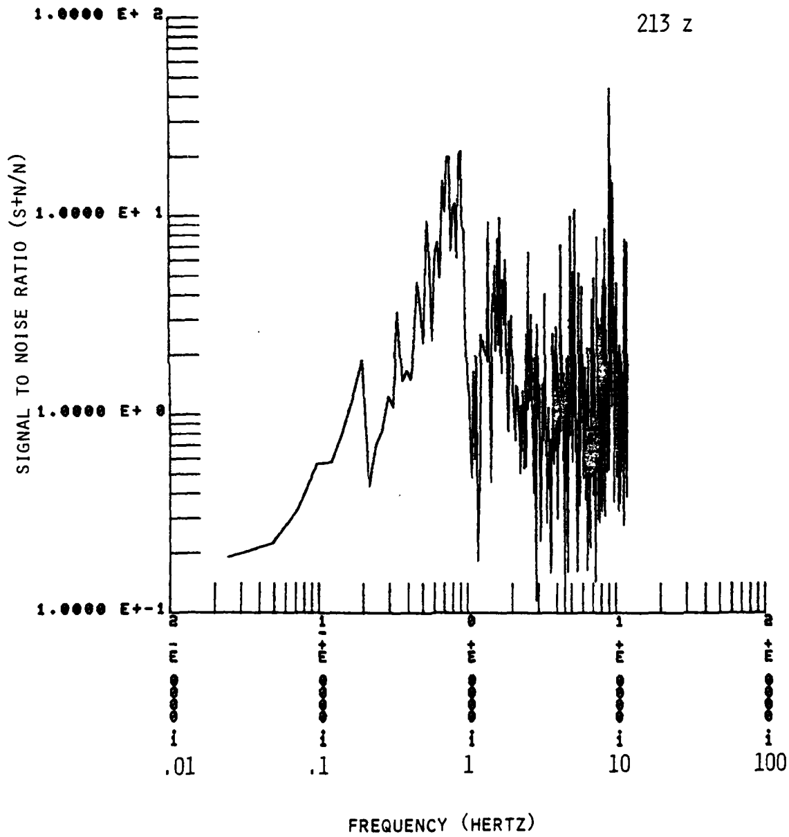
Figure 2-14 HARZER P wave signal to noise ratio.
