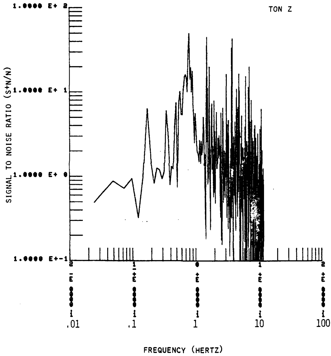
Figure2-15.HARZER P wave signal to noise ratio. TON Z
