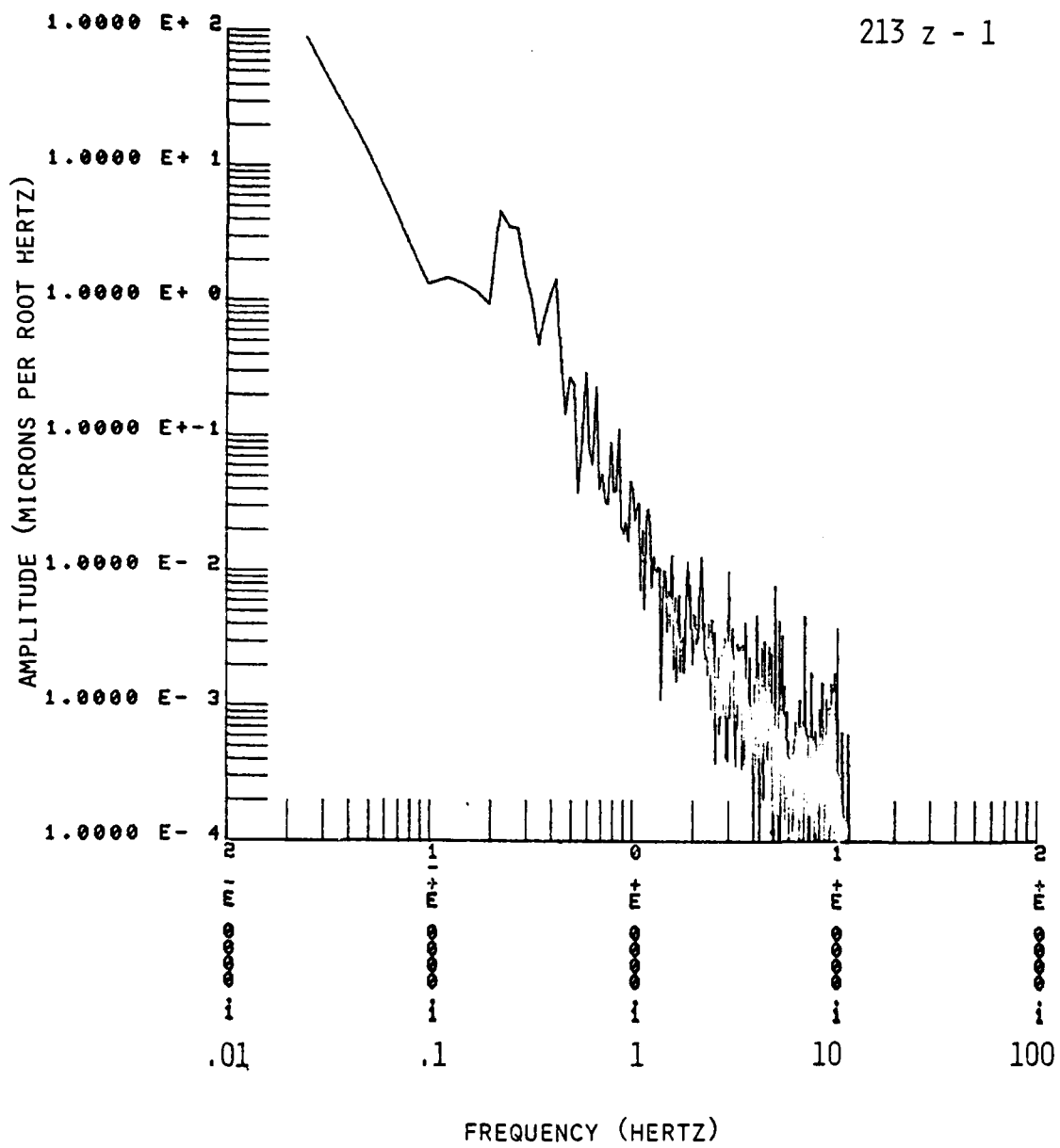
Figure 3-31.HARZER noise spectrum. 213 Z
