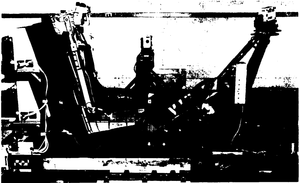
Figure 26. Test Fixture Mounted on the Impact Carriage for the X Axis Tests.
