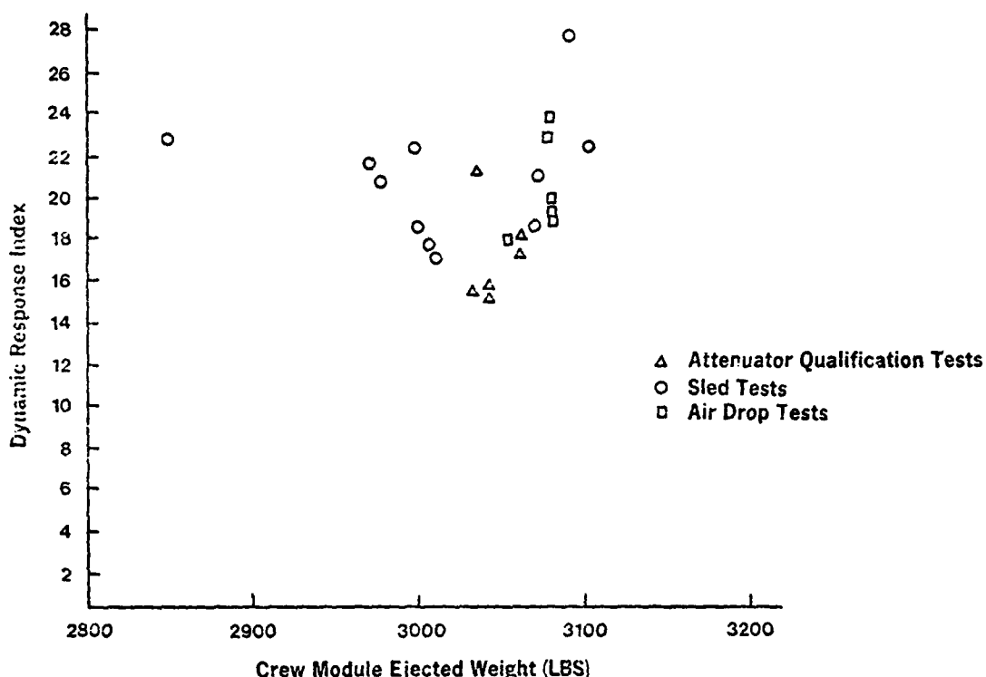
Figure 6. Dynamic Response Index Values Calculated From Ground Landing Impact Test Data (Gossick et al. , 1968).
