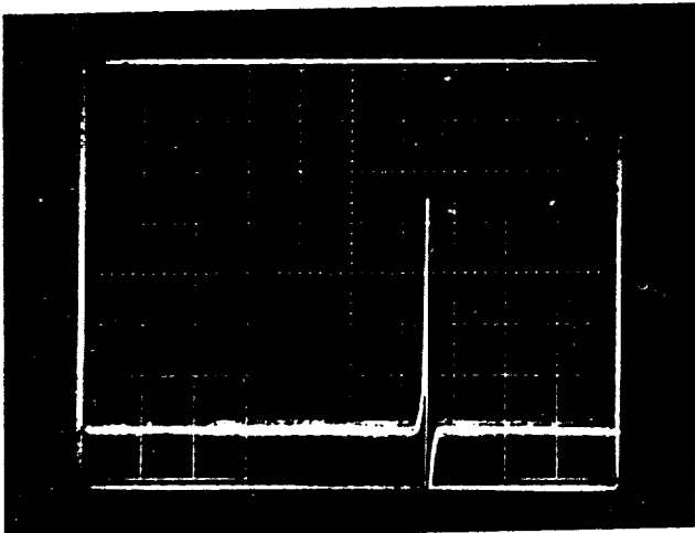
Figure 2.6 Pressure-time Records for NACO Propellant with BKNO 3 , BP, and NC Igniters
