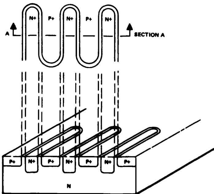
Figure 14. Origin of Simulated Interdigitated Structure
