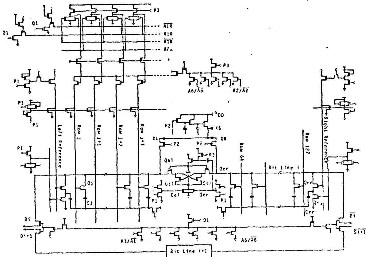
Fig. 4 Bit-Line Circuitry a la MX-4116
