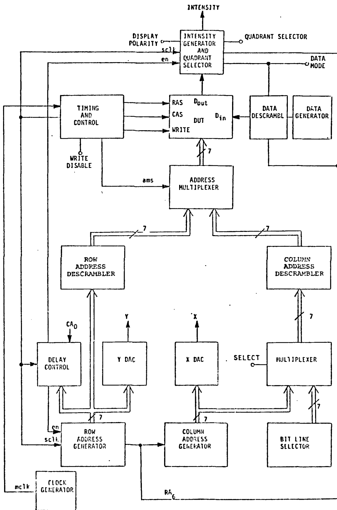
Fig. 11: Raster-Scan Memory-Exerciser
