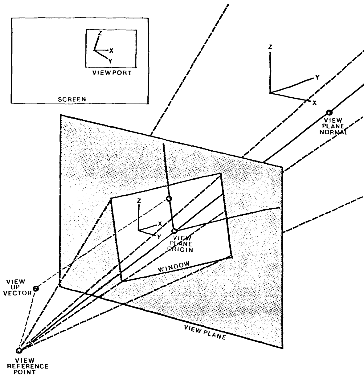
Figure C-15 General Viewing Scheme
