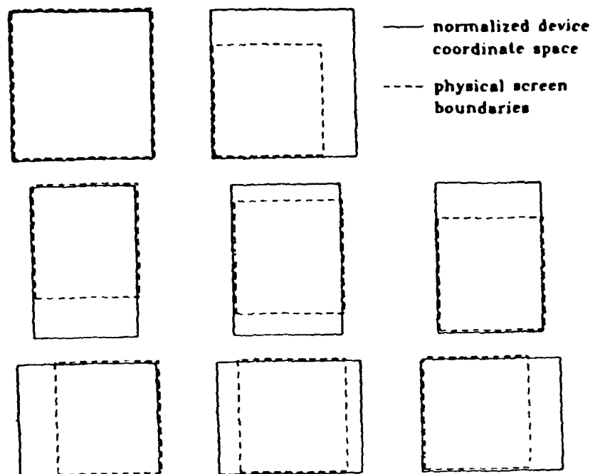
Figure C-17 Possible mappings of Normalized Device Coordinate space to physical screen coordinates
