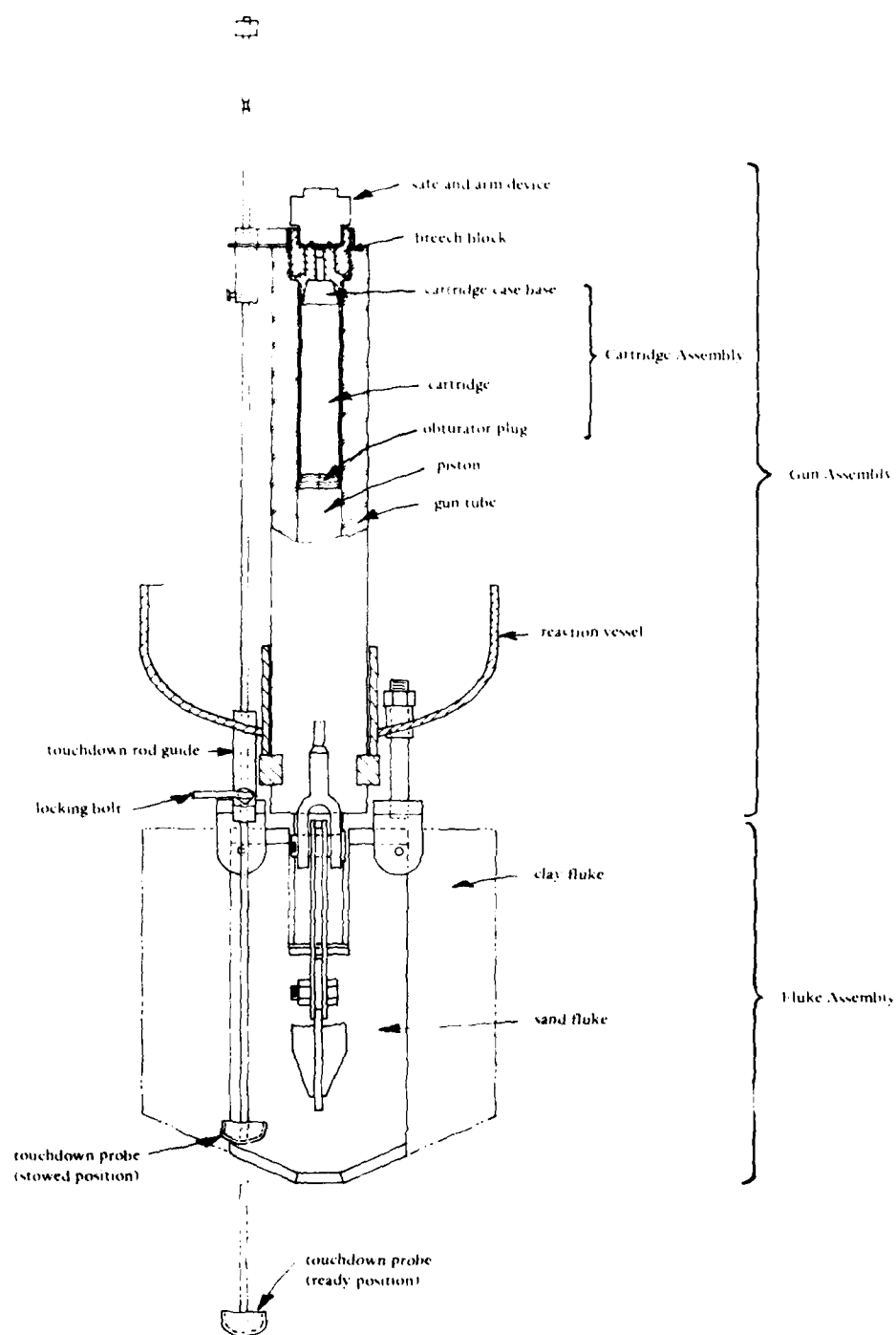
Figure 2. Schematic of the NCEL 10K propellant-embedded anchor.
