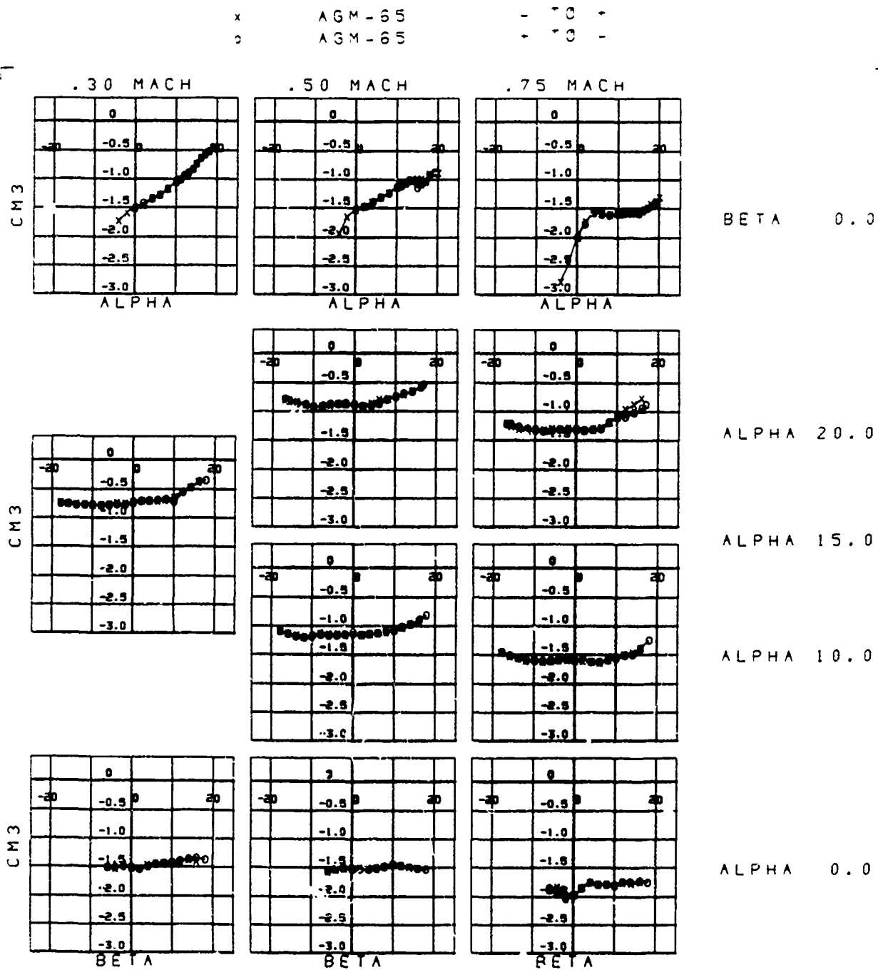
Figure 14. Hysteresis Data, CM, Pylon 3, Configuration 30
