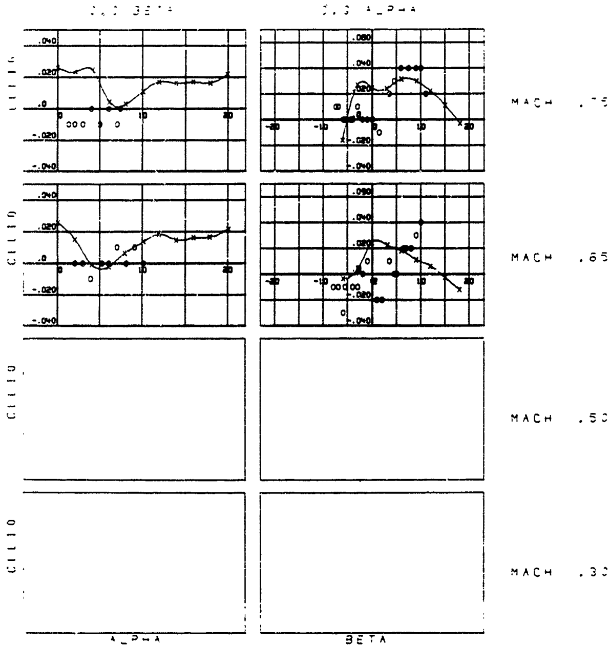
Figure 147. Wind Tunnel Versus 100% Loads Flight Test, Pylon 10, SUU-30, CL1
