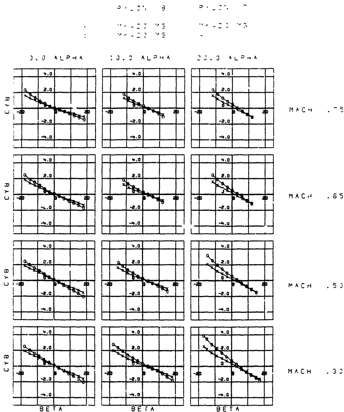
Figure 84. CY, Pylon 3 Versus Pylon 7, Cases 51, 54
