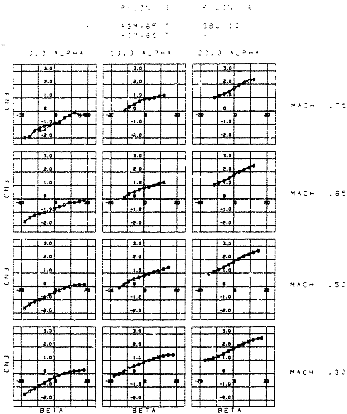
Figure 77. CN, Pylon 3 Versus Pylon 4, Cases 21, 34
