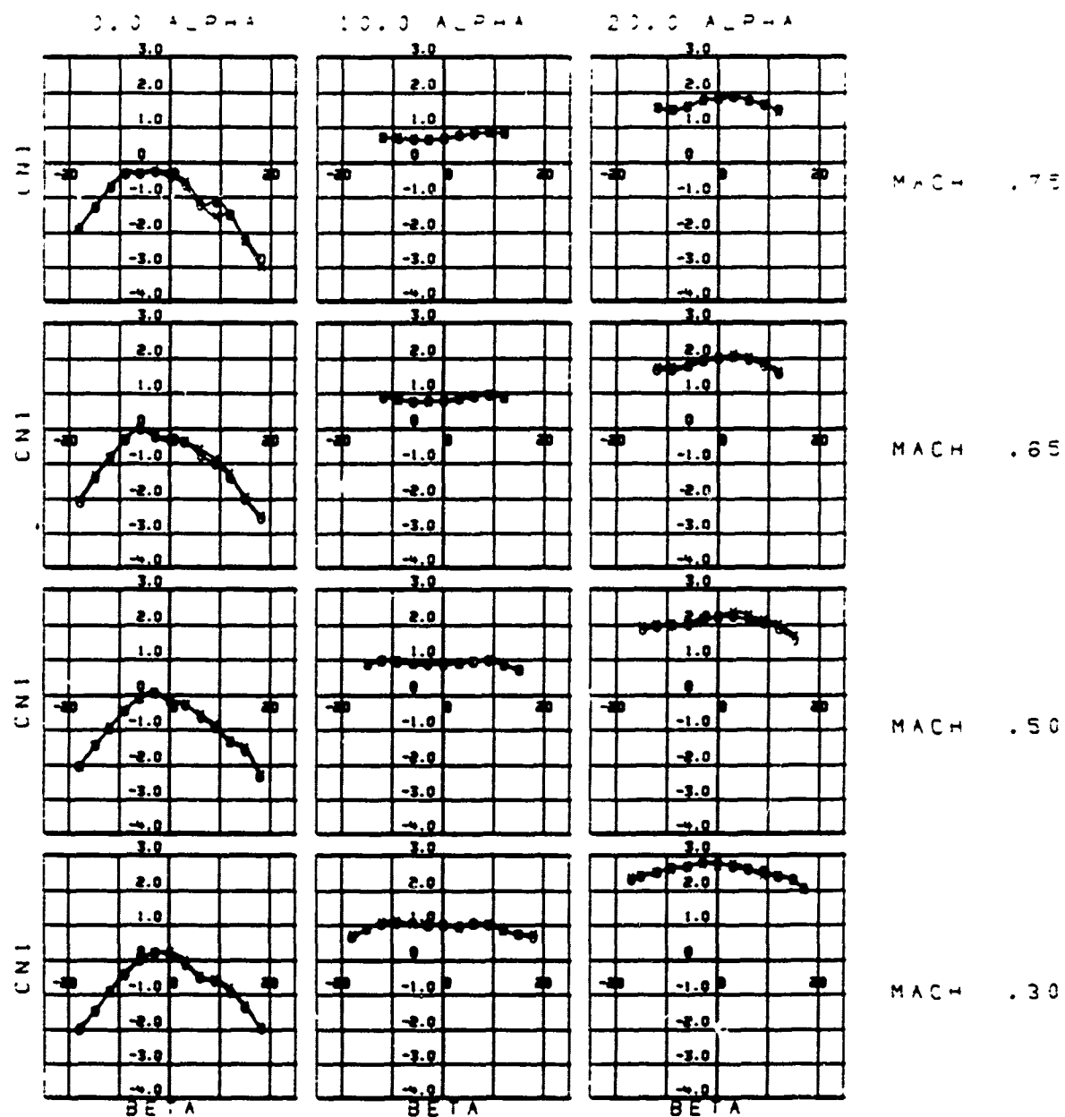
Figure 41. CN, Pylon 1 Versus Pylon 3, Cases 4, 12
