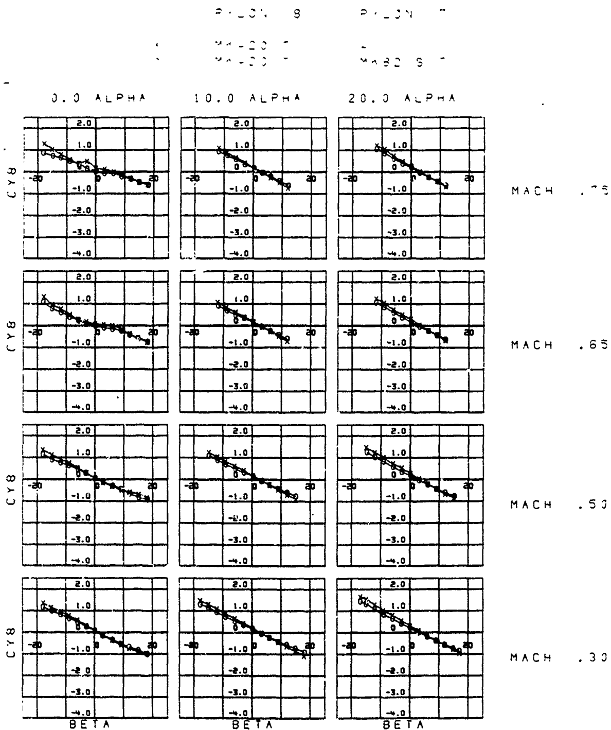
Figure 86. CY, Pylon 8 Versus Pylon 7, Cases 50, 55
