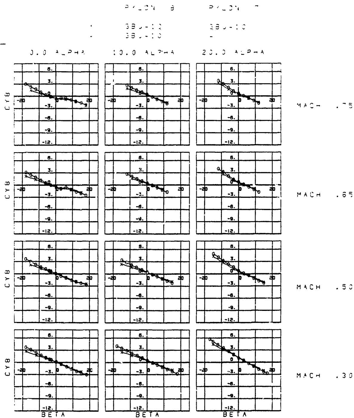
Figure 88. CY, Pylon 8 Versus Pylon 7, Cases 49, 56
