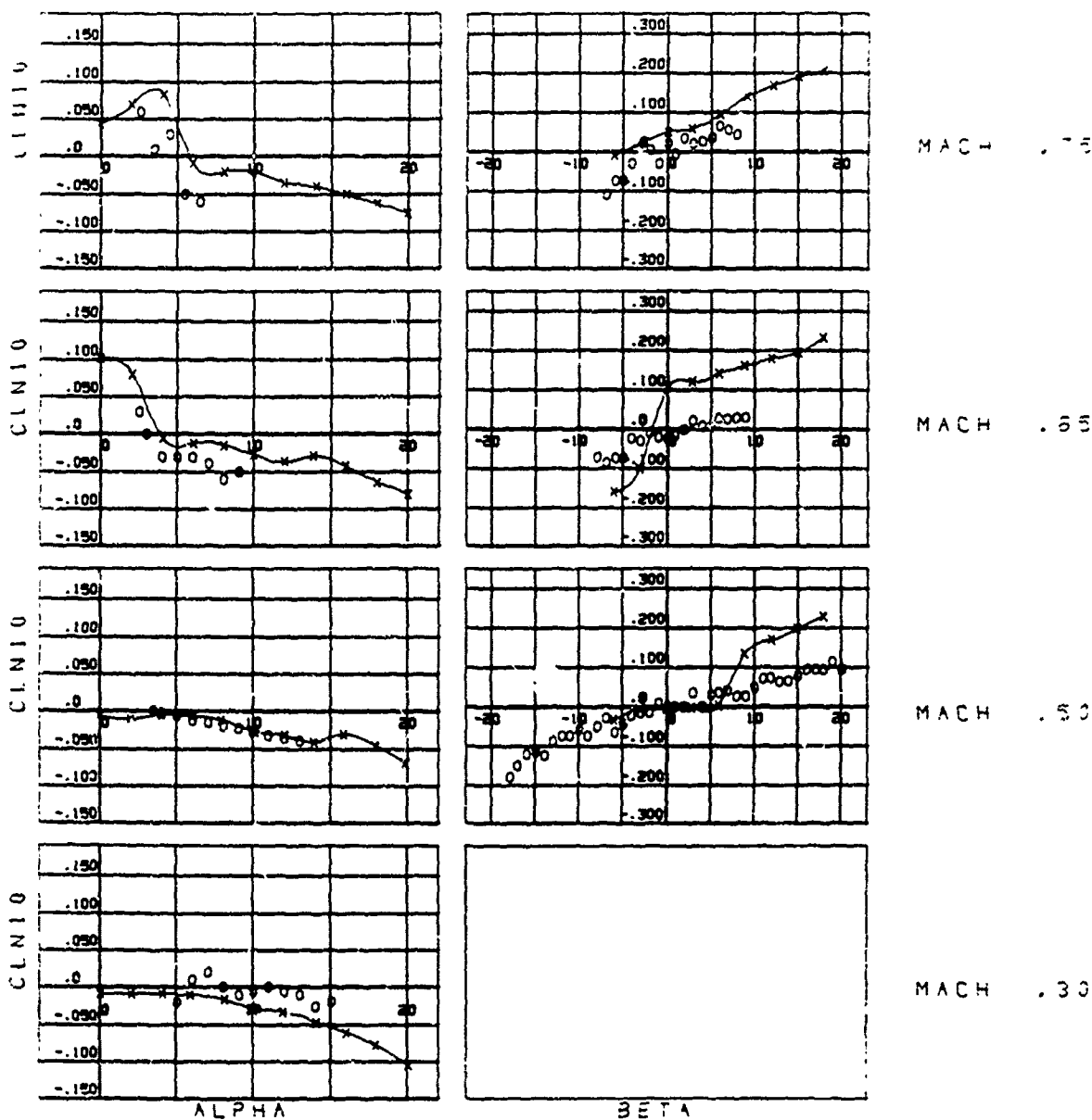
Figure 141. Wind Tunnel Versus 80% Loads Flight Test, Pylon 10, SUU-30, CLN
