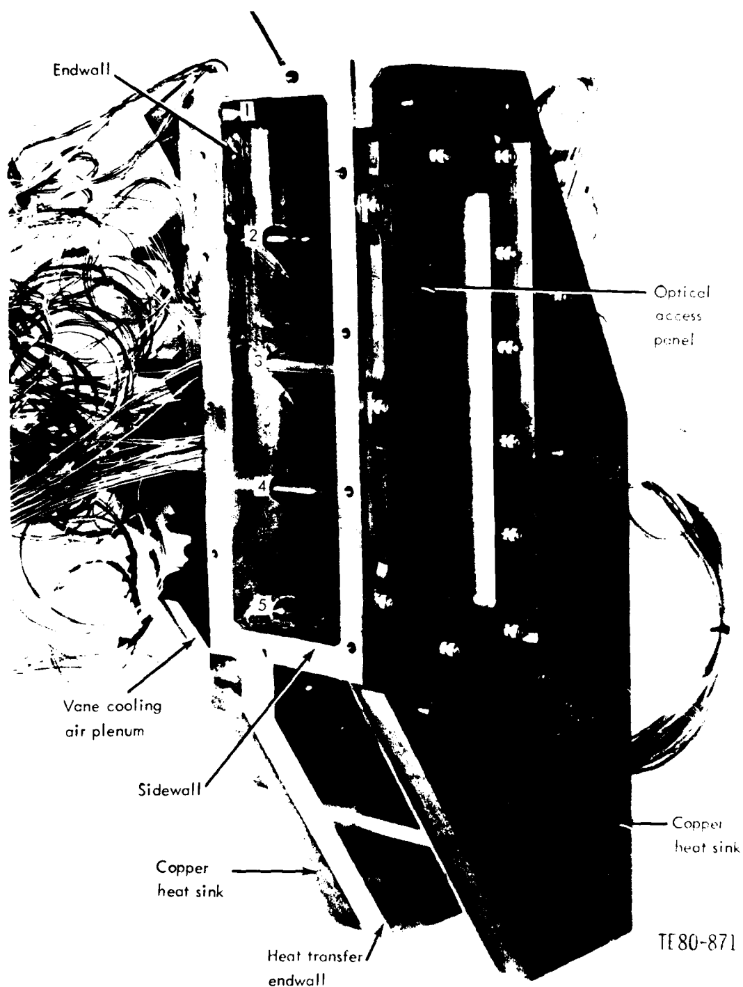
Figure 10. Cascade assembly.
