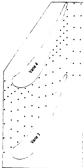
Figure 20. Relative thermocouple locations for adiabatic endwall.
