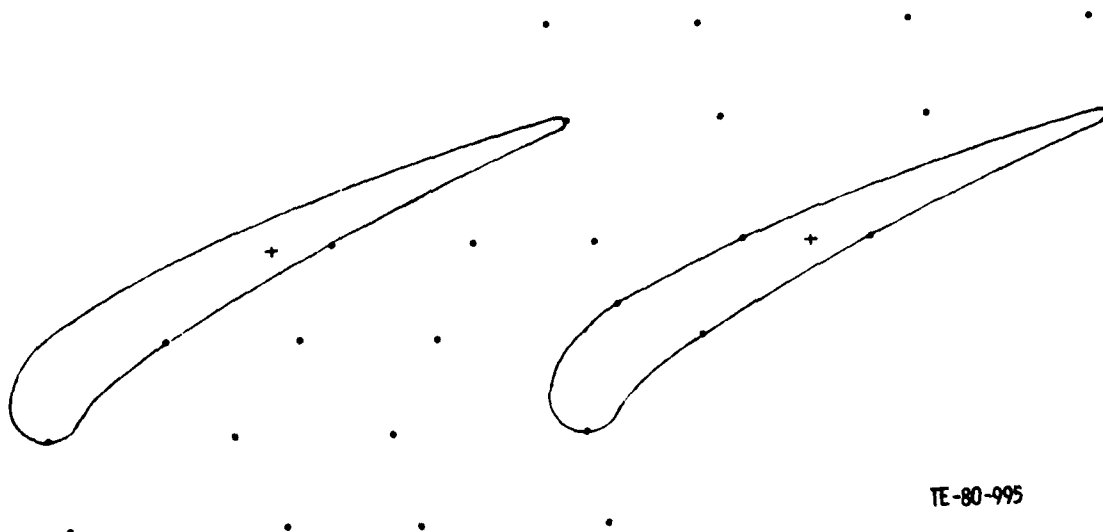
Figure 35. Relative thermocouple locations for cooled side of tip endwall.
