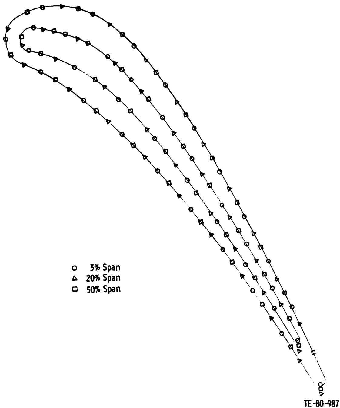
Figure 25. Relative location of exterior and interior thermocouples.
