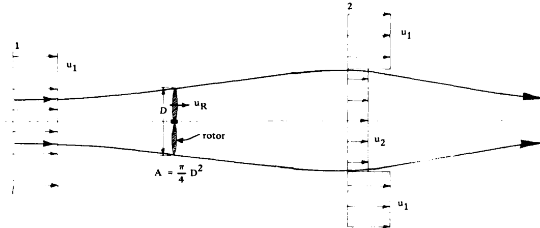
Figure 4.1. Flow configuration through a wind turbine rotor.
