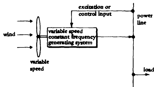
Figure 4.31. The schematic of a field-modulated alternator.
