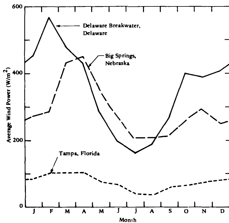
Figure 2.25. Average monthly wind power available at three sites.
