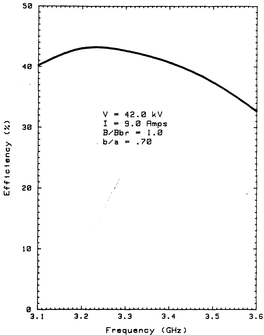
FIGURE 4.24 PREDICTED CONVERSION EFFICIENCY OF S-BAND TWT WITH BRILLOUIN BEAM
