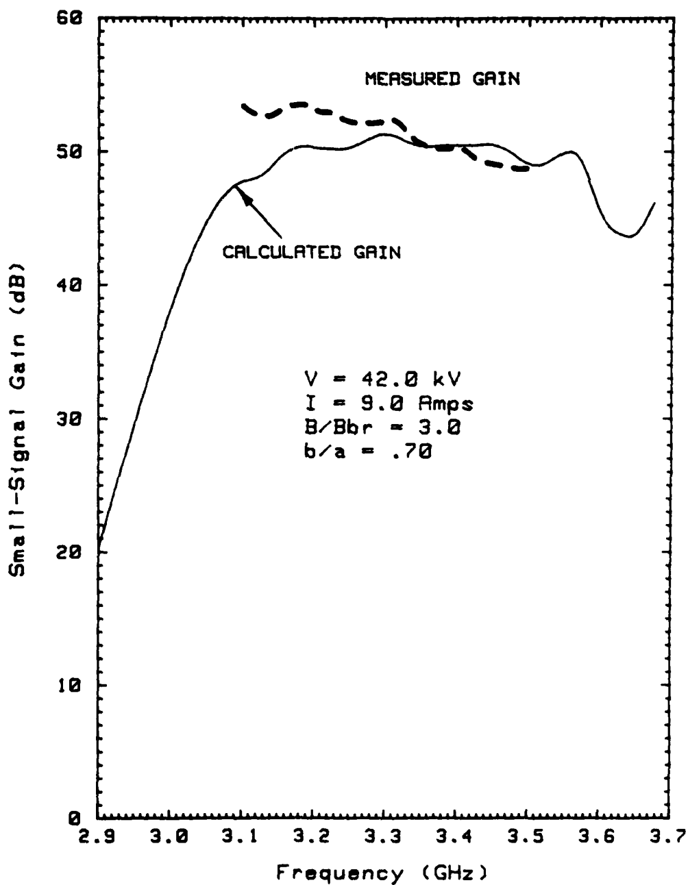
FIGURE 4.20 COMPARISON OF PREDICTED AND MEASURED SMALL SIGNAL GAIN FOR HIGH EFFICIENCY TWT
