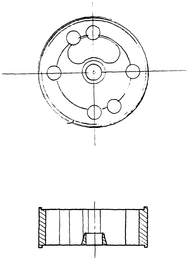
FIGURE 3.5 SKETCH SHOWING TYPE I CAVITY SPACER AND PLATE WITH LOSSY CERAMIC CYLINDERS IN CAVITY WALL
