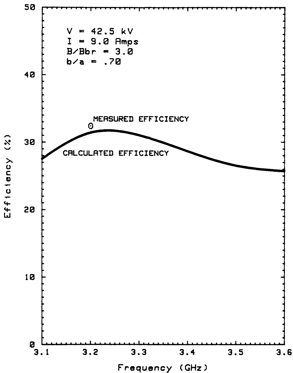
FIGURE 4.23 COMPARISON OF PREDICTED AND MEASURED CONVERSION EFFICIENCY FOR HIGH EFFICIENCY S BAND TWT
