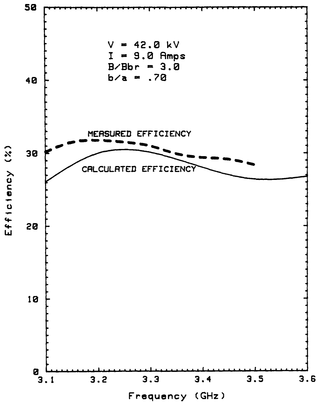
FIGURE 4.22 COMPARISON OF PREDICTED AND MEASURED CONVERSION EFFICIENCY FOR HIGH EFFICIENCY S-BAND TWT
