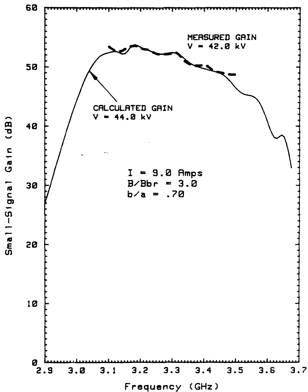
FIGURE 4.21 COMPARISON OF PREDICTED AND MEASURED SMALL SIGNAL GAIN FOR HIGH EFFICIENCY S-BAND TWT
