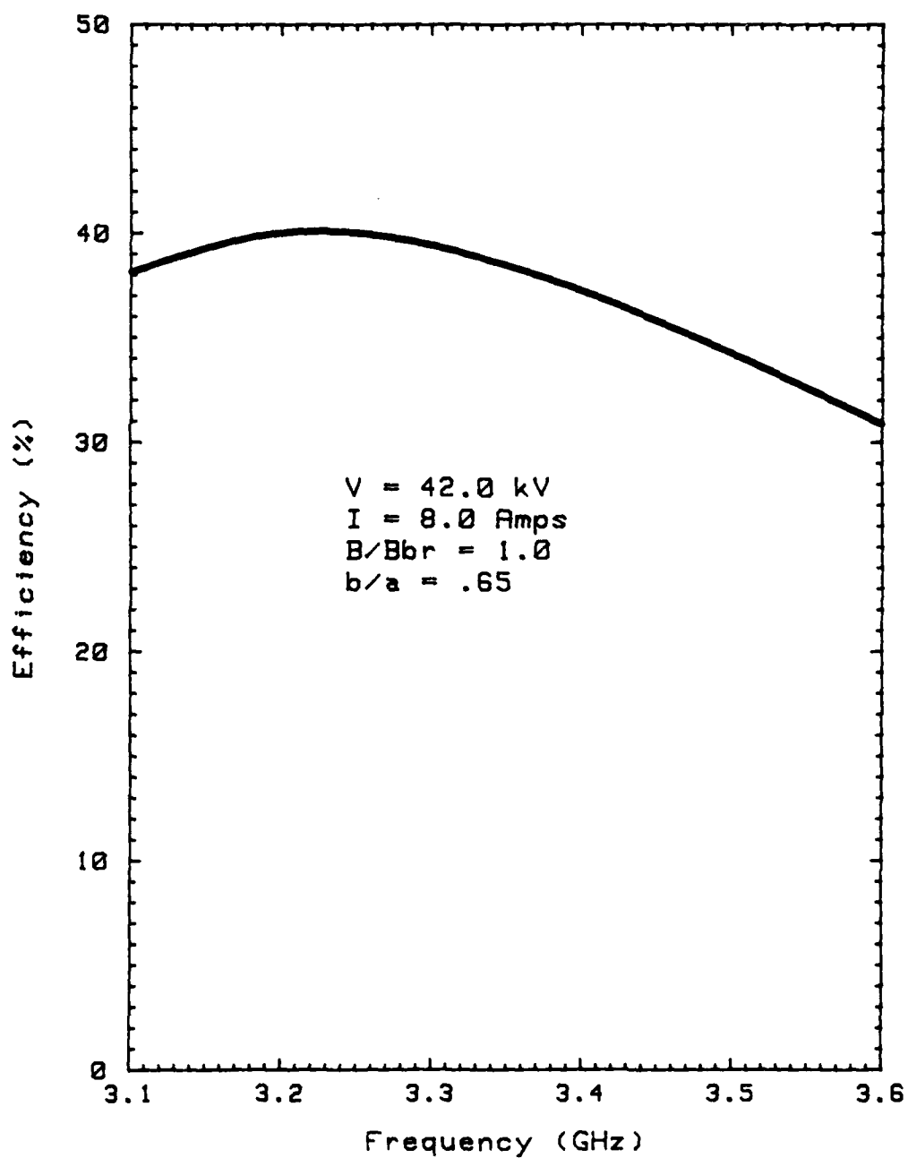
FIGURE 3.9 PREDICTED CONVERSION EFFICIENCY FOR HIGH EFFICIENCY S-BAND TWT
