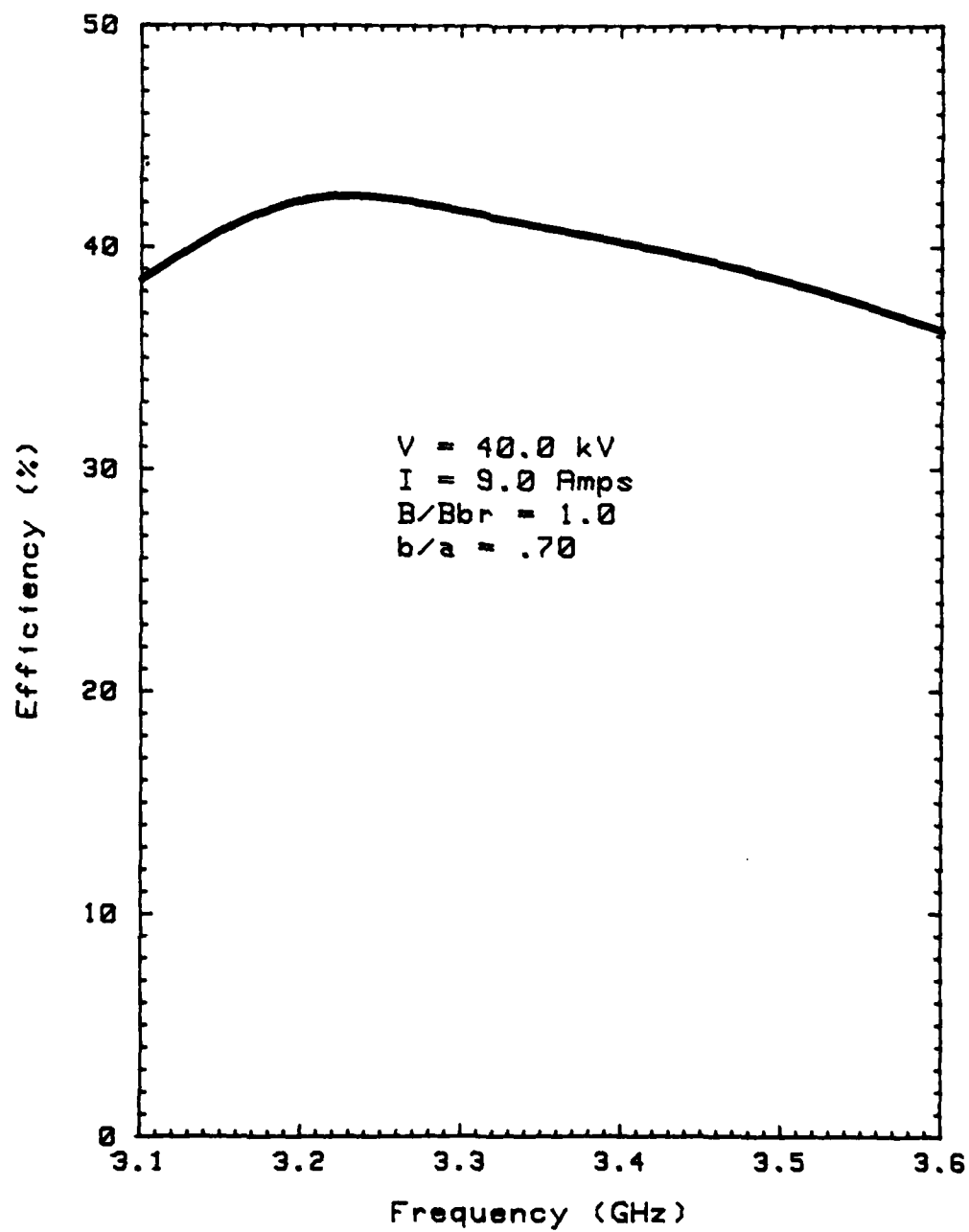
FIGURE 4.25 PREDICTED CONVERSION EFFICIENCY OF S-BAND TWT WITH BRILLOUIN BEAM
