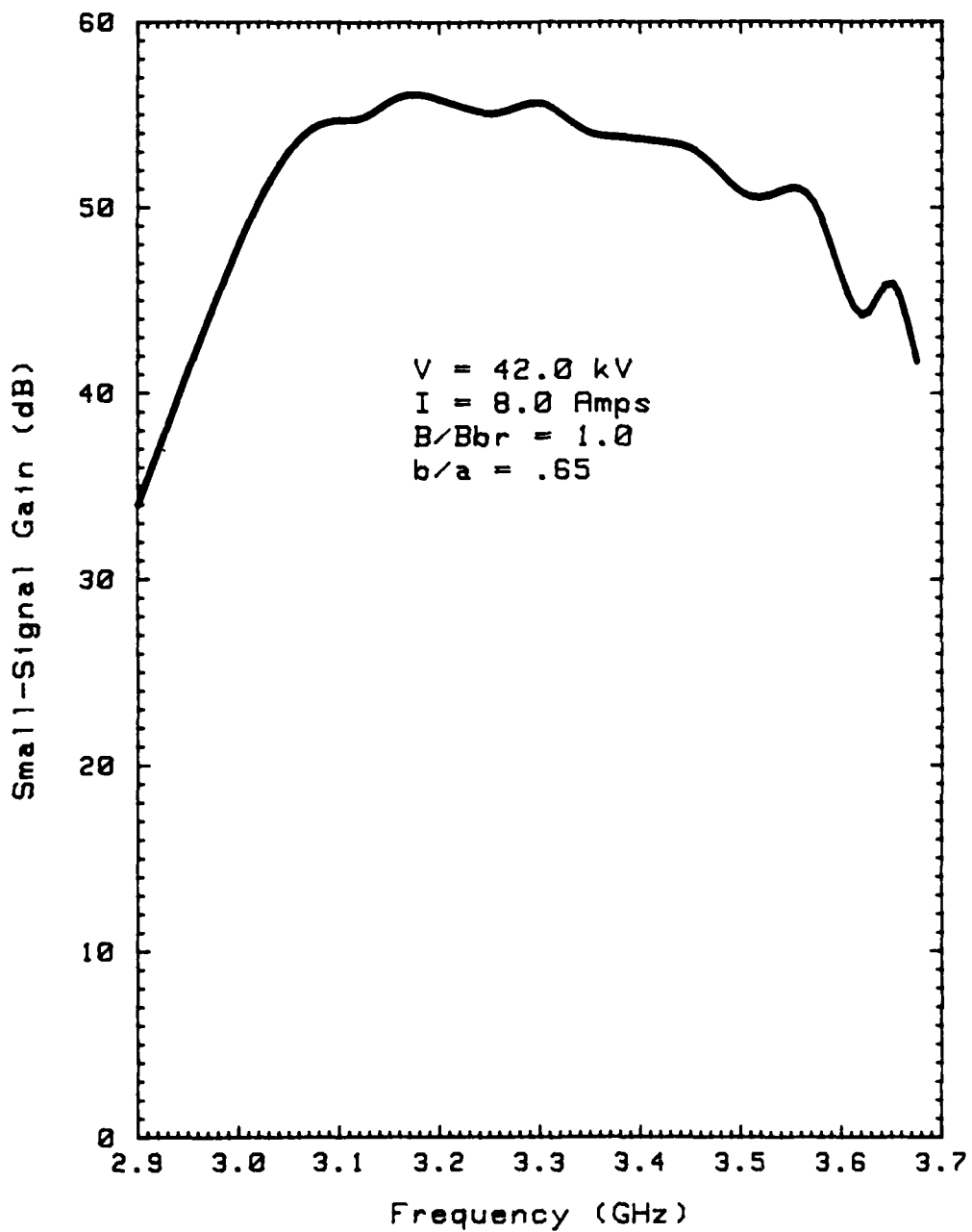
FIGURE 3.8 PREDICTED SMALL SIGNAL GAIN FOR HIGH EFFICIENCY S-BAND TWT
