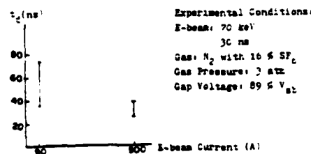
Fig. 7b. Delay Time vs E-beam Current.
