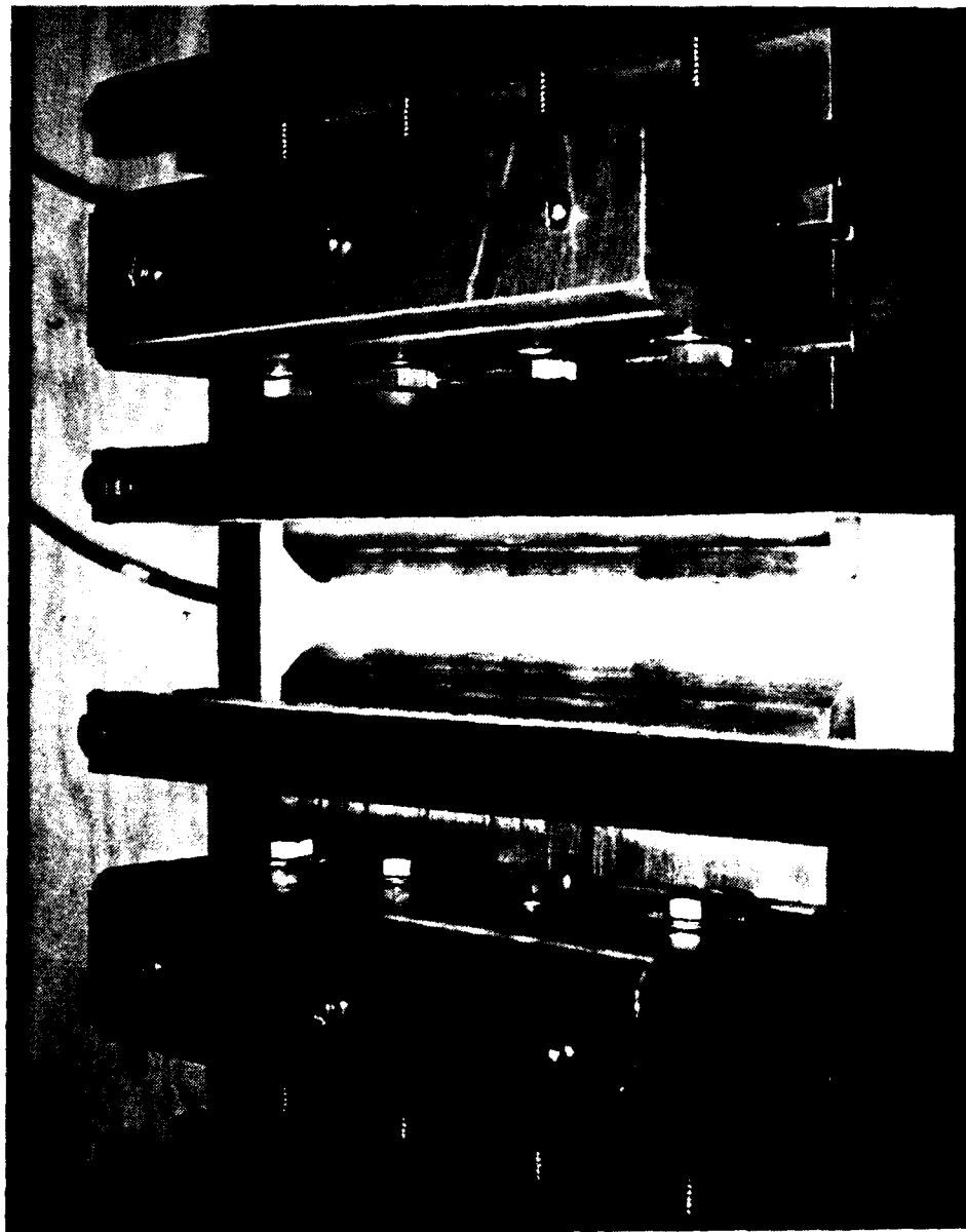
Fig. 14 Discharge Across Delrin, in air, at 45 kV
