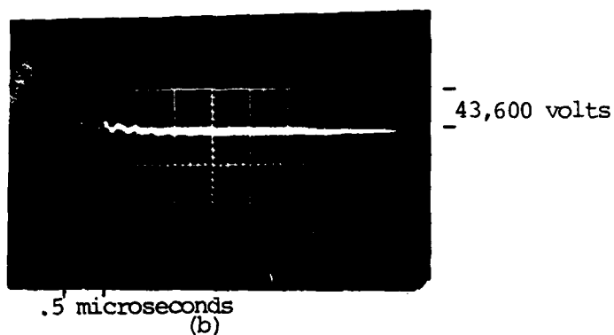
Figure 6 Oscillogram of surface flashover potential across the same Lucite insulator in 1 atmosphere of N_2 after exposure to 80,000 shots in the irradiation chamber.
