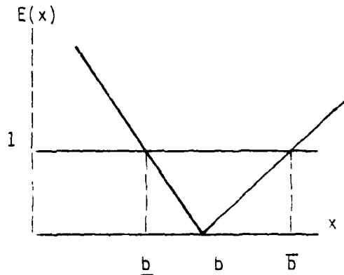
Fig. 1. Piecewise Function for Linear Programming.
