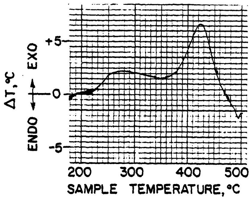
Fig. 4. DTA Results for R-45M with A0
