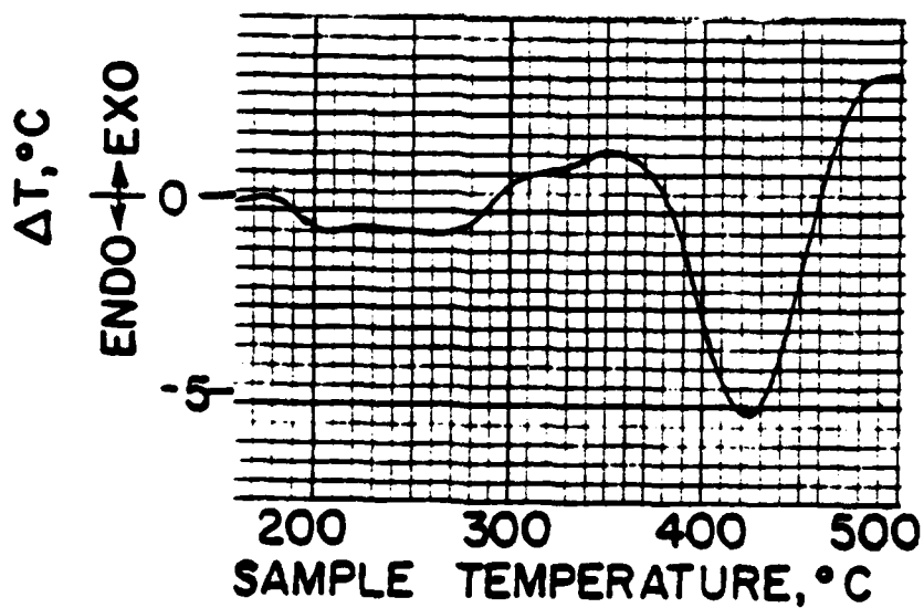
Fig. 14. DTA Results for P1M Fuel
