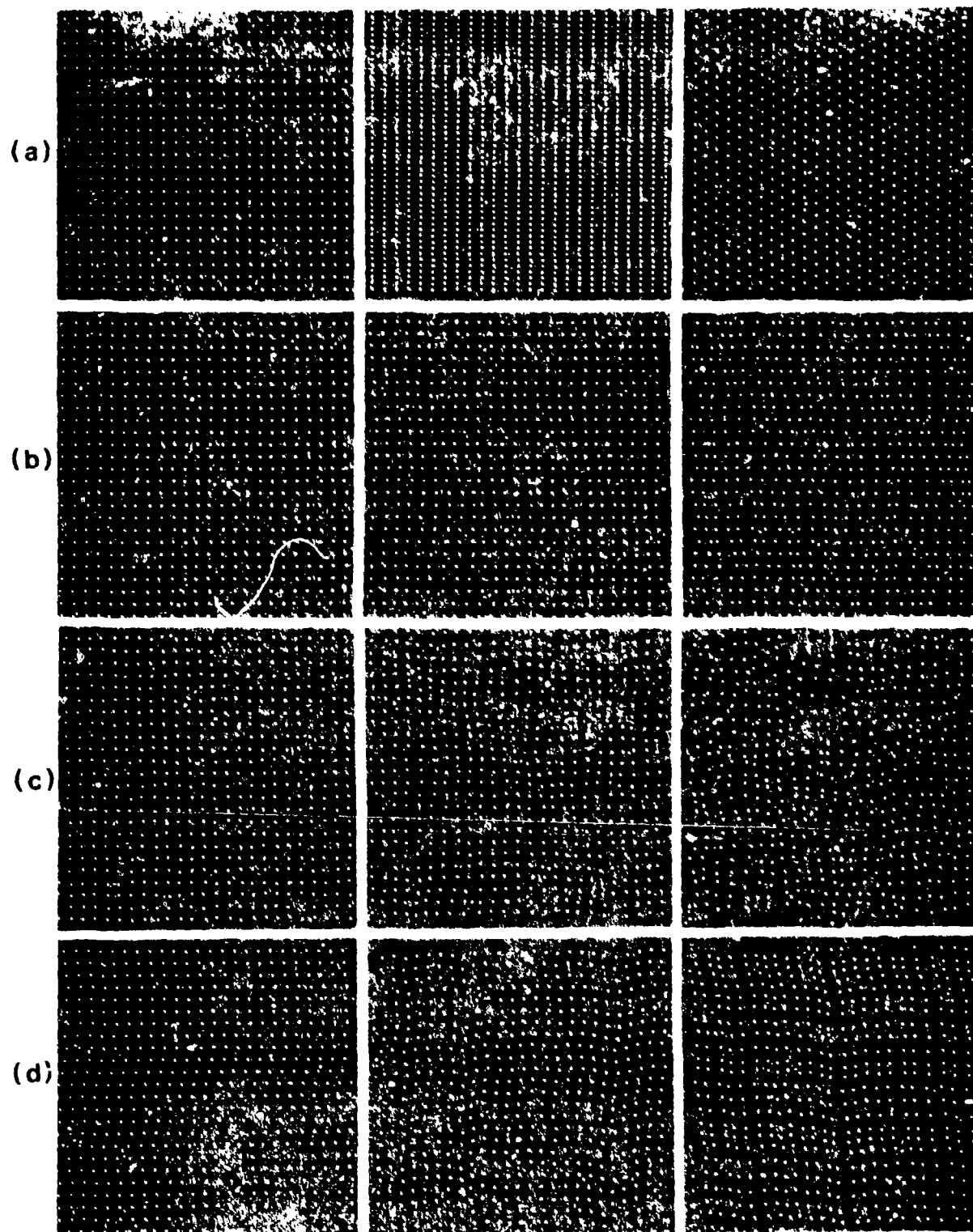
Figure 3-14 Contour-contrast patterns
