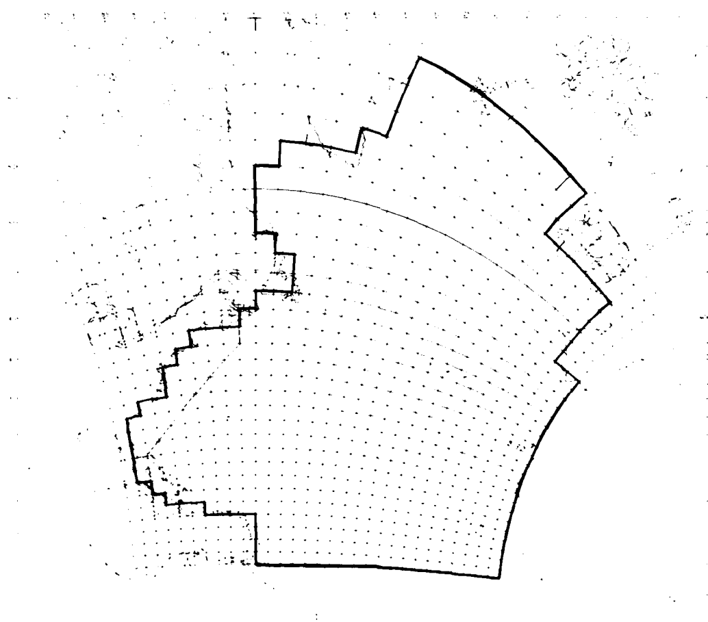
Figure 2. WIS spherical orthogonal grid on a Mercator projection. Heavy dark line is numerical boundary; dashed line is approximate limit of Phase II area
