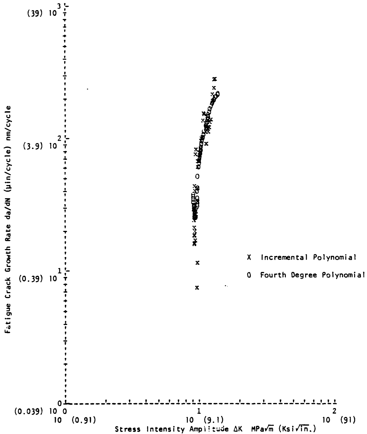
Figure A-3b. Fourth Degree Polynomial Curve Fit, TL Orientation
