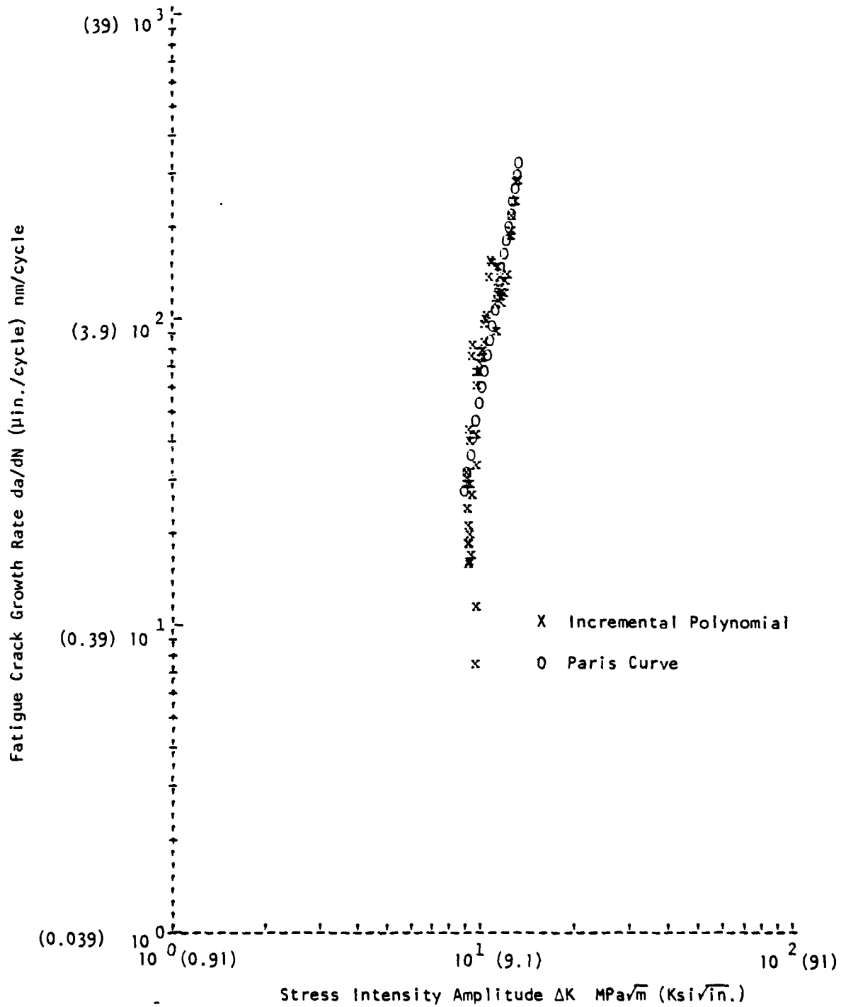
Figure A-1b. Paris Curve Fit, TL Orientation
