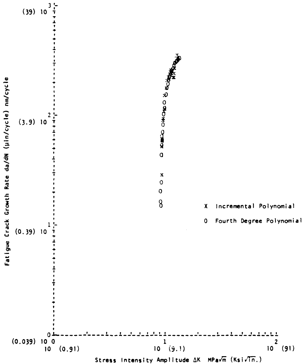
Figure A-3a. Fourth Degree Polynomial Curve Fit, LT Orientation
