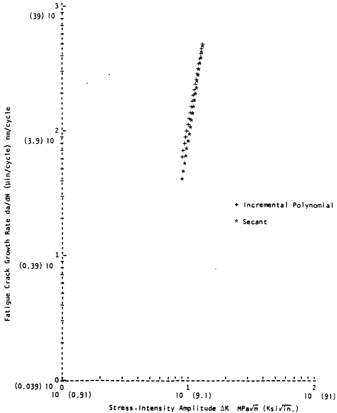
Figure A5a. Comparison of Paris Curves for Incremental Polynomial and Secant Data, LT Orientation
