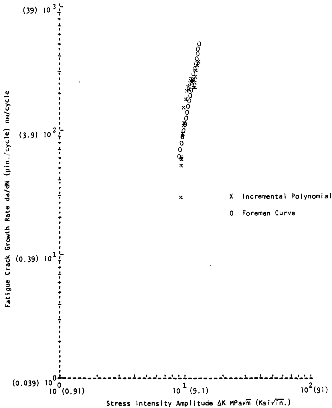
Figure A-2a. Foreman Curve Fit, LT Orientation
