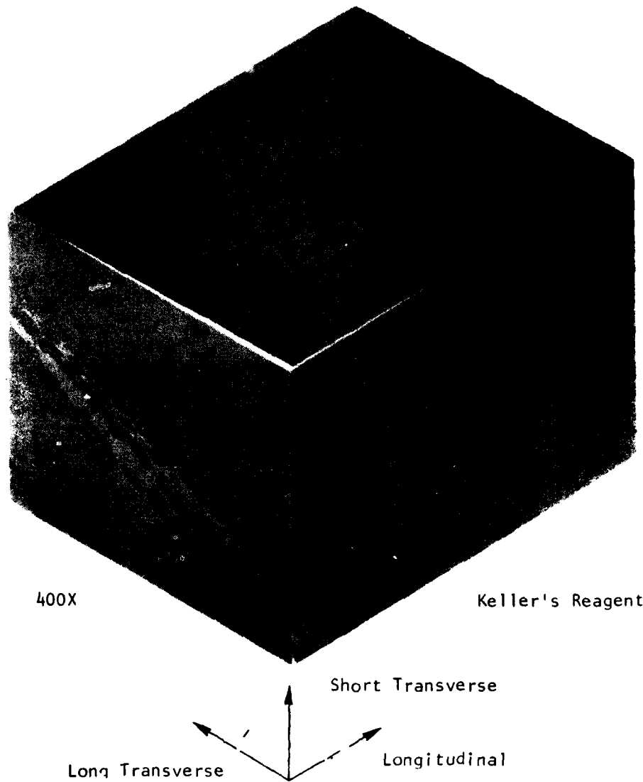
Figure 1b. Microstructural Montage of 7050 Al, Shock Hardened plus 250°F - 4 hour Age
