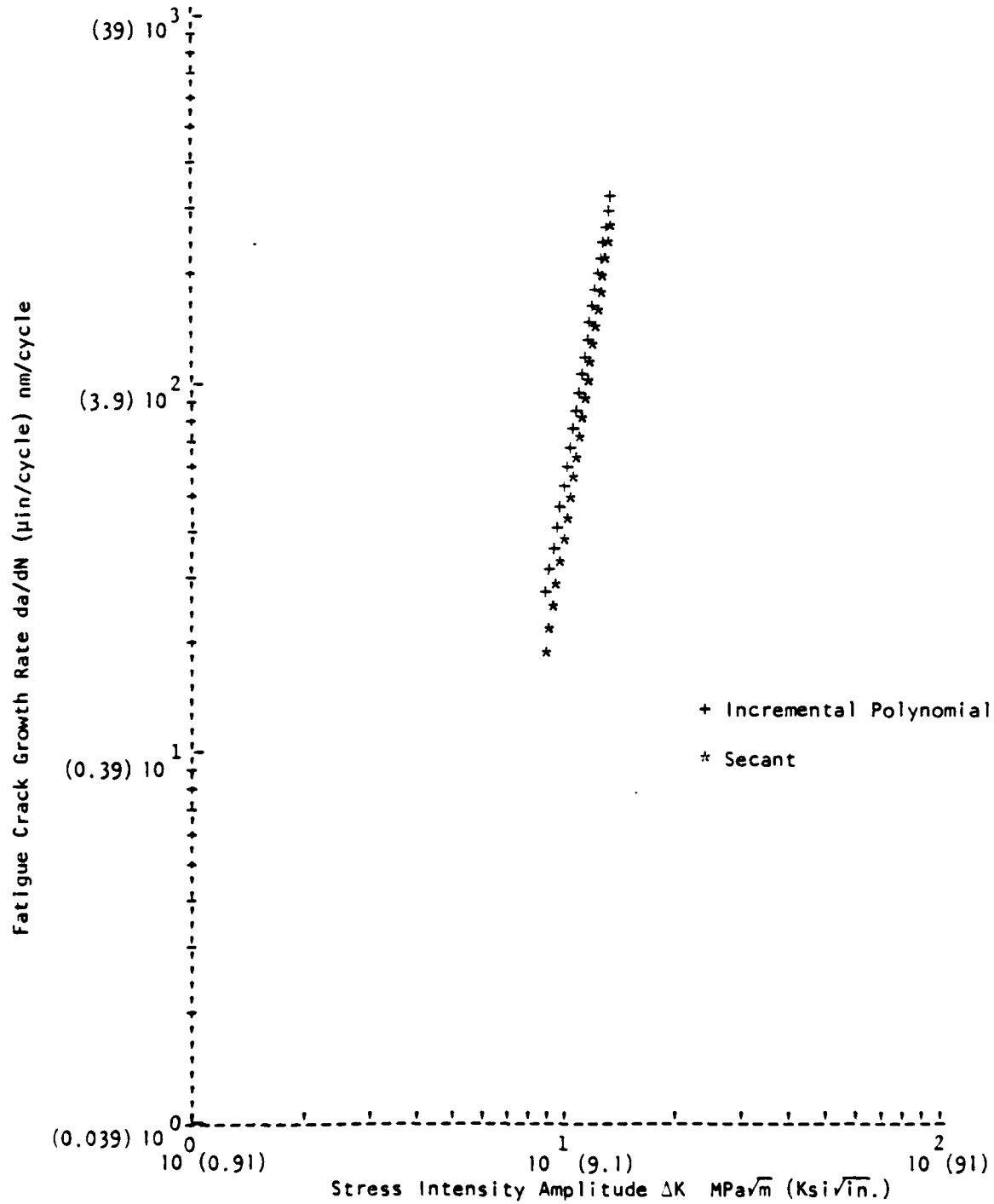
Figure A-5b. Comparison of Paris Curves for Incremental Polynomial and Secant Data, TL Orientation
