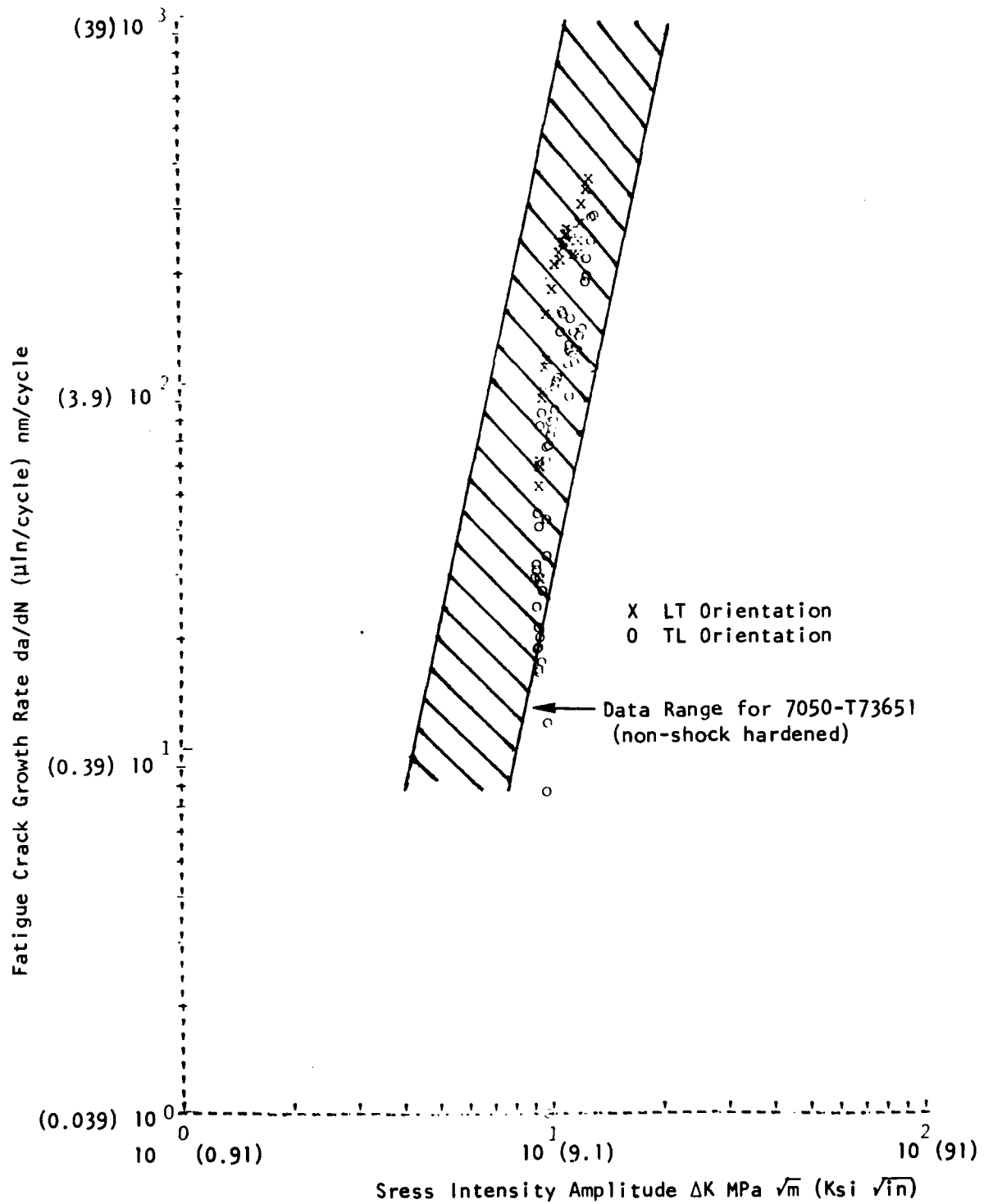
Figure 5. Comparison of Fatigue Crack Growth Rate Test Results for Shock Hardened 7050 Alloy with Data Range for Non-Shock Hardened 7050-T73651 (reference (d)).
