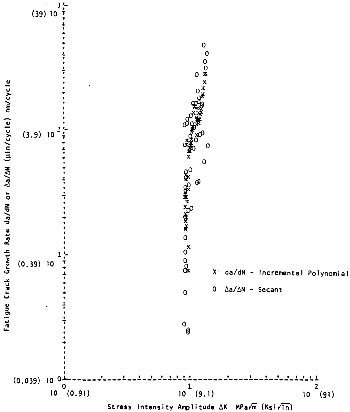
Figure A-4b. Comparison of Secant vs Incremental Polynomial Methods of Data Reduction, TL Orientation
