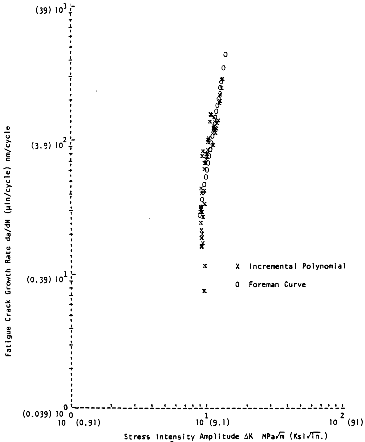
Figure A-2b. Foreman Curve Fit, TL Orientation
