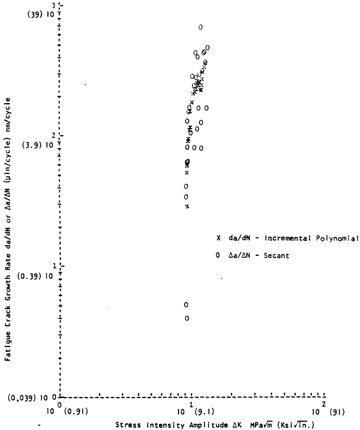
Figure A-4a. Comparison of Secant vs. Incremental Polynomial Methods of Data Reduction, LT Orientation
