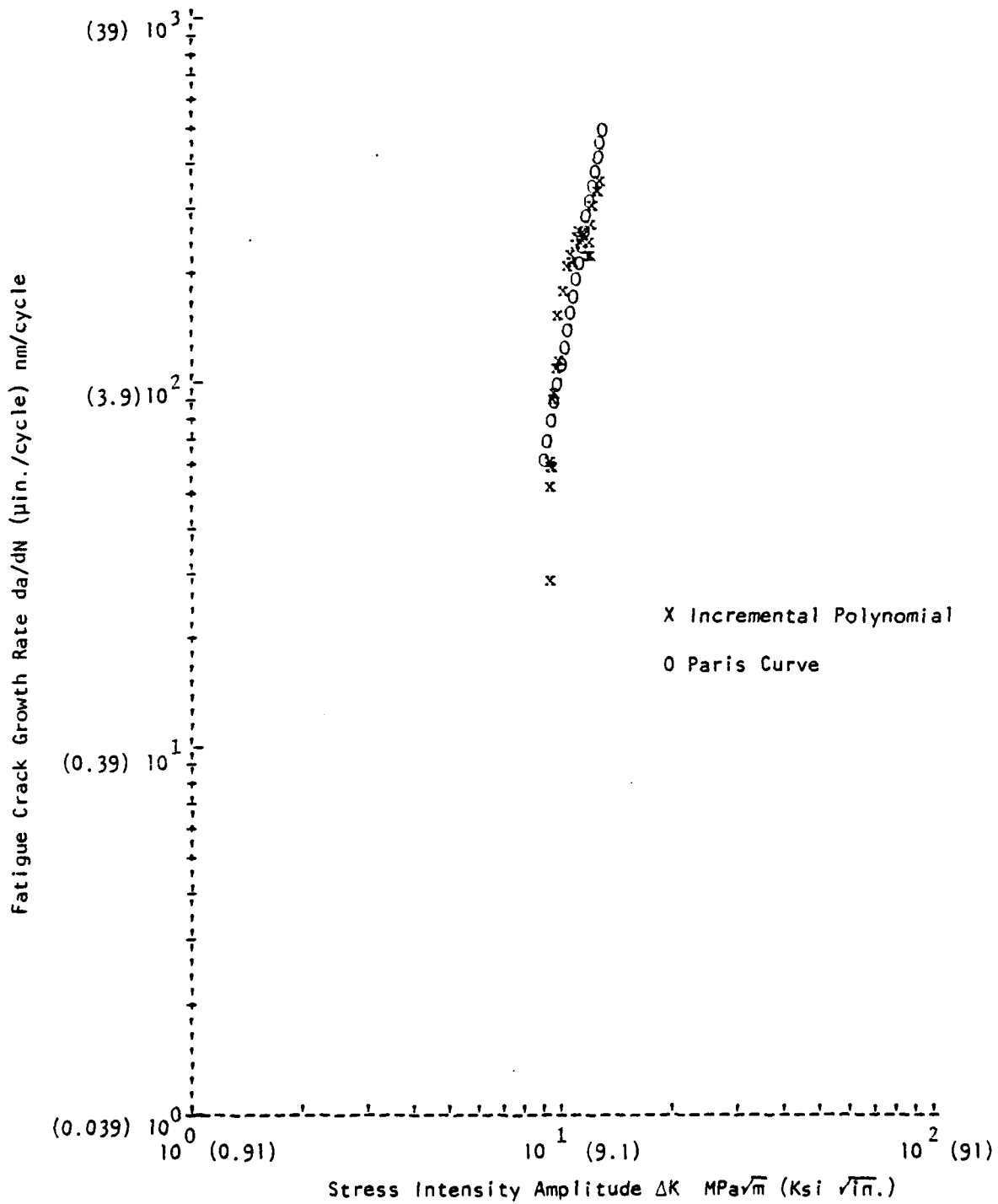
Figure A-1a. Paris Curve Fit, LT Orientation
