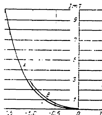
Fig. 15. Comparison of the alleged parts T (6.19) for M-profiles/airfoils of different types (A - type of the profile/airfoil Fig. 12; B - type of the profile/airfoil Fig. 14).
