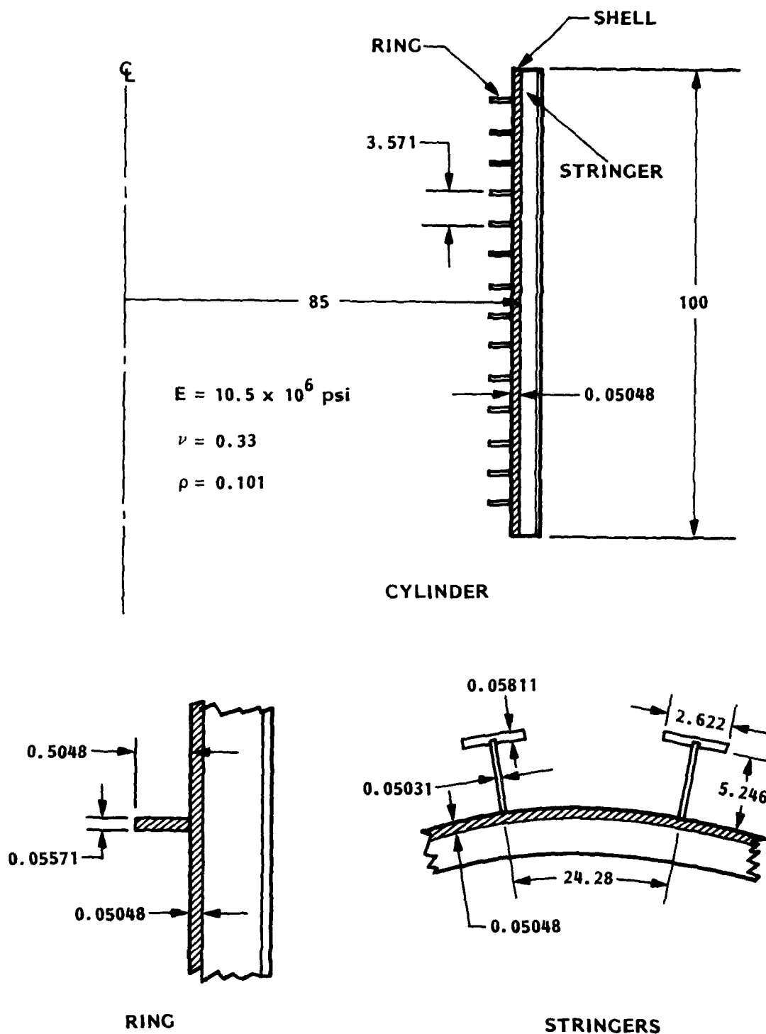
Figure 20. Ring and stringer stiffened cylindrical shell under pure torsion. The dimensions correspond to an optimum design obtained by Simitse and Giri [63] (See Table 4, Case 2)
