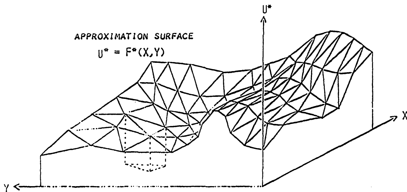
FIGURE 1-B. APPROXIMATE SOLUTION REPRESENTED BY PIECEWISE LINEAR FUNCTIONS MAKING UP HEXAGONALLY CONNECTED TRIANGULAR FACETS. IFE UNKNOWNNS ARE \{a1_j, \dots, aN_j, x_j, y_j\}
