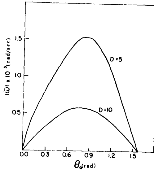
Fig. 11. Angular velocity of a cylinder falling towards a horizontal plane for various initial orientations (in rads) at \mathcal{D}_{1,c} = 10 , 5. Same cylinders' and liquids' properties as of Fig. 5.
