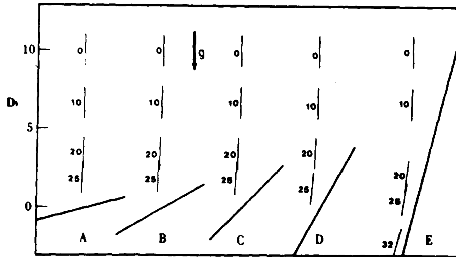
Fig. 12. Time history of a cylinder falling towards a plane inclined to the horizontal at angles: A-15°, B-30°, C-45°, D-60°, E-75°; initial orientation - vertical; \mathcal{D}_{1,c} = 10 . Numbers near positions indicate elapsed time in seconds. Same cylinders' and medium's properties as of Fig. 5.
