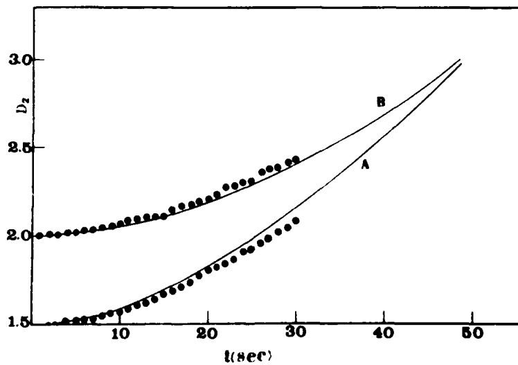
Fig. 6. Drift displacement and orientation of a cylinder near a vertical wall as a function of time. Same parameters as of Fig. 5 except for : A. D_{2c} = 1.5 \text{ l} ; \theta_0 = 89^\circ . B: \theta_0 = 21 , \theta_0 = 93^\circ .
