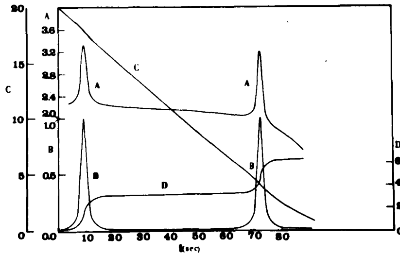
Fig. 20. Change with time of the vertical velocity, A (in 1/sec), angular velocity B (in rads/sec), distance from the wall C (in l), and orientation angle D (in rads) of a cylinder within a Couette flow.
