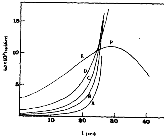
Fig. 18. Angular velocity of a cylinder falling towards an inclined plane. Same parameters and conditions as of Fig. 12. ( D_2 reaches a minimum at the point P).
