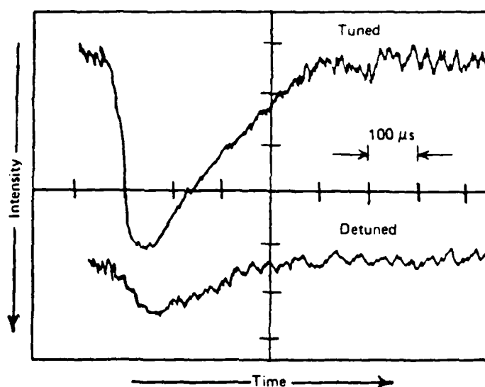
Figure 22. Illustration of Cavity Experiments for One Experimental Condition. Plenum Conditions Correspond to 3820 K and 3.1 Atm. The cavity Pressure Was 30 torr With X_{Ar}: X_{HI}: X_H = 84:11:5
