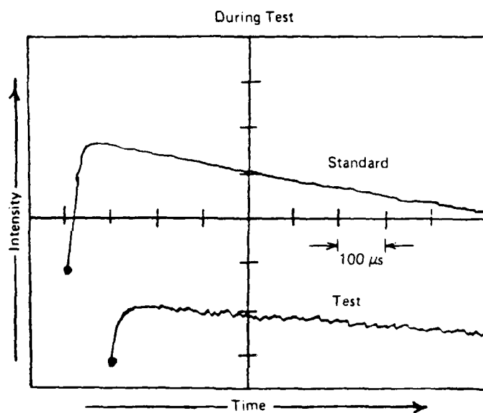
Figure 25(b). Illustration of Gain Measurement In 12-Inch System. Plenum Conditions Were 4100 K and 3.7 Atm. Cavity Pressure Measured at 22 torr With X_{Ar} : X_{HI} : X_{H_2} 80:14:6. A 35% Loss Is Recorded. During Test
