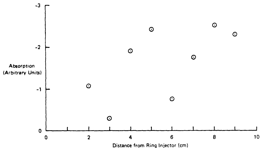
Figure 50. Relative Absorption at 2062Å as a Function of Distance Downstream from Ring Injector
