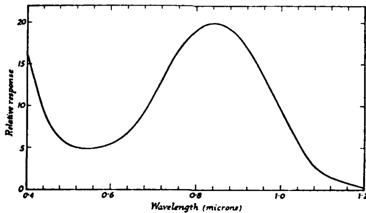
Fig. 2 — Relative Wavelength Response of the S-1 Photocathode
