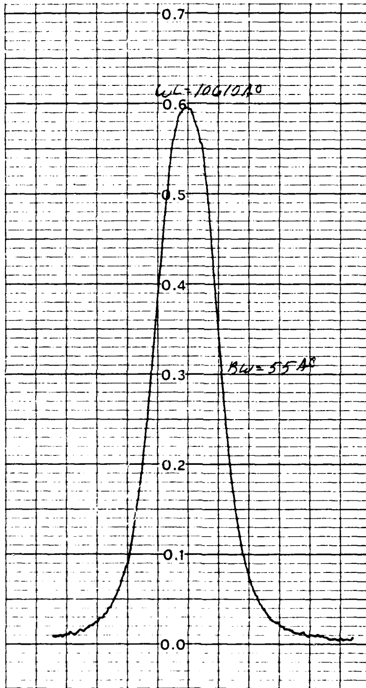
Fig. 3 - Spectrograph Trace of Narrow-Band-Pass Filter Centered at 1.061 \mu\text{m}
