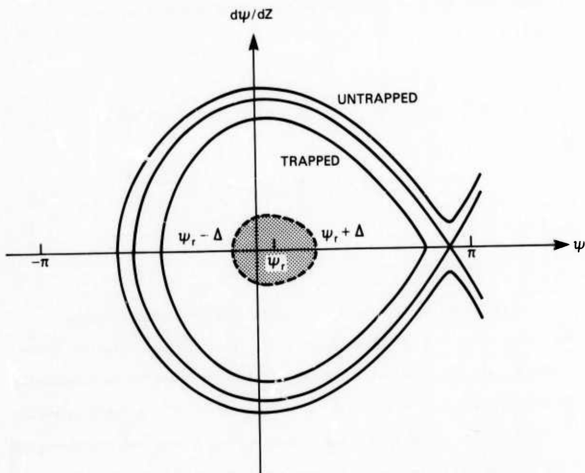
Fig. 1 — Schematic representation of phase space distribution about the resonant phase, showing the separatrix for a tapered wiggler
