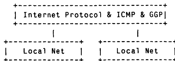
Gateway Protocols
