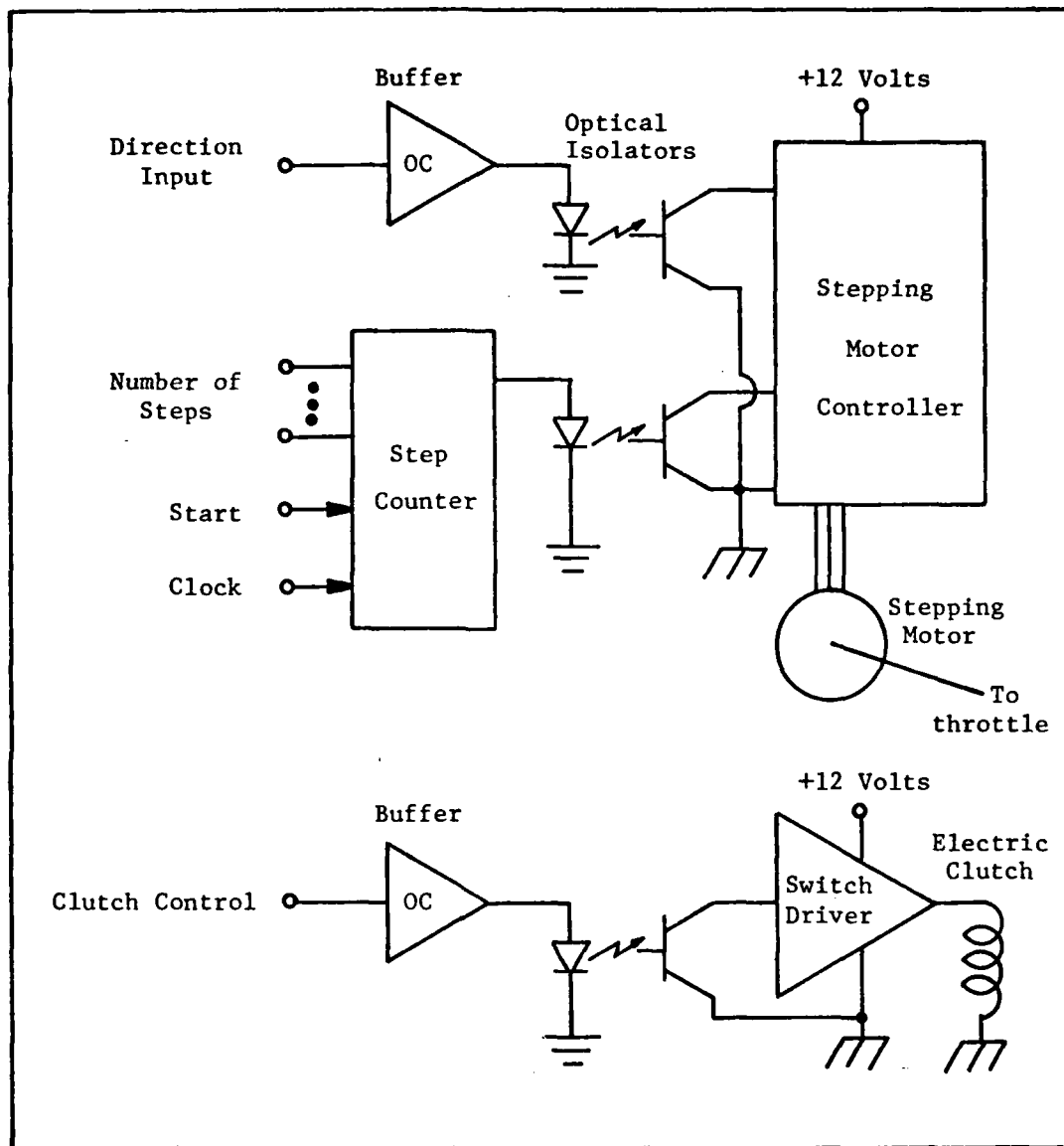
Fig. 6. Function Diagram of Hybrid Controller
