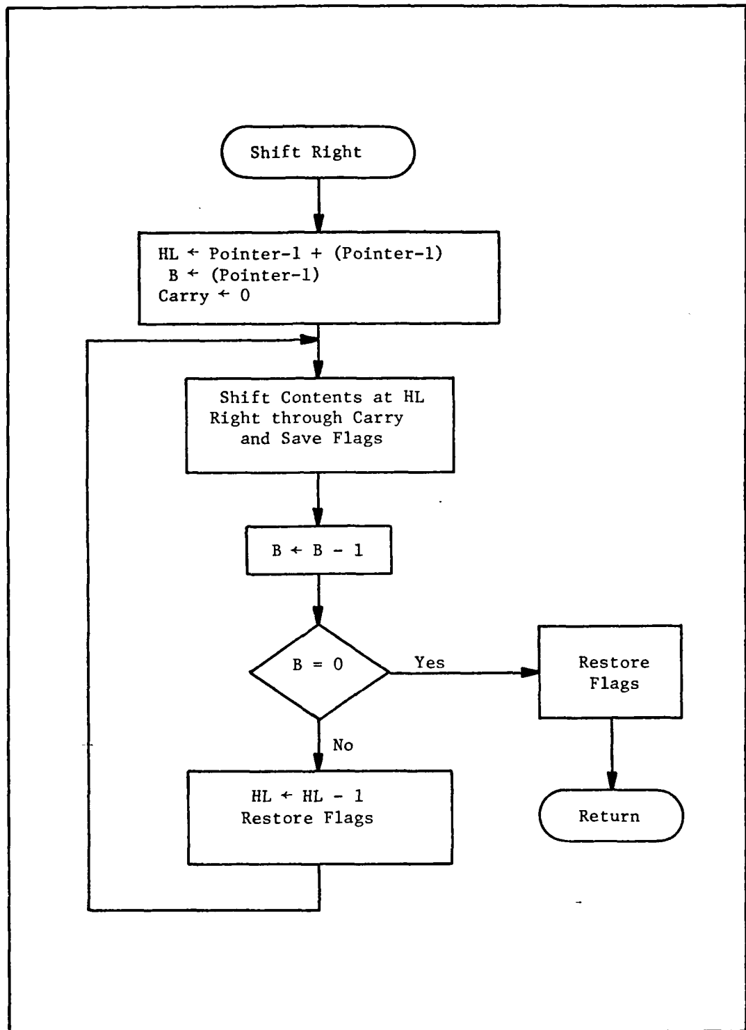
Fig. 36. Vector Shift Right (RSHIFT) Flow Chart
