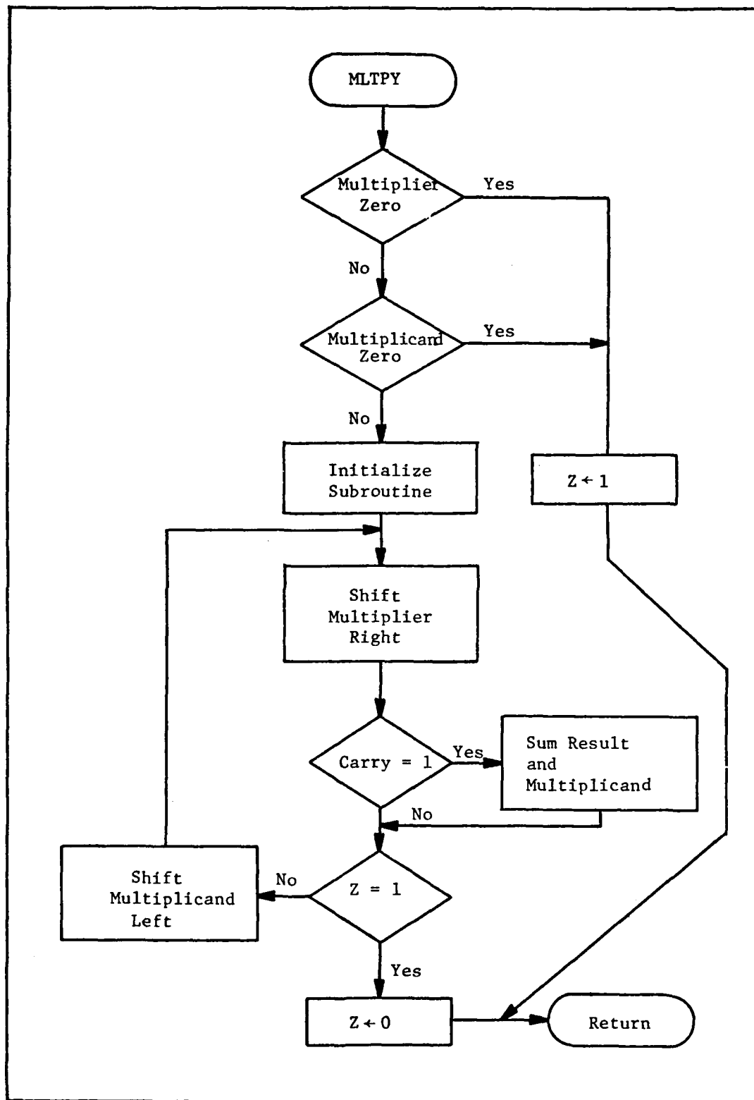
Fig. 35. Multiplication Subroutine (MLTPY) Flow Chart
