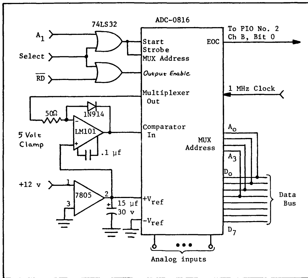
Fig. 18. Data Acquisition System Interface Logic
