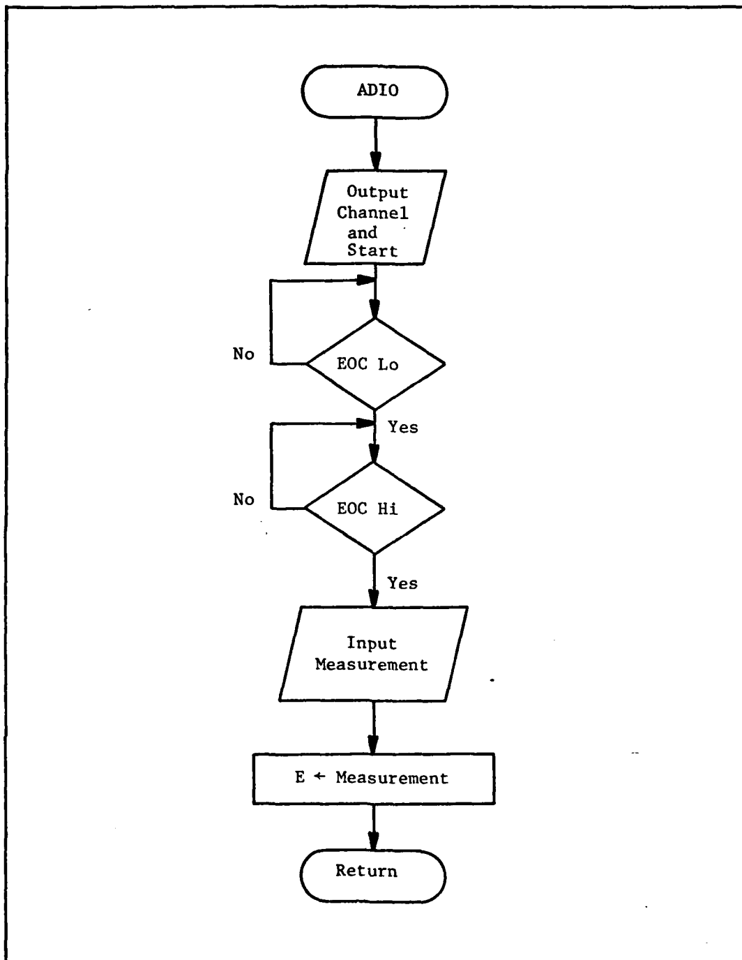
Fig. 33. Analog to Digital Input Subroutine Flow Chart
