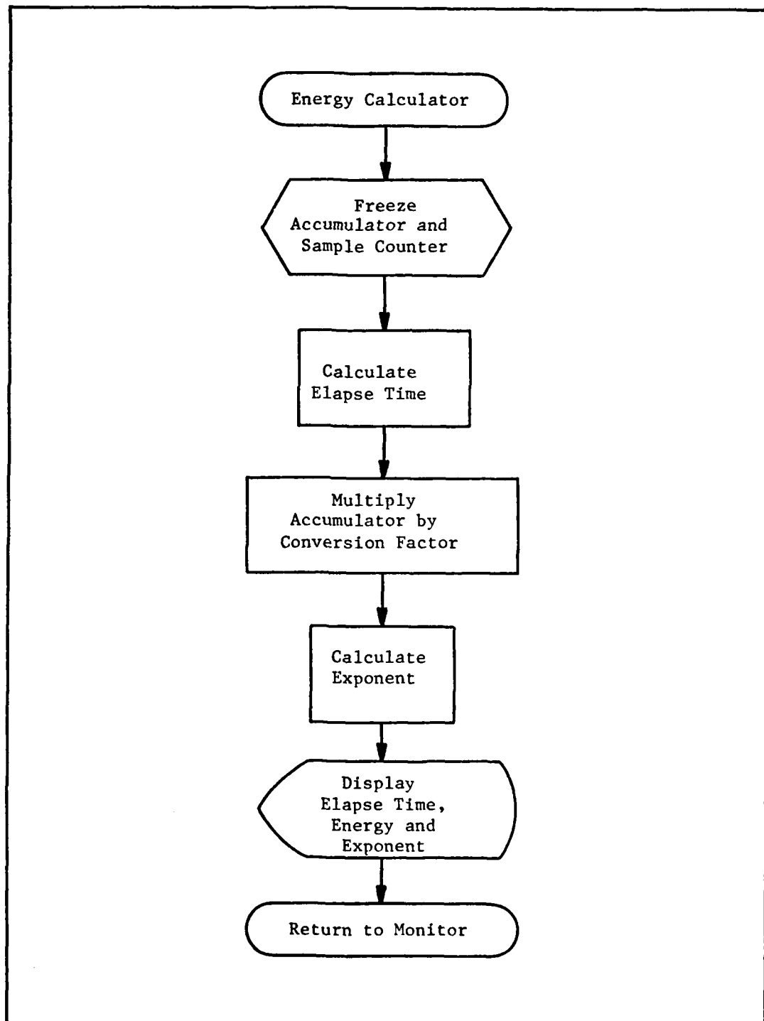
Fig. 12. Energy Calculation Flow Chart
