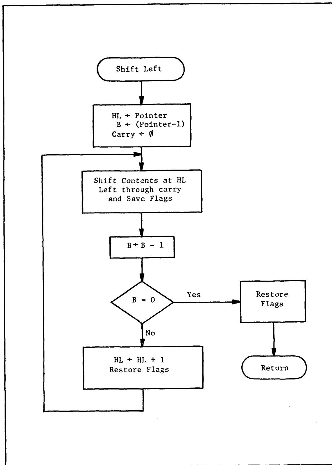
Fig. 37. Vector Shift Left (LSHIFT) Flow Chart
