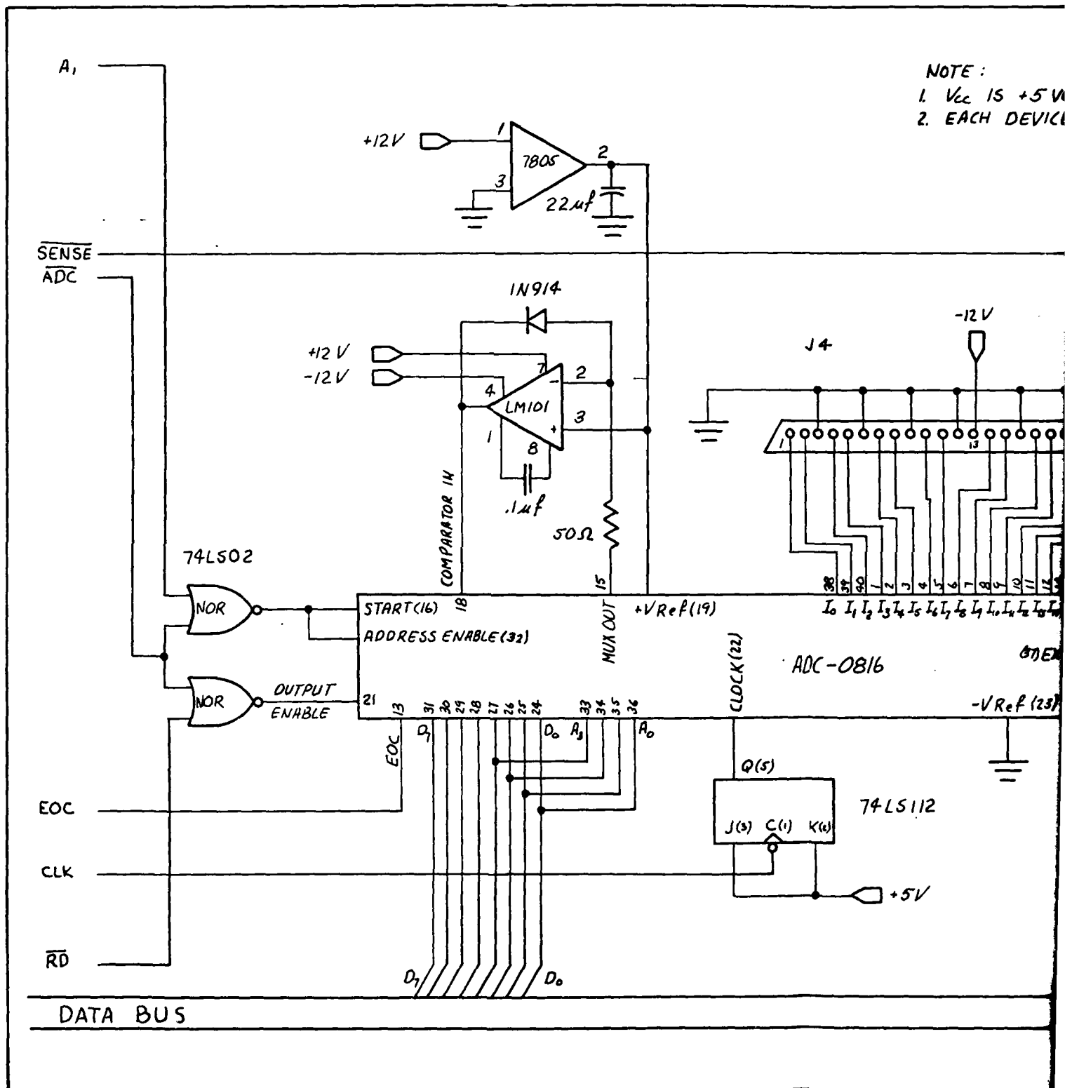
Fig. 16. Microcomputer Schematic Diagram, A/D Converter and Sense (Sheet 5 of 5)
