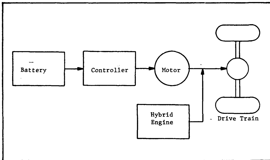
Fig. 2. Parallel Hybrid Vehicle Block Diagram (Ref. 2)
