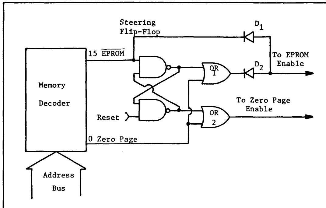
Fig. 17. Memory Overlay Logic Diagram
