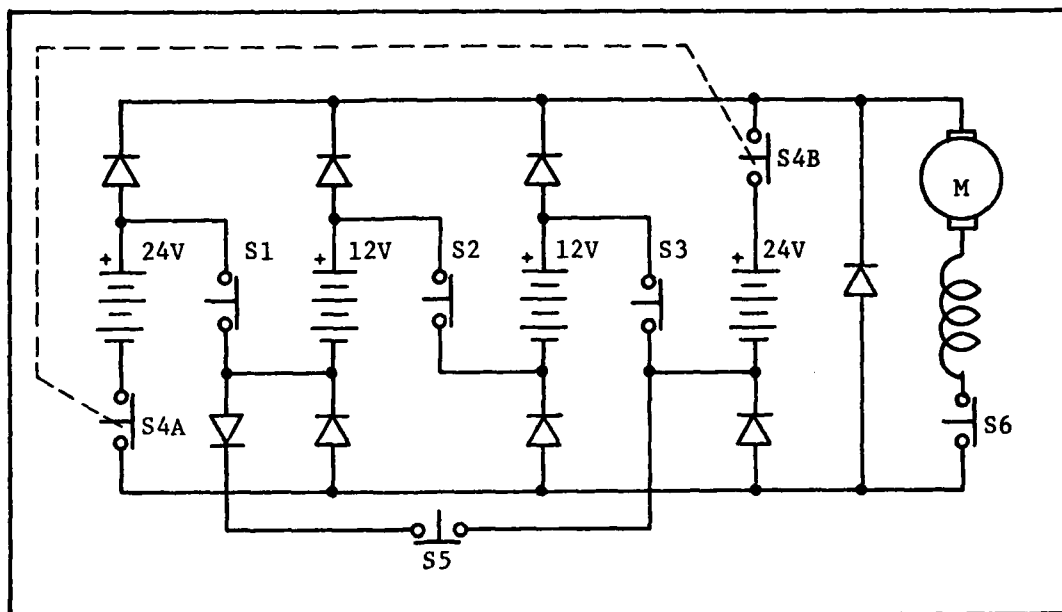
Fig. 26. Existing 5 Step Battery Switching System
