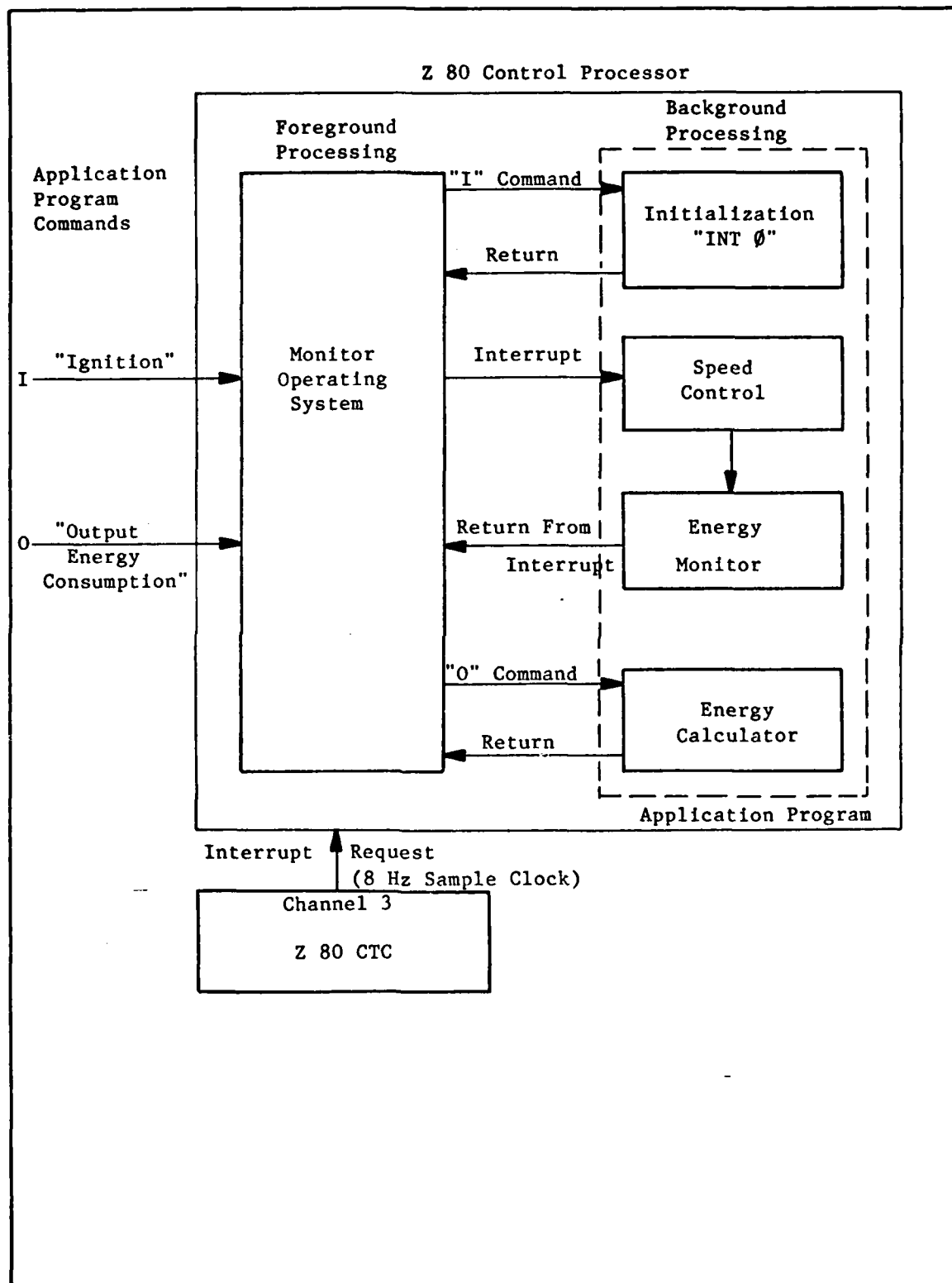
Fig. 8. Software Flow Diagram for the Control System
