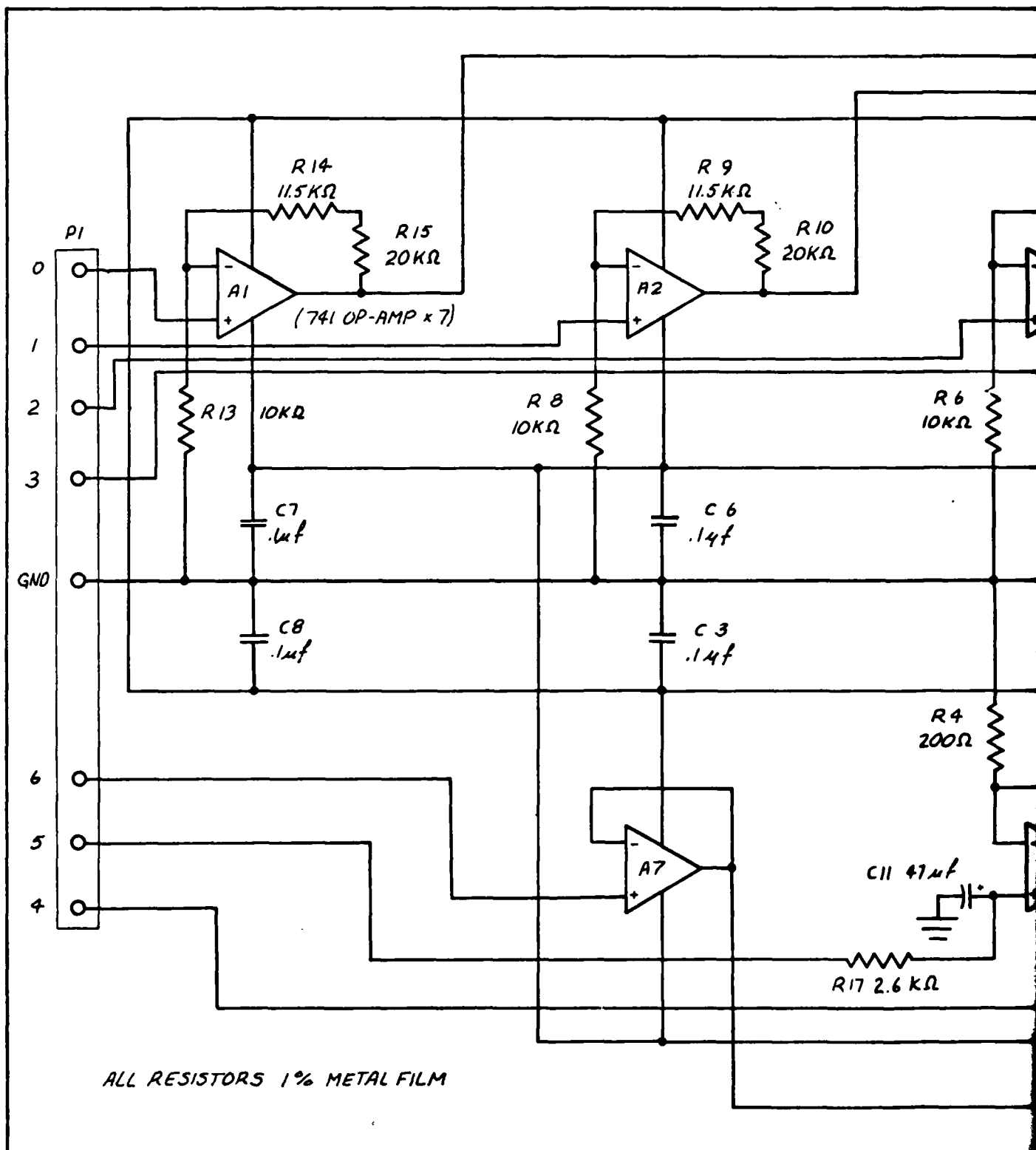
Fig. 25. Analog Input Amplifiers Schematic Diagram
