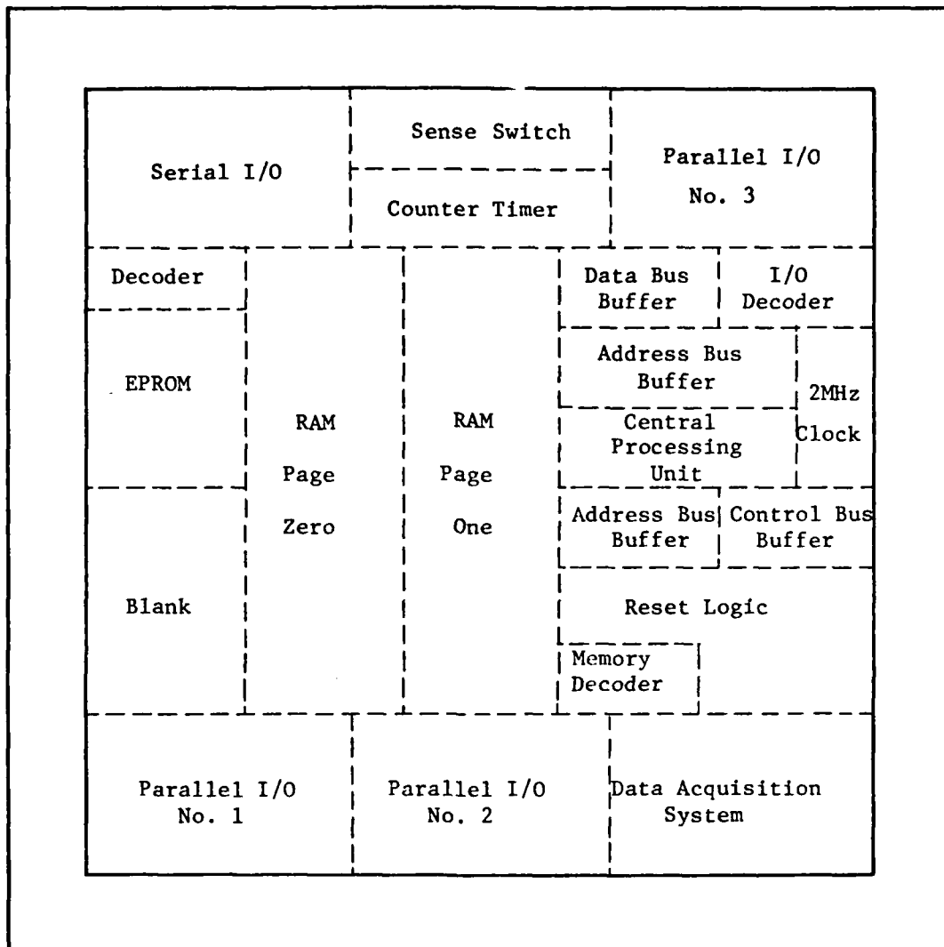
Fig. 15. Functional Layout of Microcomputer
