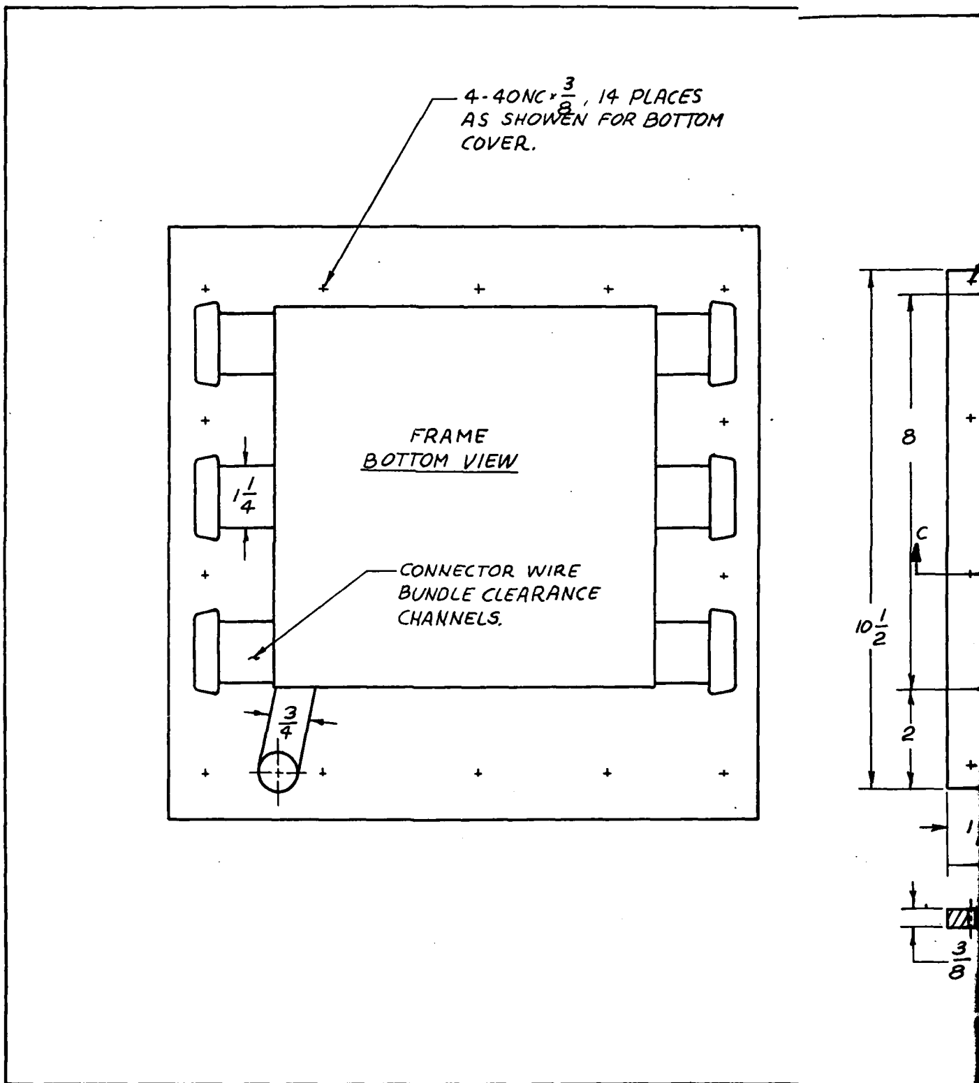
Fig. 23. Microcomputer Enclosure, Frame and Bottom Cover (Sheet 2 of 3)
