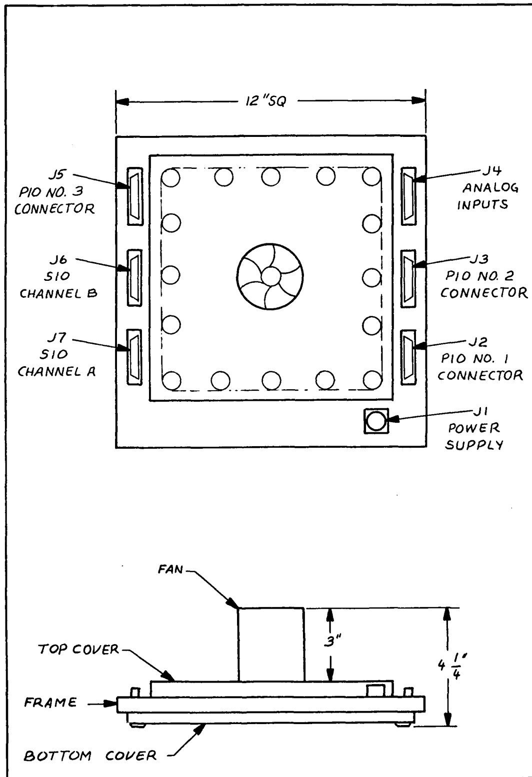
Fig. 21. Outline Drawing of Microcomputer and Connector Designation
