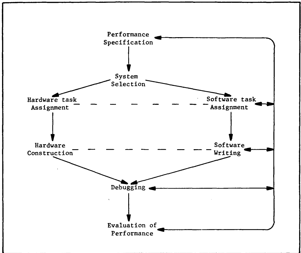
Fig. 1. Design Methodology (Ref. 7)
