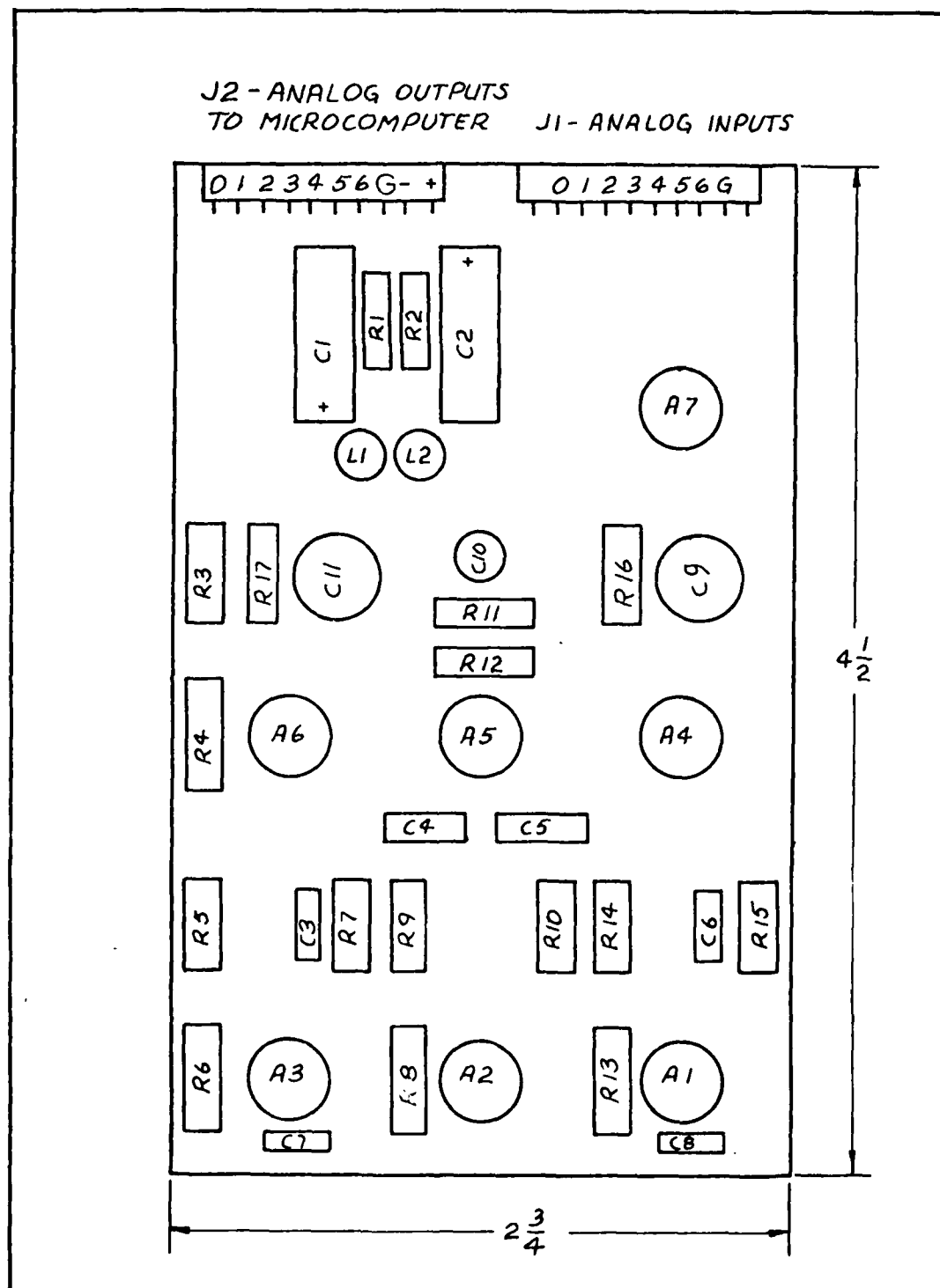
Fig. 24. Component Layout for Analog Input Amplifiers.
