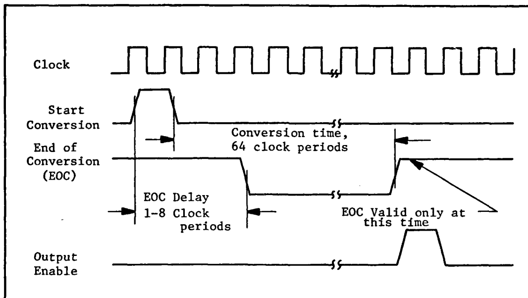
Fig. 19. End of Conversion Timing Diagram
