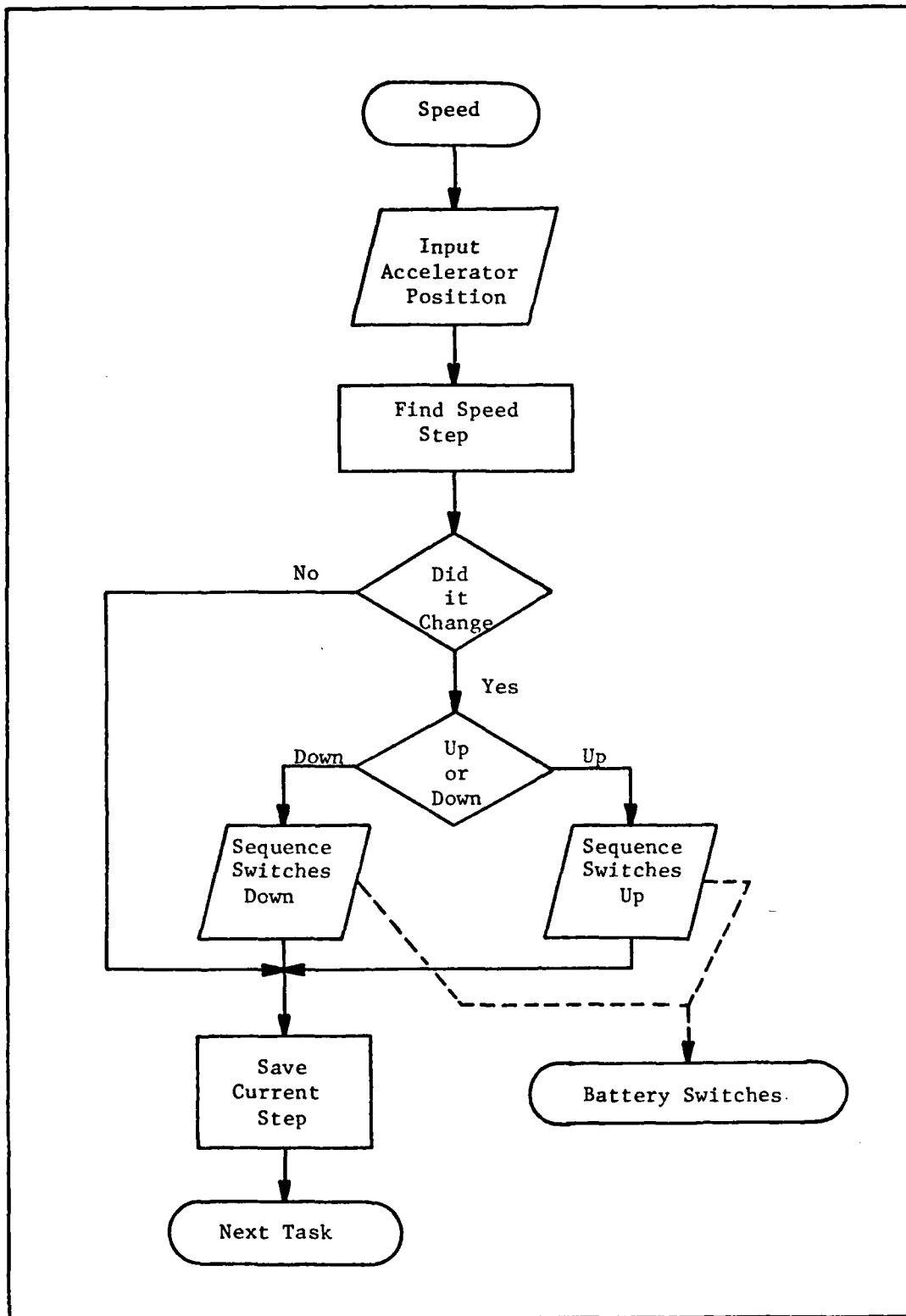
Fig. 9. Speed Control Flow Chart
