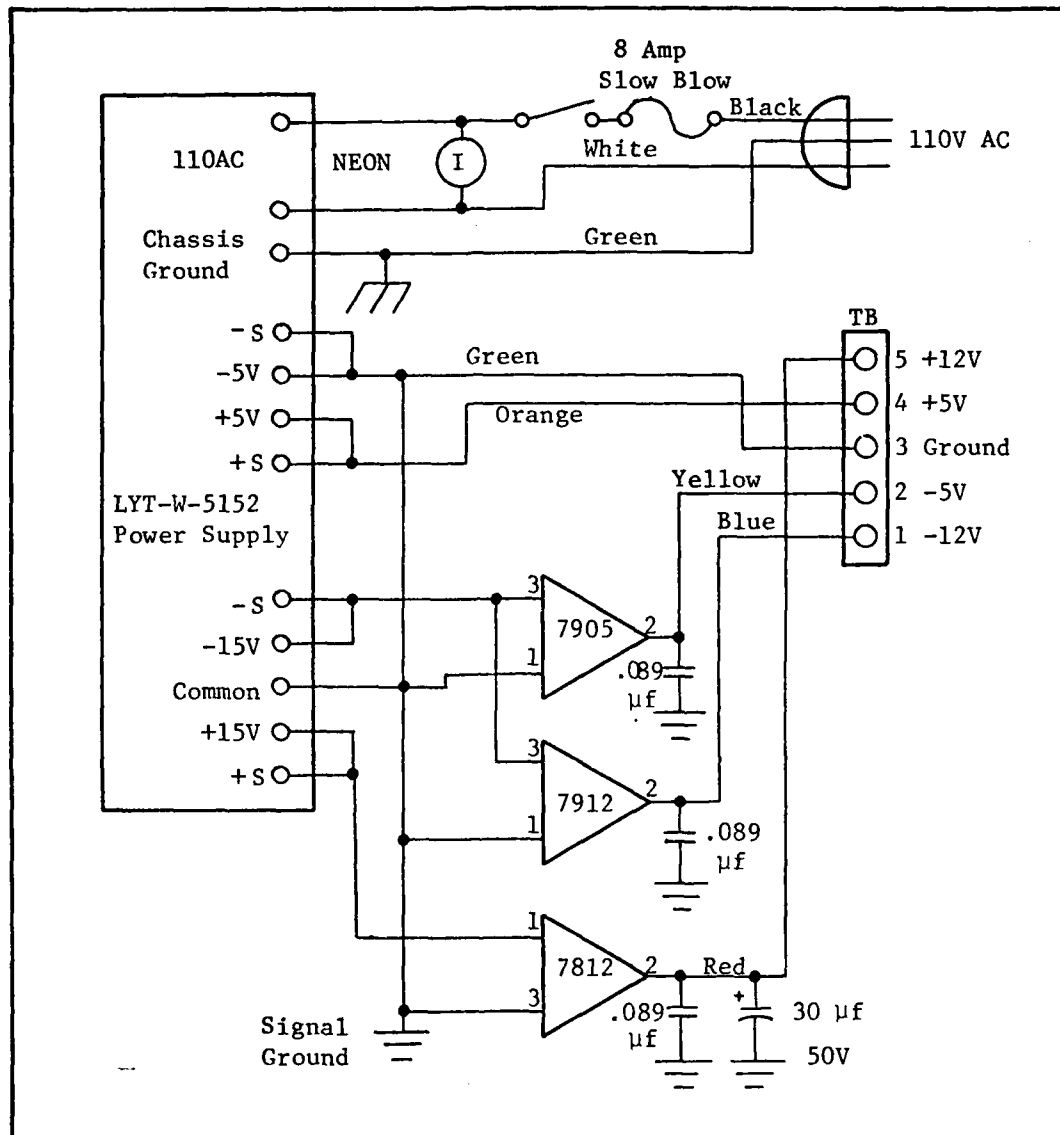
Fig. 29. Electrical Diagram of Power Supply
