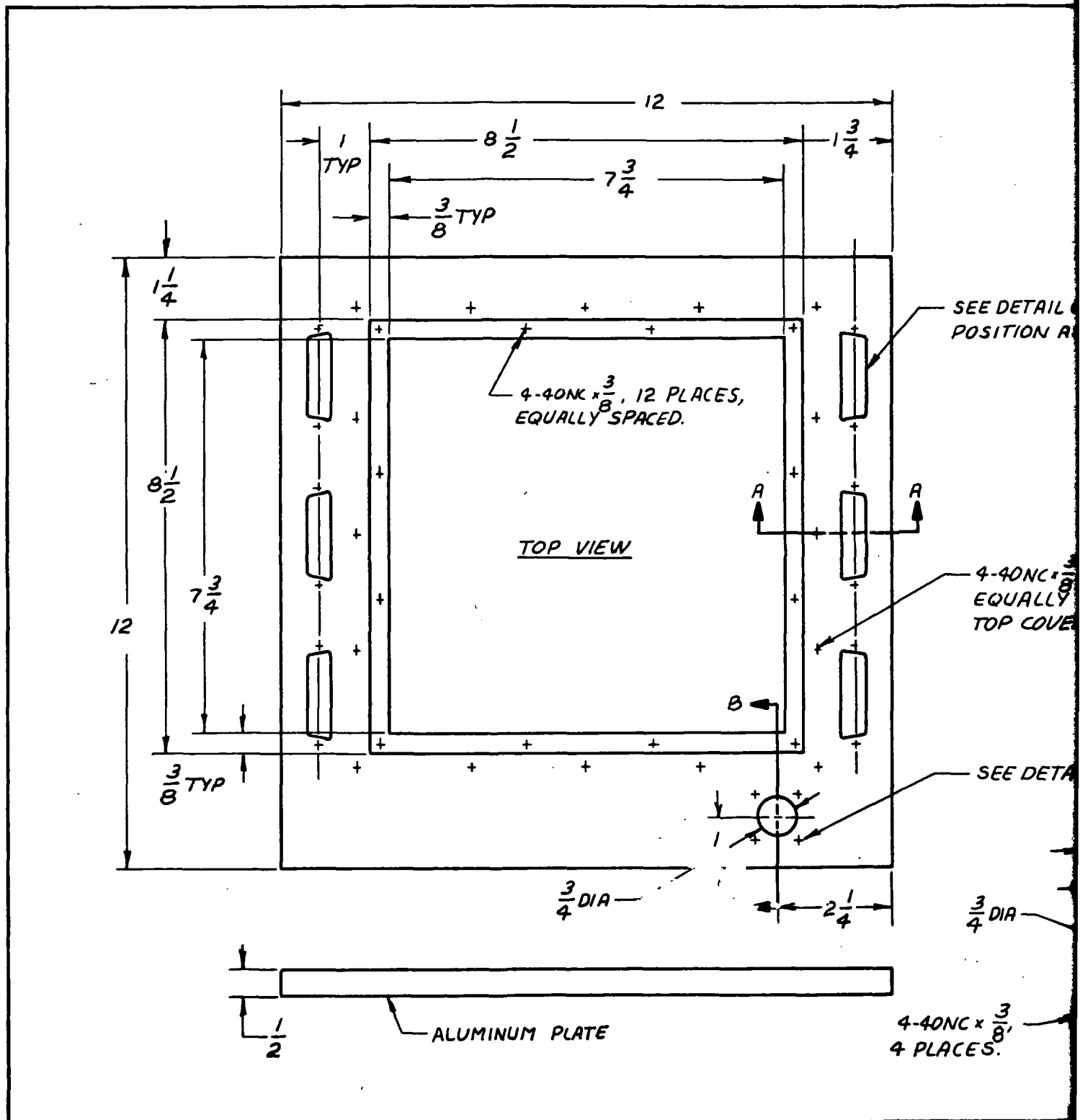
Fig. 23. Microcomputer Enclosure, Frame (Sheet 1 of 3)
