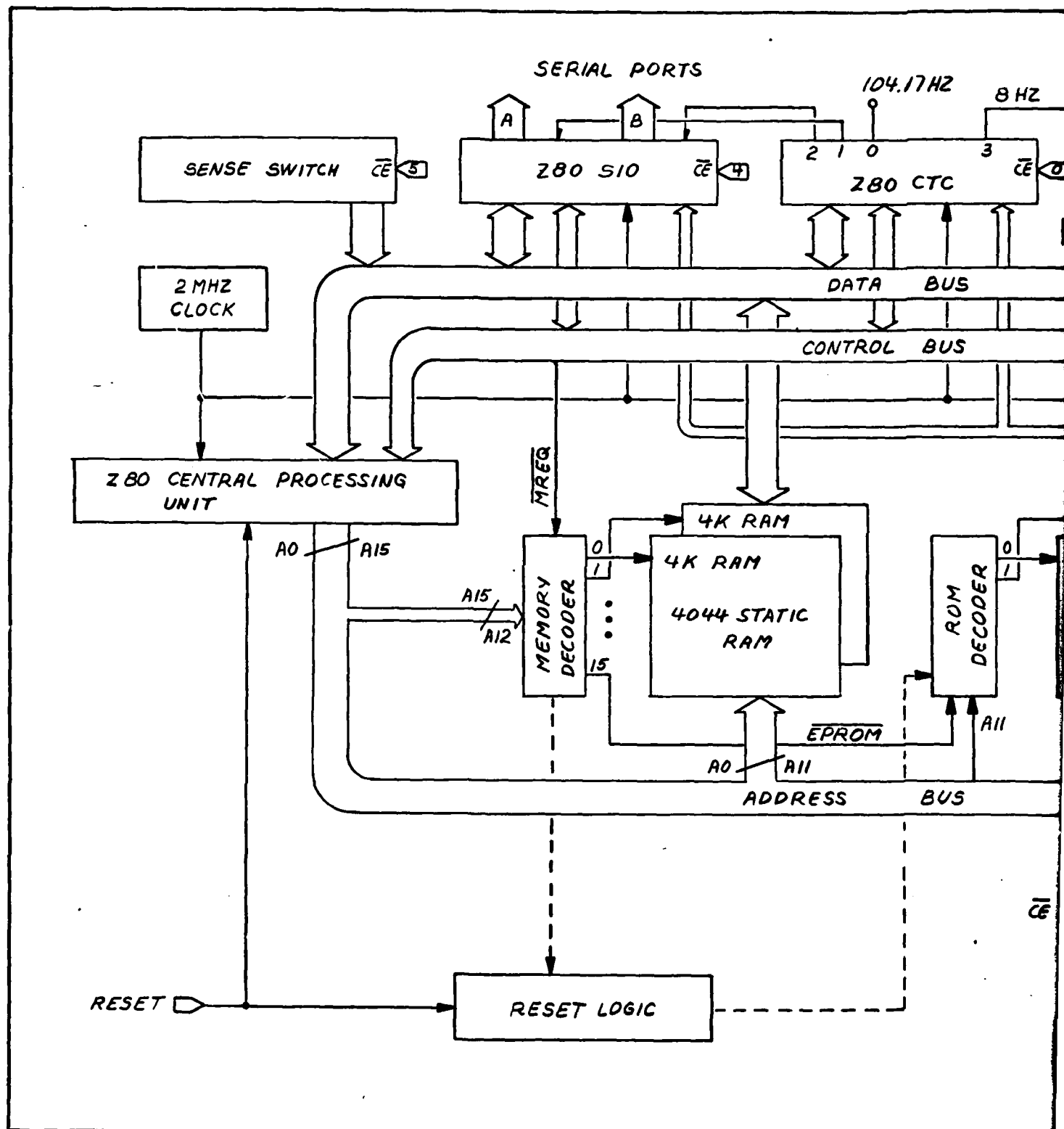
Fig. 4. Microcomputer Block Diagram
