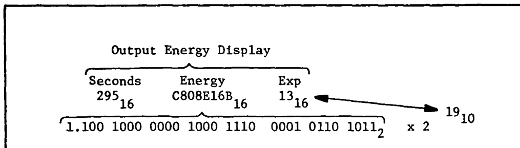
Fig. 31. Consumed Energy Expressed in Scientific Notation
