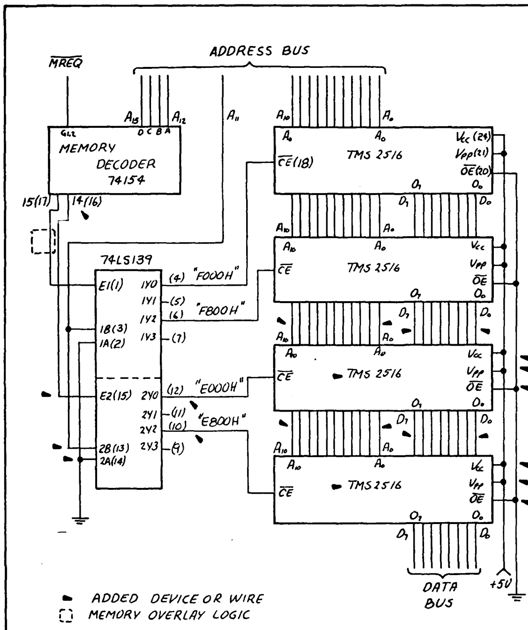
Fig. 20. EPROM Enlargement Schematic Diagram
