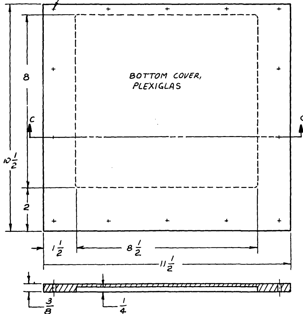
SECTION C-C
