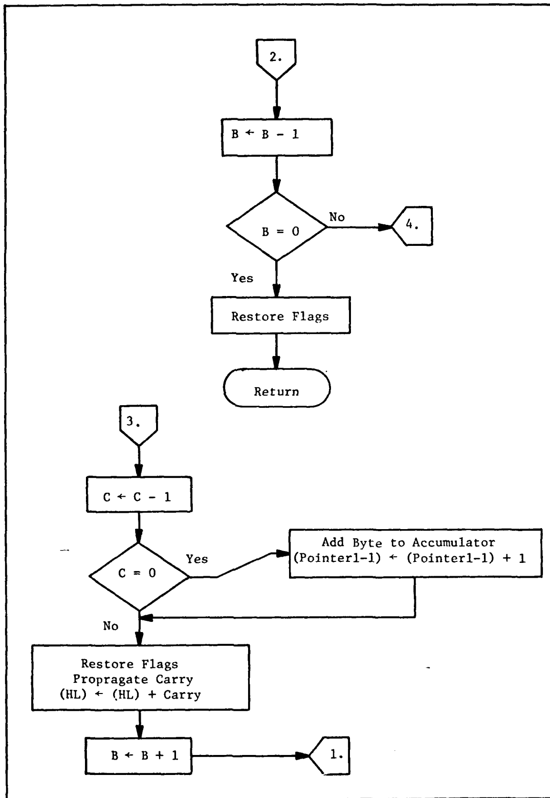
Fig. 38. Vector Summation (SUM) Flow Chart (Sheet 2 of 2)
