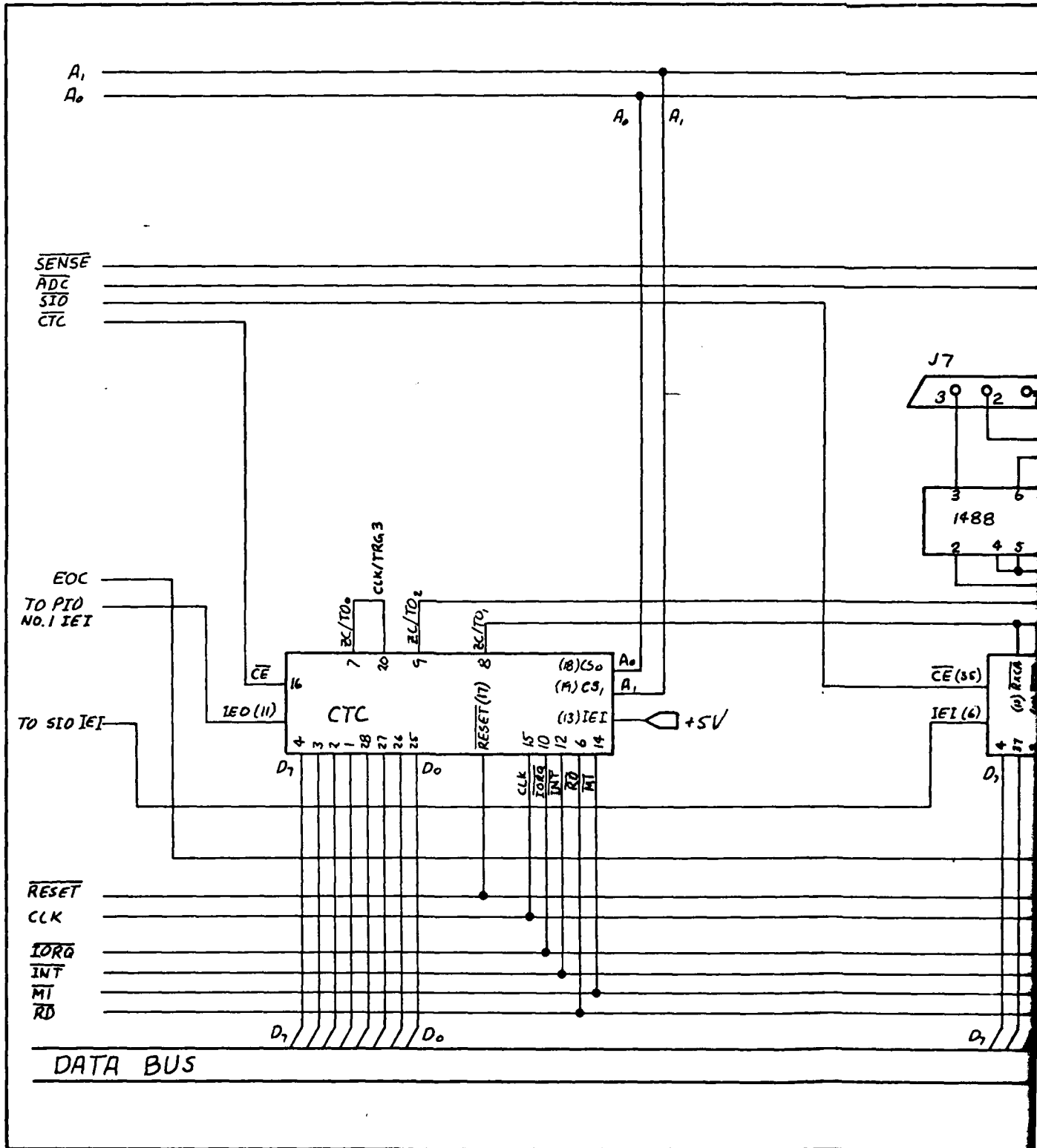
Fig. 16. Microcomputer Schematic Diagram, Serial I/O (Sheet 4 of 5)
