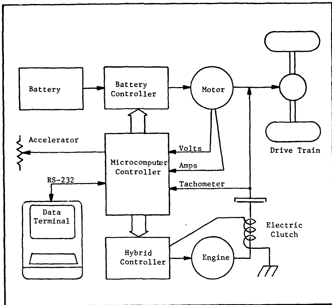
Fig. 3. Microcomputer Controller Parallel Hybrid Vehicle Block Diagram
