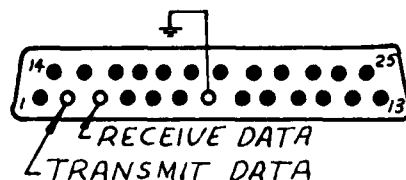
Fig. 22. Microcomputer Connector Pin-out Diagram
