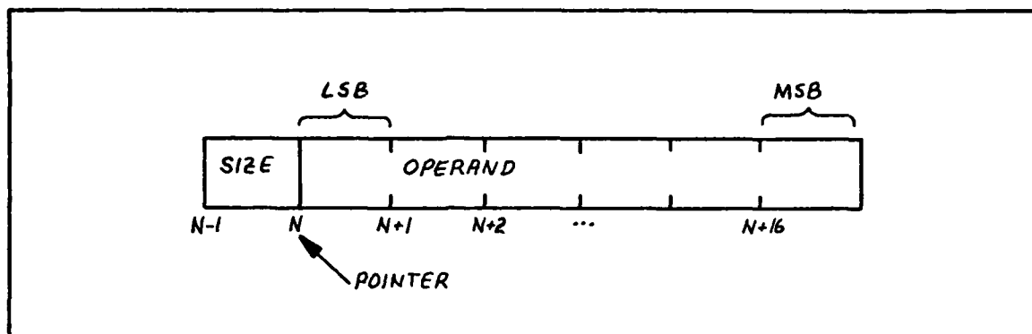
Fig. 34. Memory Vector
