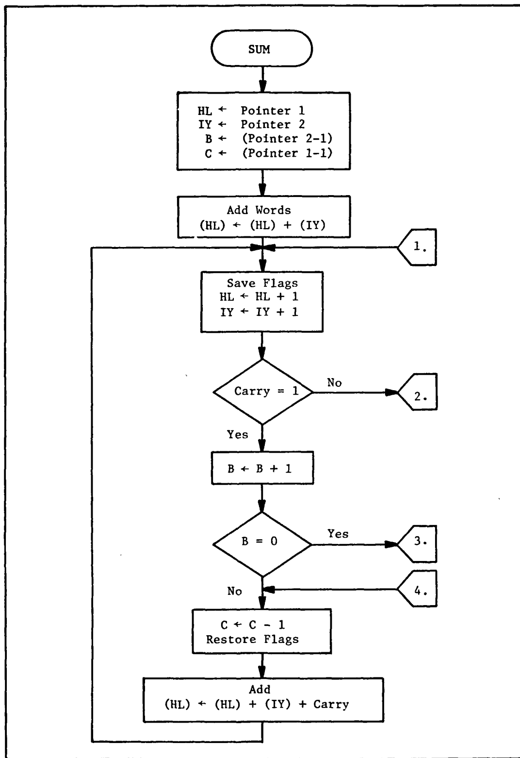
Fig. 38. Vector Summation (SUM) Flow Chart (Sheet 1 of 2)
