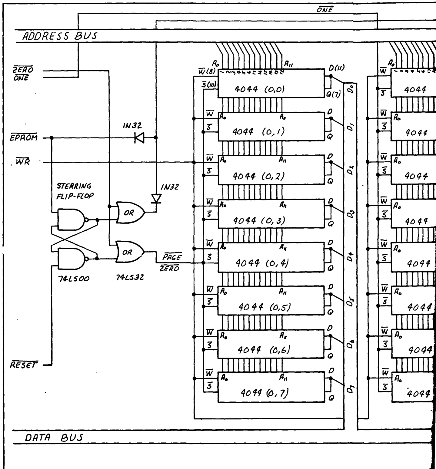
Fig. 16. Microcomputer Schematic Diagram, Memory (Sheet 2 of 5)
