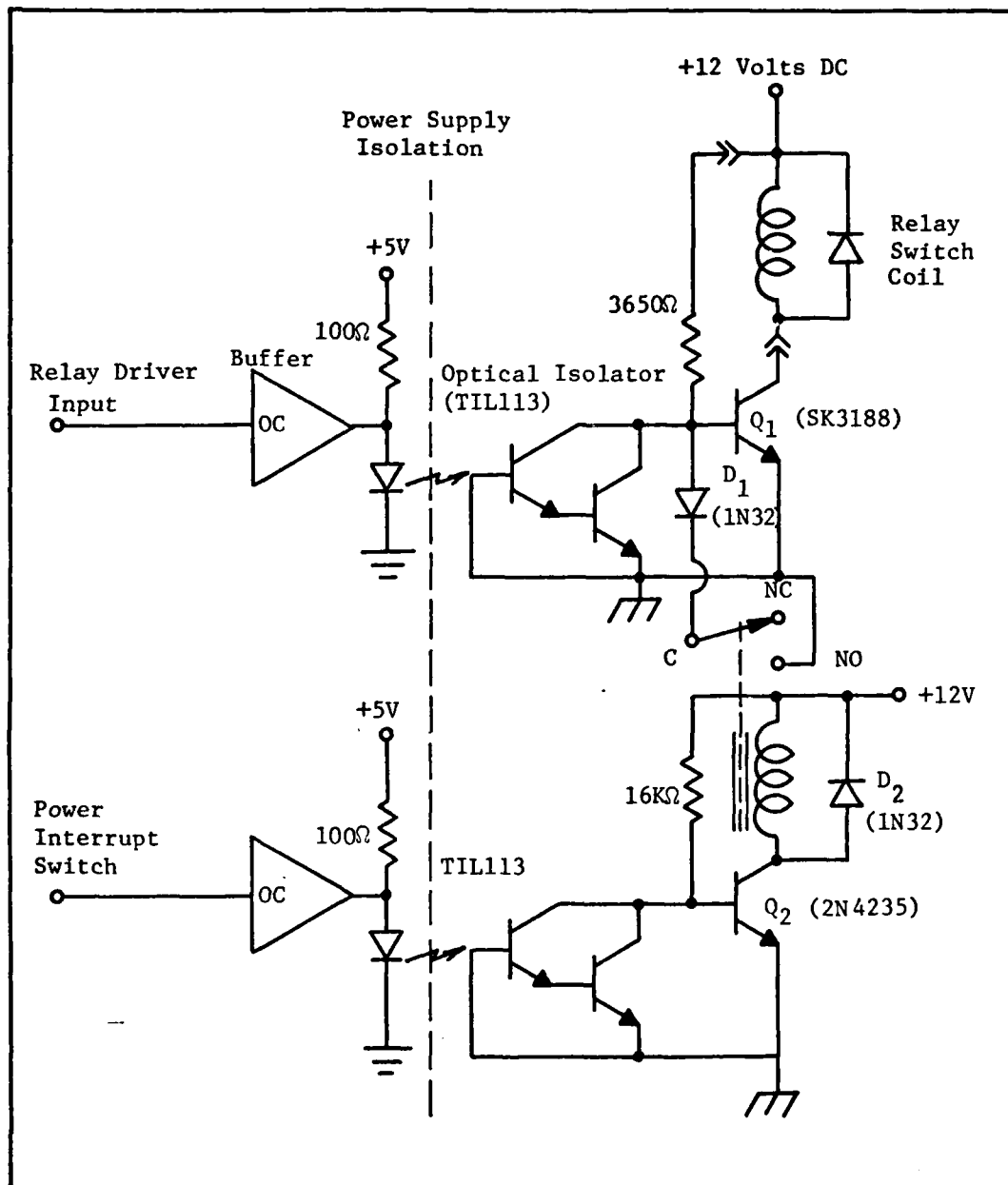
Fig. 5. Battery Controller Showing one Relay Driver and Power Interrupt Logic
