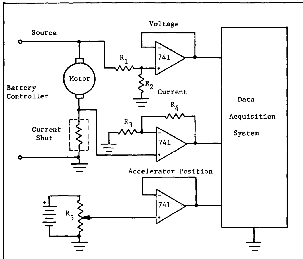
Fig. 7. Simplified Schematic Diagram of Analog Scaling Circuits
