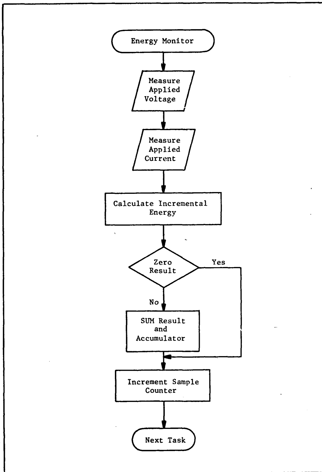
Fig. 11. Energy Monitor Flow Chart
