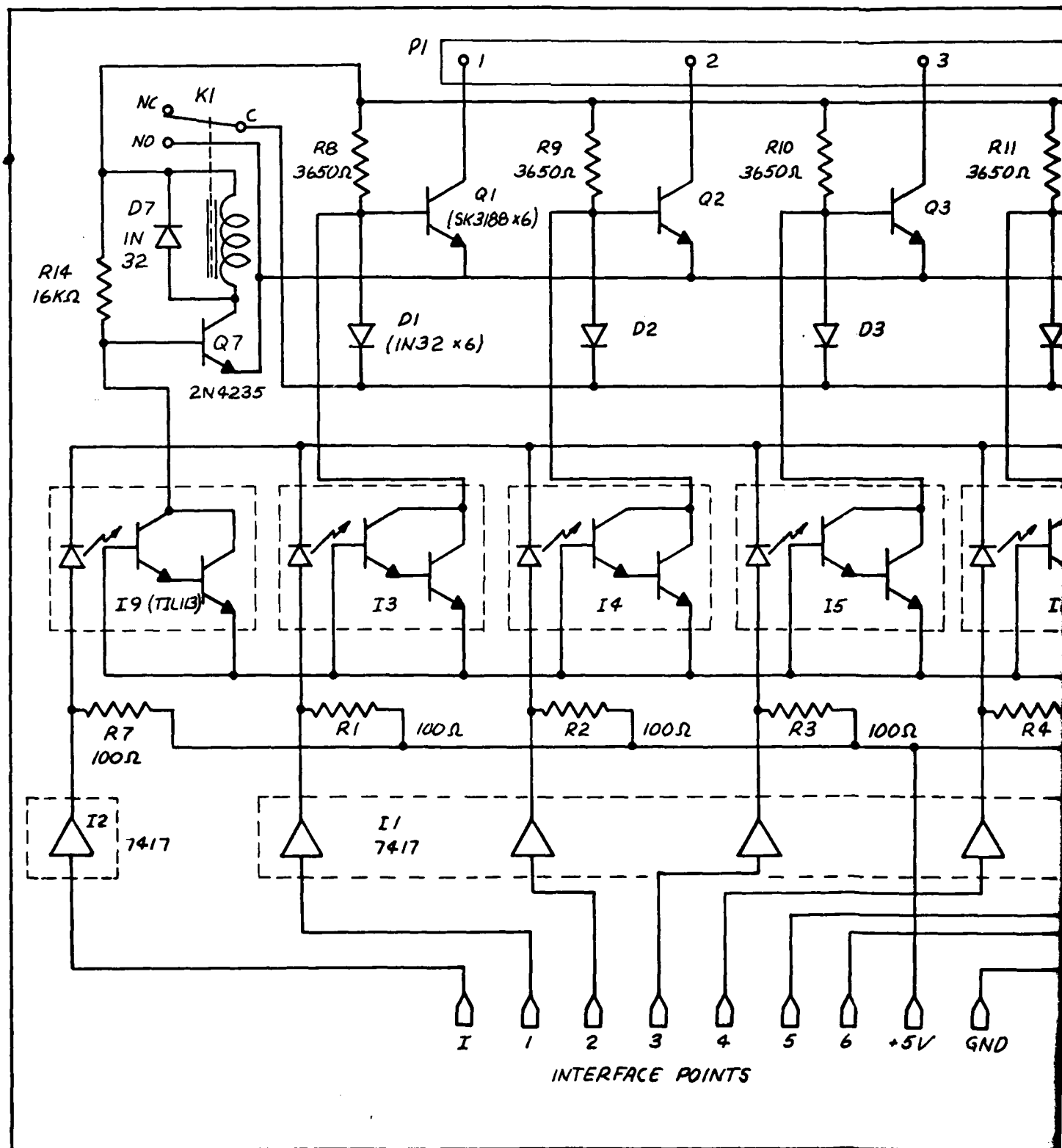
Fig. 27. Schematic Diagram of Digital Interface
