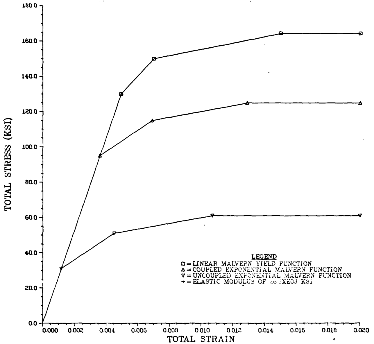
FIGURE 12. STRAIN HARDENING YIELD FUNCTIONS USED IN VARIOUS VERSIONS OF THE MALVERN OVERSTRESS FLOW LAW.
