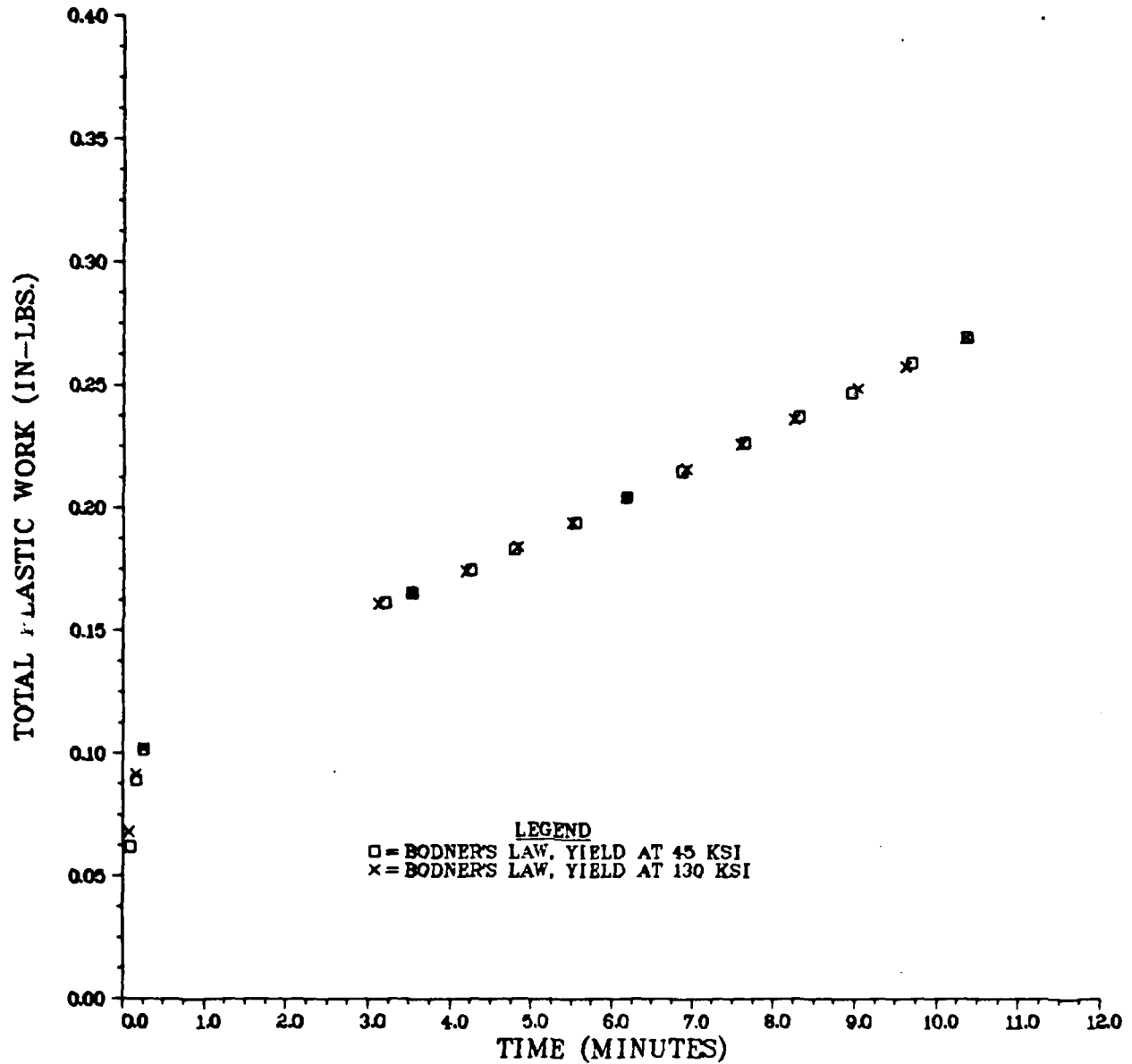
FIGURE 21. TOTAL PLASTIC WORK VERSUS FINITE ELEMENT NODE RELEASE TIMES FOR AN APPLIED LOAD OF 16060 LBS.
