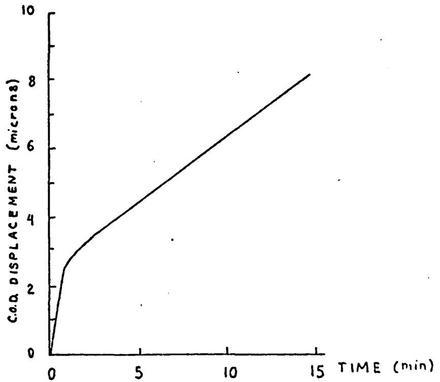
FIGURE 17. TEST 9 EXPERIMENTAL RESULTS (Sharpe, Ref. 8)
