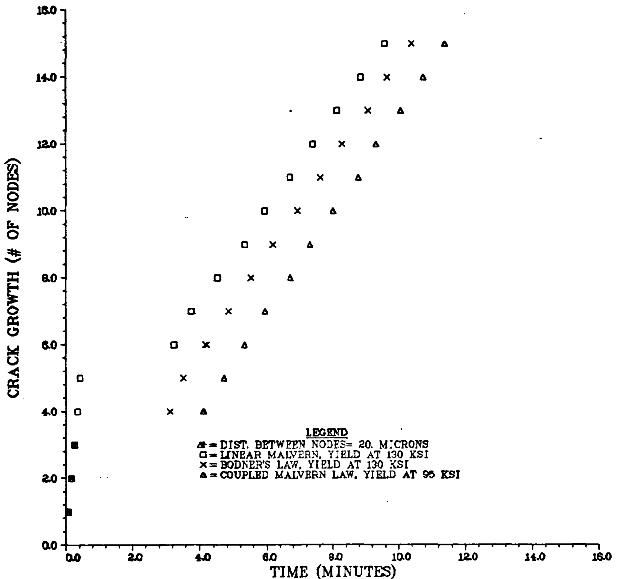
FIGURE 26. NUMBER OF NODES RELEASED VERSUS TIME FOR VARIOUS FLOW LAWS WITH AN APPLIED LOAD OF 16060 LBS.
