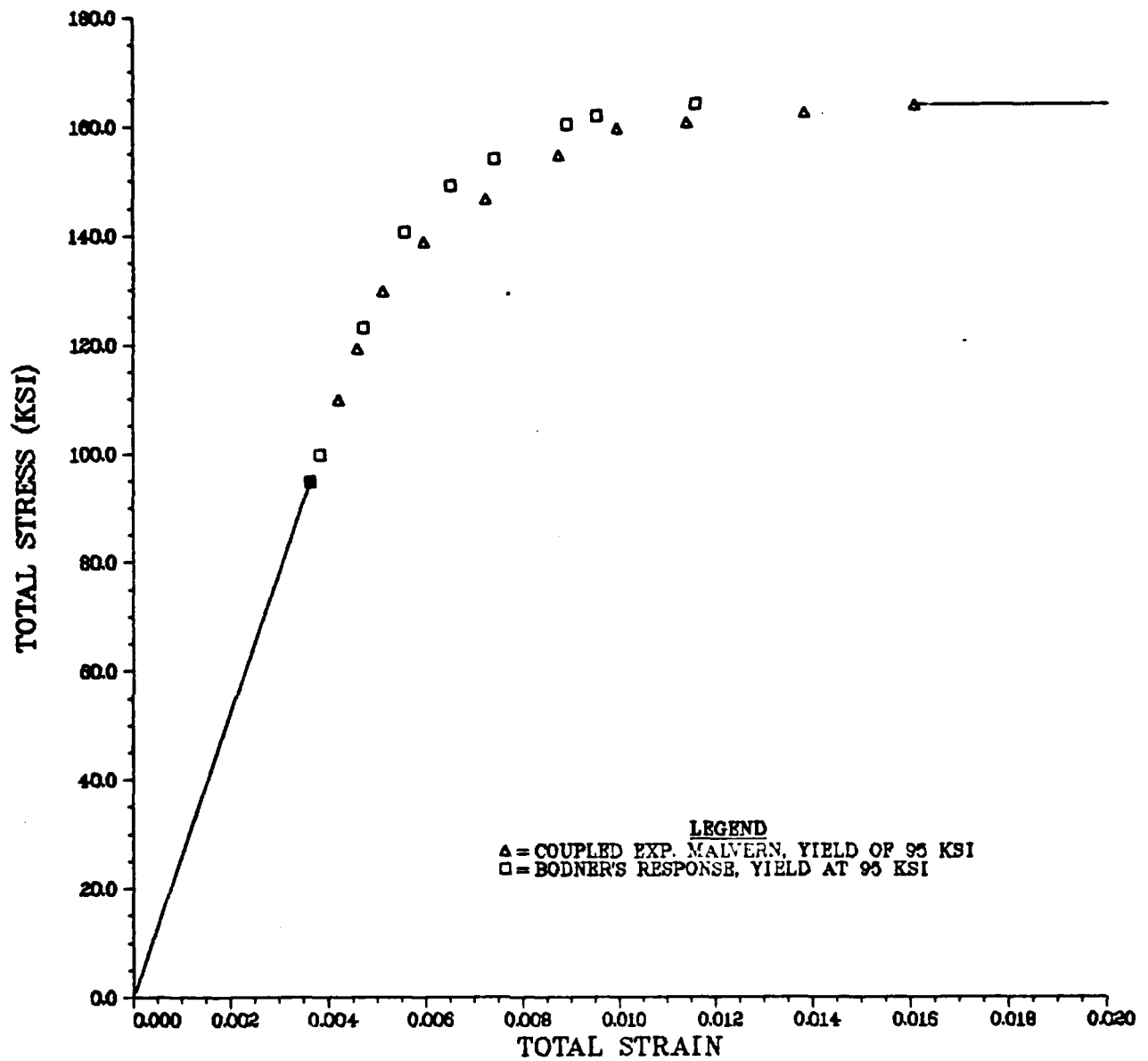
FIGURE 14. COUPLED EXPONENTIAL MALVERN VERSES BODNER'S FLOW LAW USING A UNIAXIAL FINITE ELEMENT RESPONSE OF IN100 AT 1350F.
