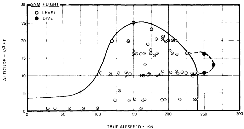
Figure 3. Altitude Envelope.
