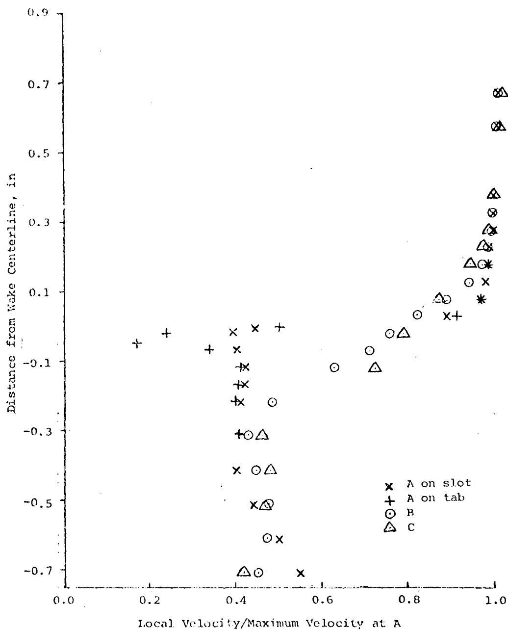
Fig. 22 Slotted Plate Velocity Profiles, U=0.40
