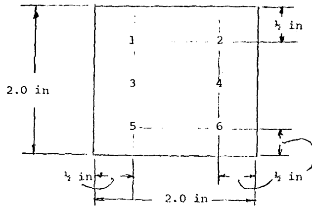
Rear View of Test Section:
