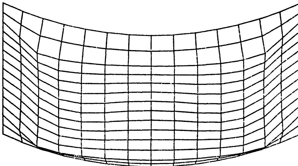
Figure 19. Pre-Buckled Displacement Geometry for (0.,45.,-45.,90.)_S Laminate
