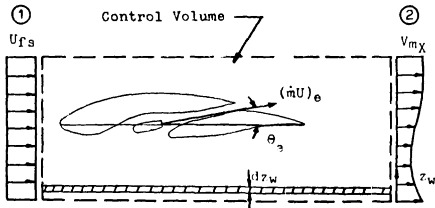
Figure 55 Wake Survey
