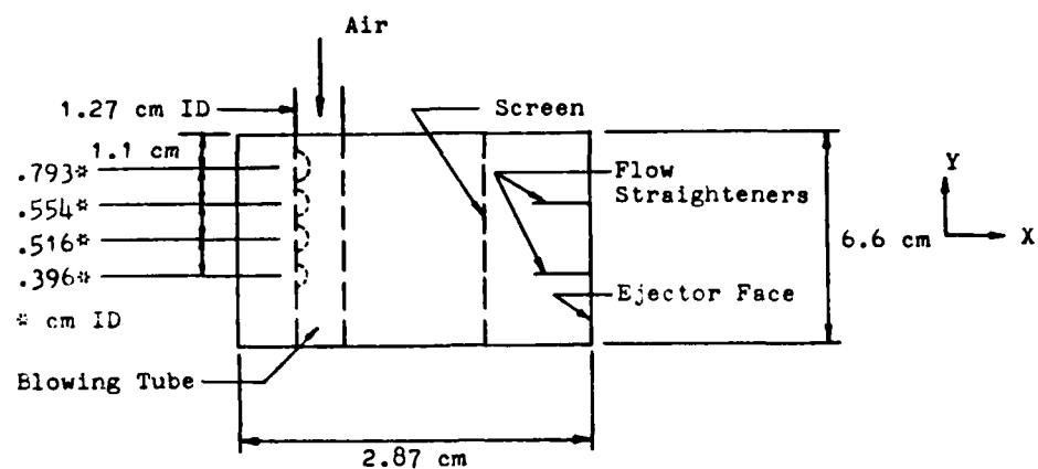
Top View
