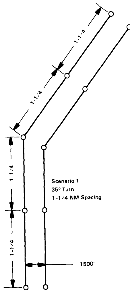
Figure 4. Fundamental Channel Design Also Employed as Low Density Buoyed Turn
