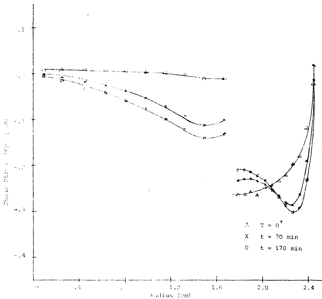
Fig 4.6-P. Shear Stress, Disc.
