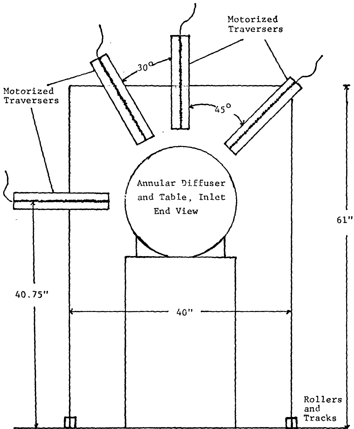
Figure 18. Traversing Mechanism
