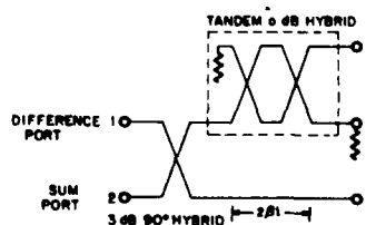
FIGURE 2: SCHEMATIC OF A 180^\circ HYBRID.
