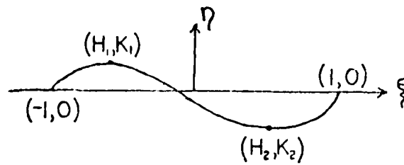
Figure 9. Piecewise Parabolic Upwind Function U_j
