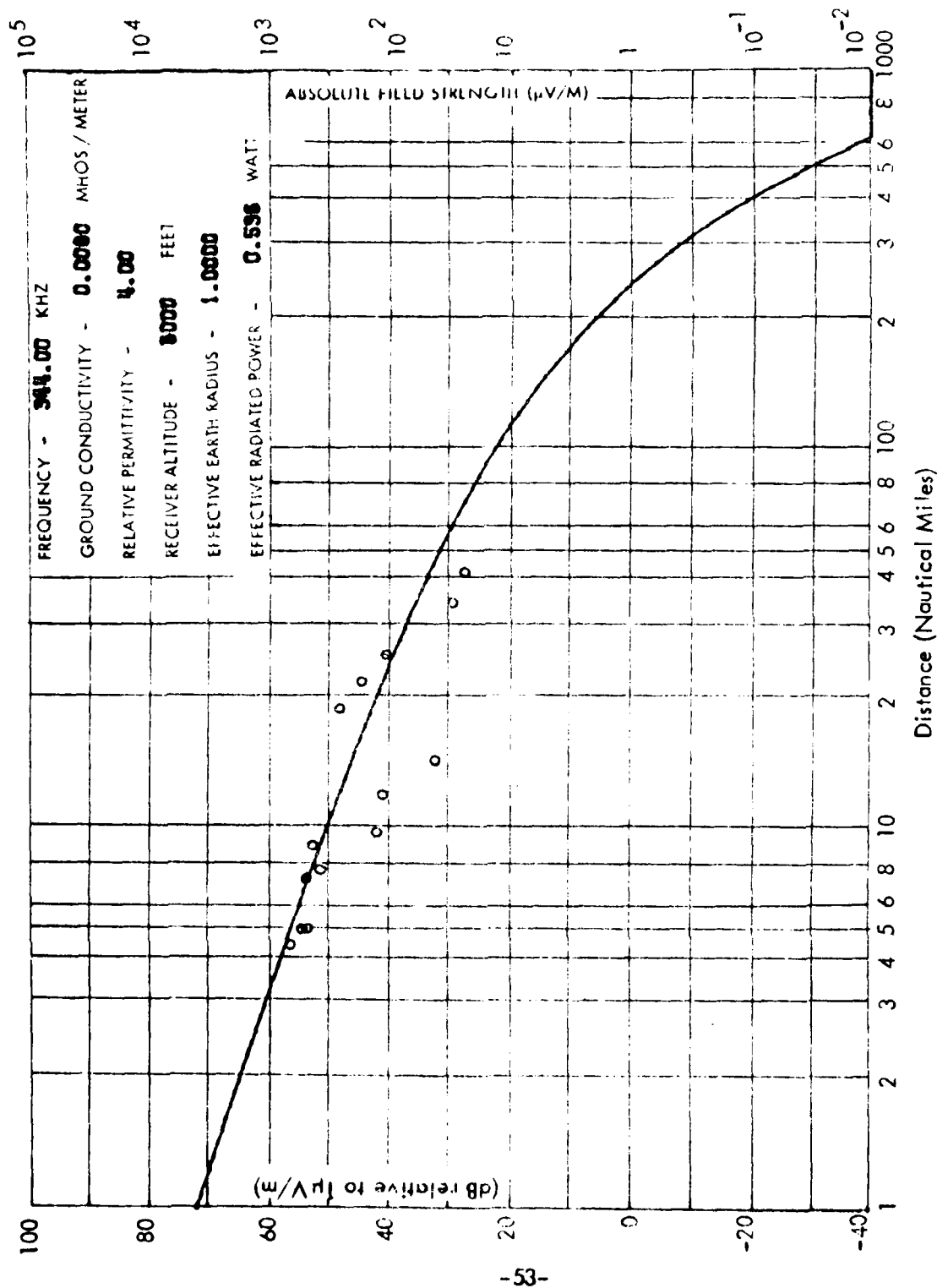
Figure 2-28. Flight Data on Picture Rocks, Pennsylvania Beacon; 6/19/79; DC-3. Coordinates: 41^{\circ}16'38''N , 76^{\circ}42'24''W ; Call Sign: PIX; Transmitter Power: 25 watts.
