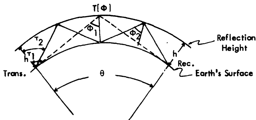
Figure 4-1. Sky Wave Propagation Model.
