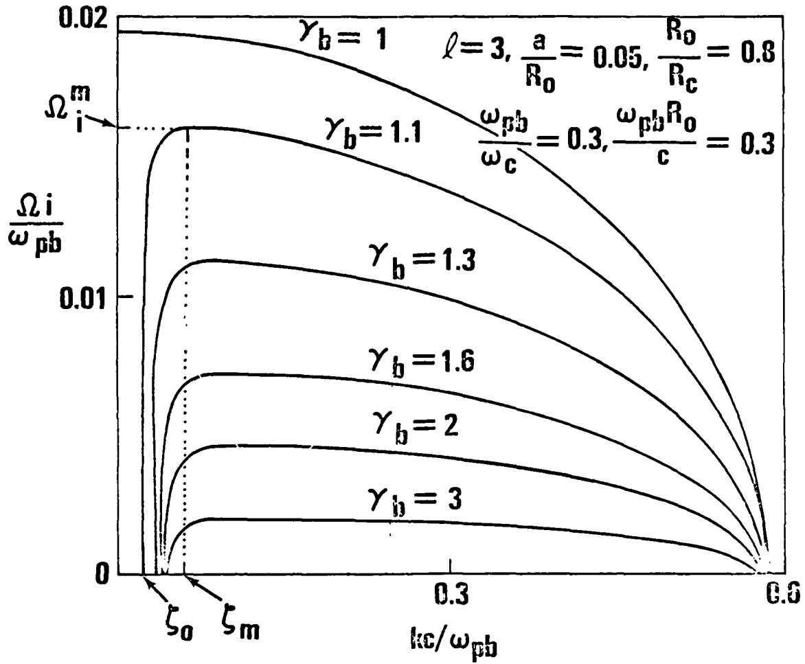
Fig. 6 Dependence of the growth rate and the long wavelength cutoff of the positive k spectrum of the instability on the beam energy \gamma_b , for the case of \ell = 3, a/R_0 = 0.05, R_0/R_c = 0.8, \omega_{pb}/\omega_c = 0.3, \omega_{pb}R_0/c = 0.3 . (Note that the latter two parameters are different from those in Figs. 3 - 5)
