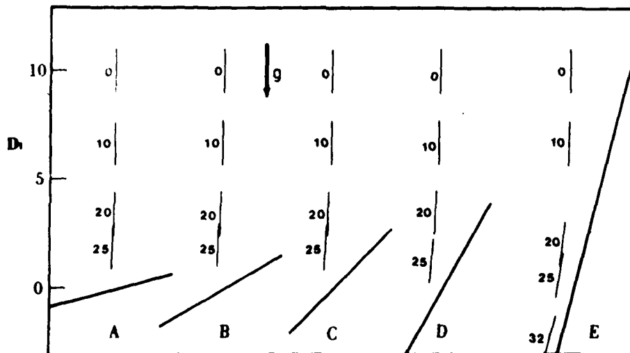
Fig. 12. Time history of a cylinder falling towards a plane inclined to the horizontal at angles: A-15°, B-30°, C-45°, D-60°, E-75°; initial orientation - vertical; D_{1,0} = 10 . Numbers near positions indicate elapsed time in seconds. Same cylinders' and medium's properties as of Fig. 5.
