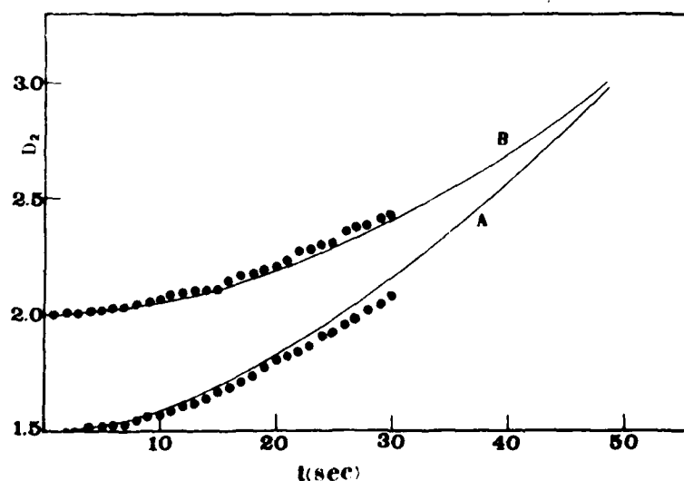
Fig. 6. Drift displacement and orientation of a cylinder near a vertical wall as a function of time. Same parameters as of Fig. 5 except for: A. D_{2,0} = 1.5 l; \theta_0 = 89^\circ . B: \theta_0 = 21 , \theta_0 = 93^\circ .
