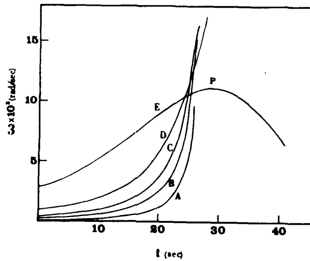
Fig. 18. Angular velocity of a cylinder falling towards an inclined plane. Same parameters and conditions as of Fig. 12. ( D_1 reaches a minimum at the point P).
