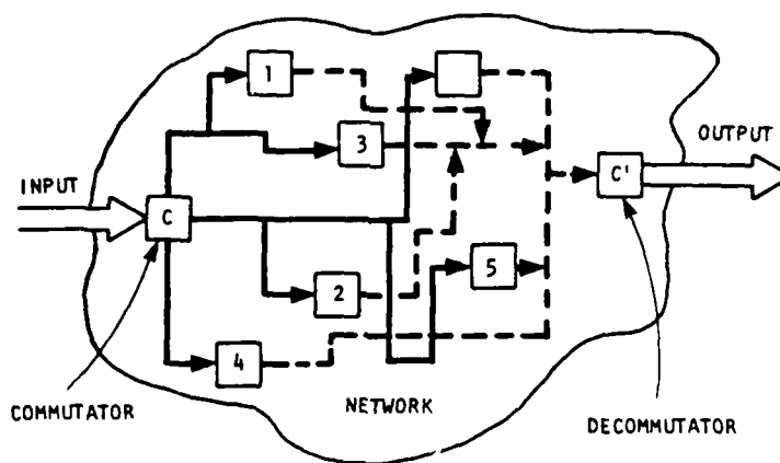
FIGURE 7 DIAGRAM OF PIPELINE PROCESSING IN A CHAMP NETWORK
