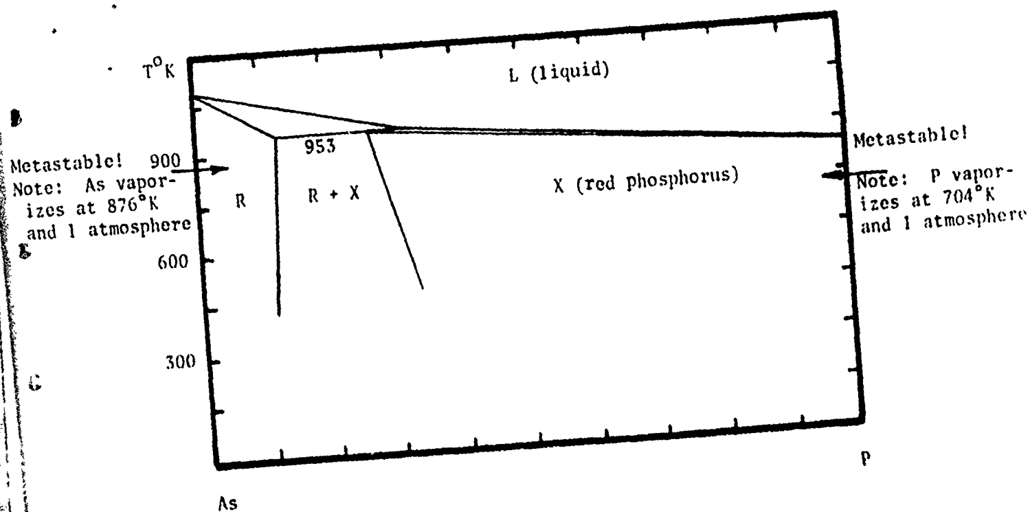
Figure 5. Calculated As-P Phase Diagram
