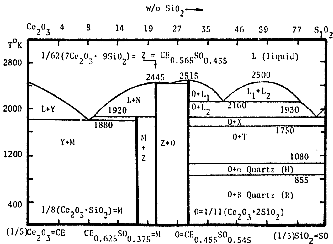
Figure 12. Calculated 1/5 Ce 2 O 3 - 1/3 SiO 2 Phase Diagram
