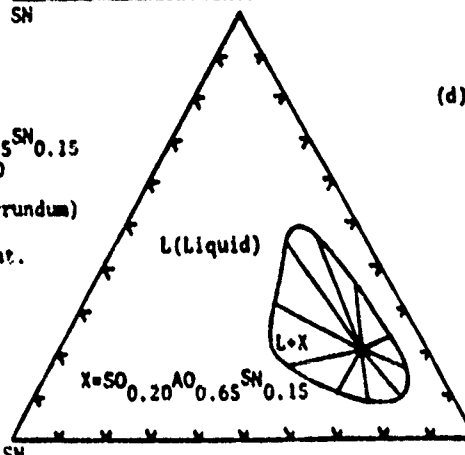
Figure 13 Calculated Pairwise (a-c) and Composite Equilibrium (d) in the (1/3)(SiO 2 ) - (1/7)(Si 3 N 4 ) - (1/5)Al 2 O 3 System at 2000K and one atmosphere
