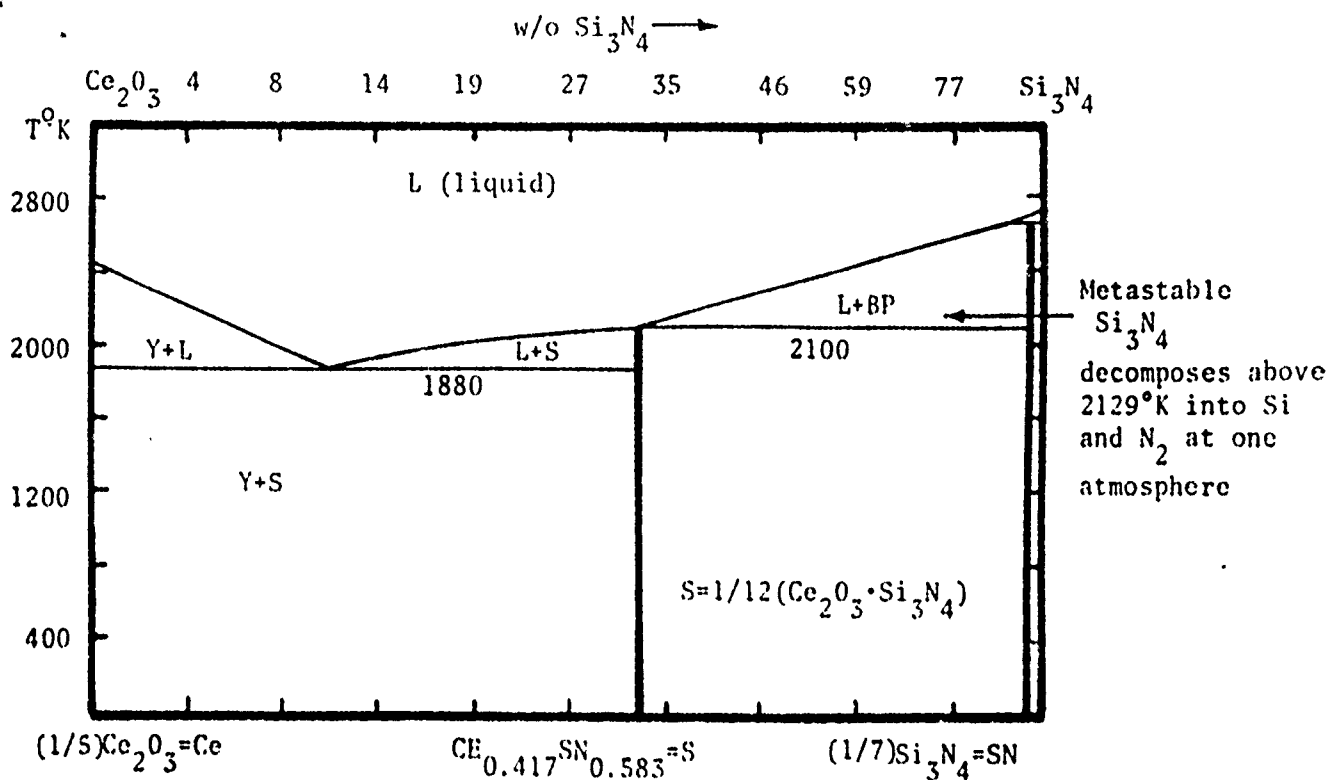
Figure 11. Calculated 1/5 Ce 2 O 3 - 1/7 Si 3 N 4 Phase Diagram
