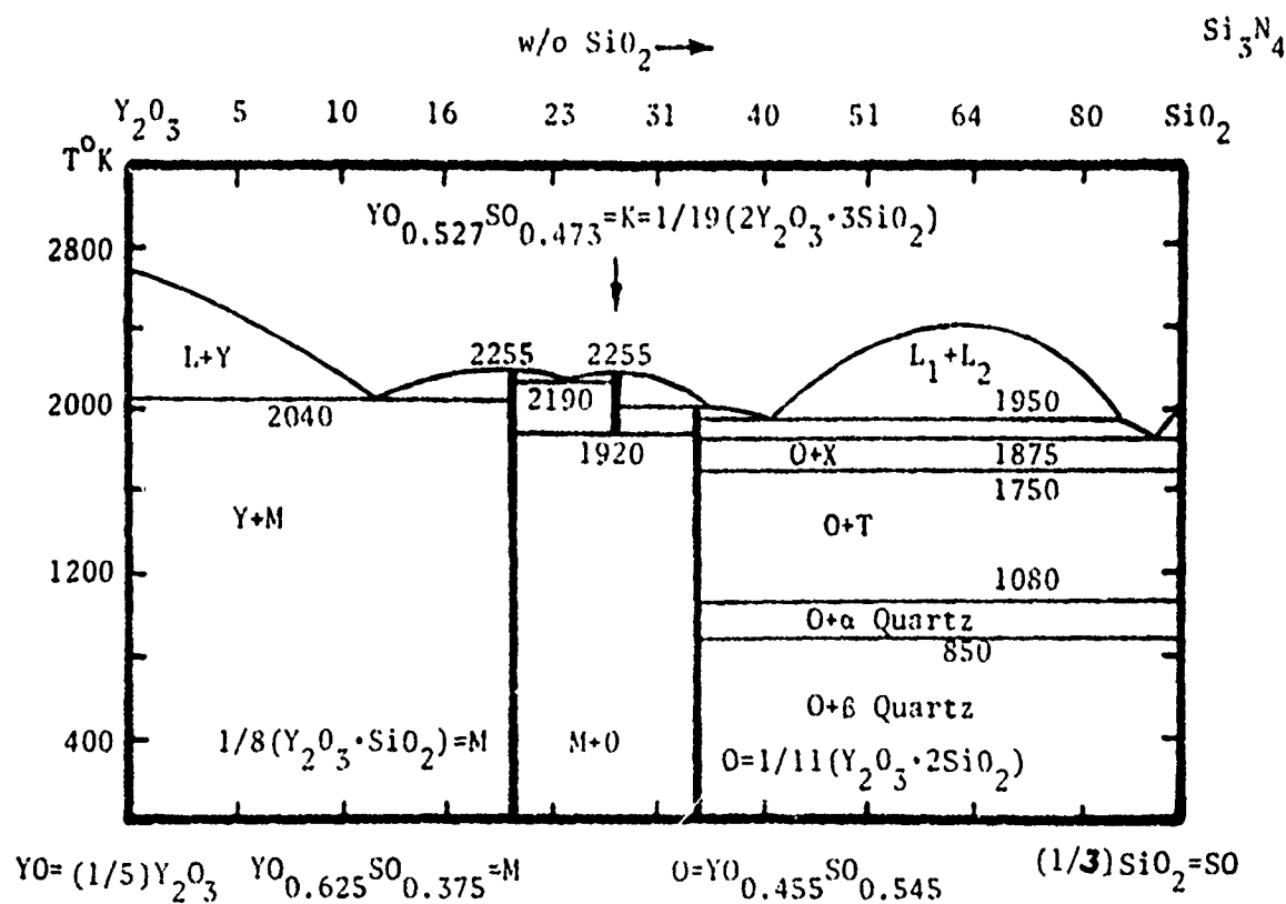
Figure 10. Calculated 1/5\text{Y}_2\text{O}_3 - 1/3\text{SiO}_2 Phase Diagram
