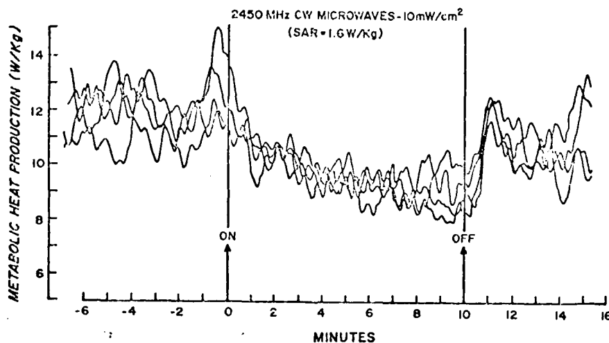
Figure 24. Stripchart tracings showing changes in metabolic heat production during 4 10-minute exposures to 10 mW/cm². Response latency to microwave onset is 60-90 seconds; that to microwave termination is 45 seconds.
